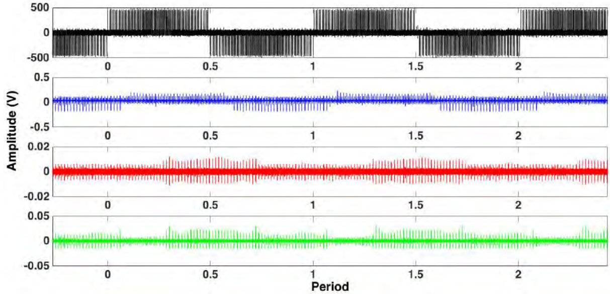
Figure IV.5: Phase to phase voltage VW(black), sensor signal filtered at 200 MHz phase V (blue), sensor signal filtered at 400 MHz phase W (red), sensor signal filtered at 400 MHz phase U (green)
