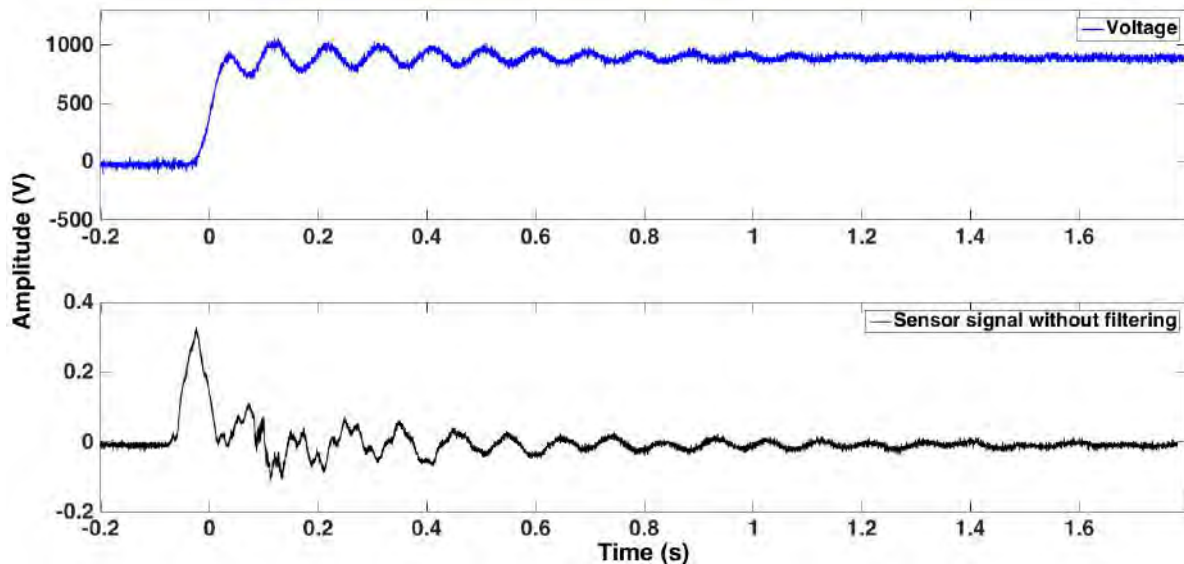
Figure III.1: Noisy signal induced by switching (black)
