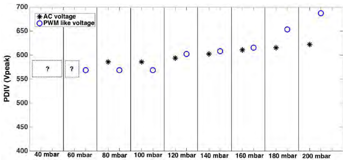
Figure II.27: Search for signal disappearance (PDIV)
