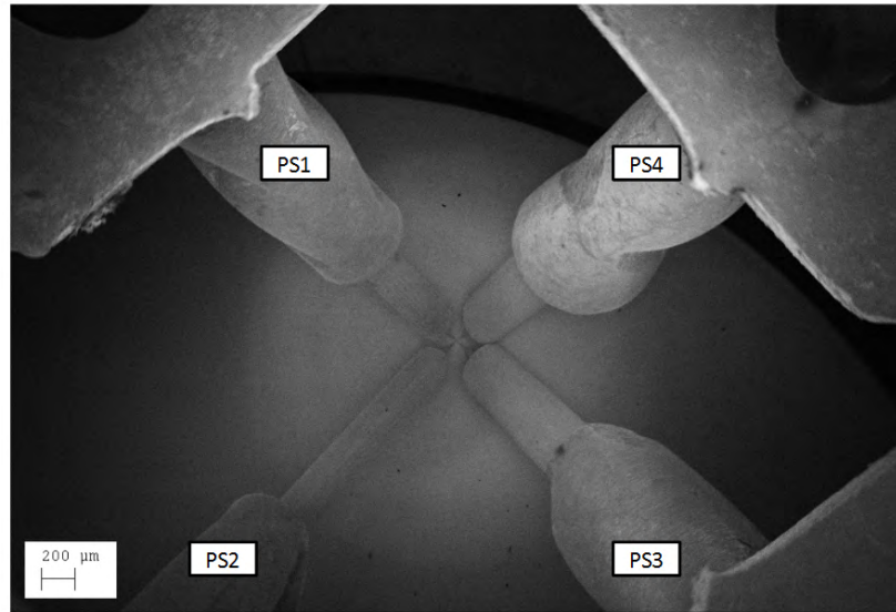
FIGURE 3.7 – Image SEM de quatre pointes 45° STM.
