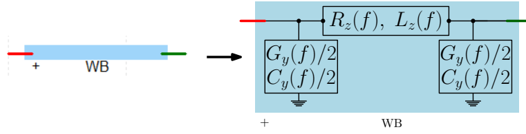
Figure H.3 – EMTPT Wideband cable interpretation
