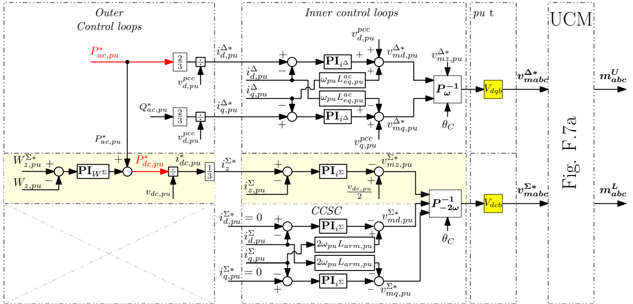
Figure F.12 – Energy-based controller # 1 from Section 3.3 [163]
