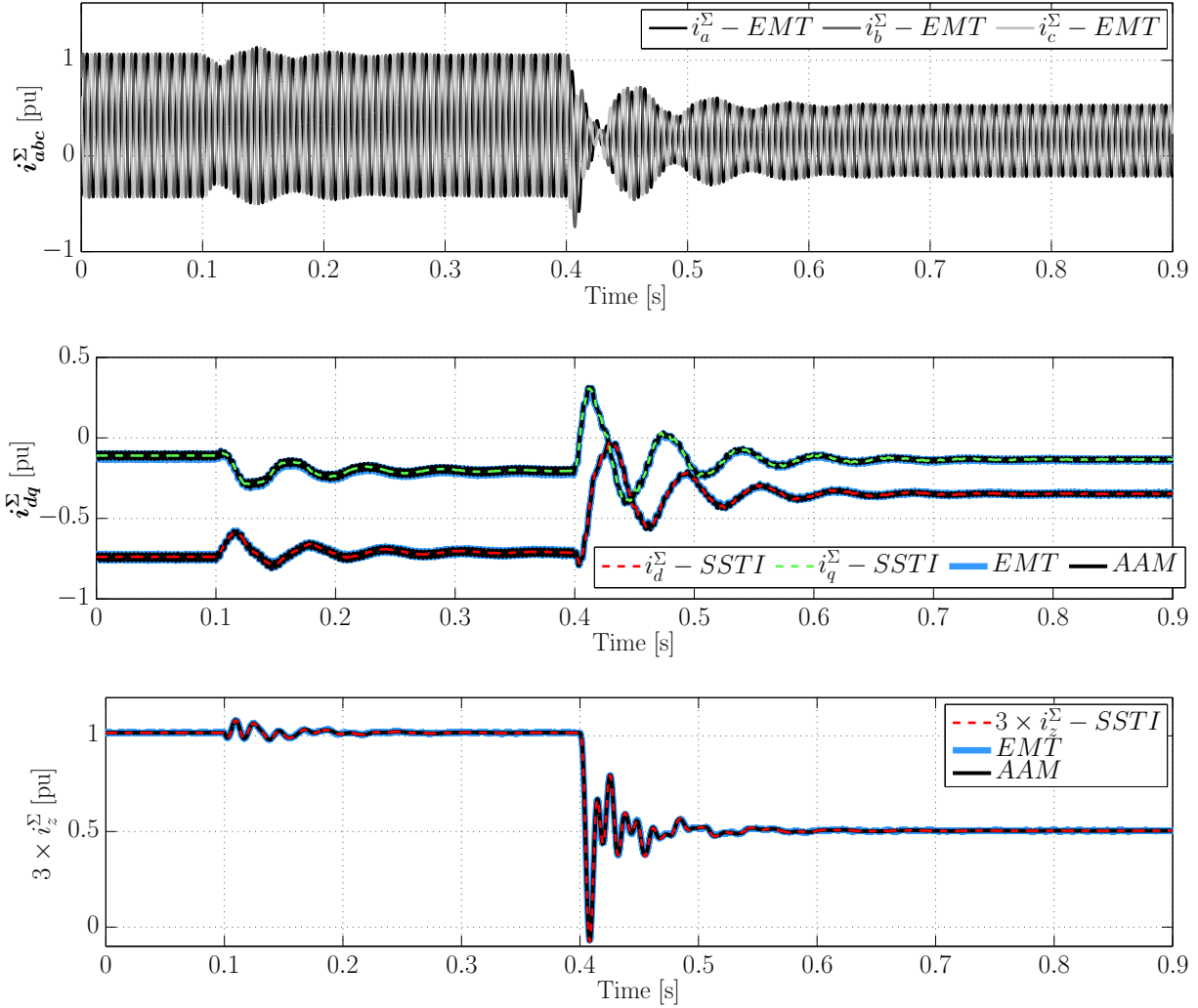
Figure 2.17 – Comparison of the derived SSTI model with the AAM and EMT models: common-mode currents i_{dqz}^\Sigma i) dq components and ii) zero-sequence
