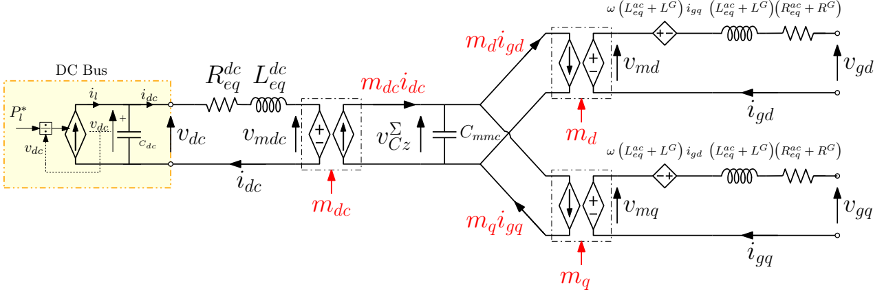
Figure 4.6 – Circuit diagram of SSTI-MMC simplified model from [123]
