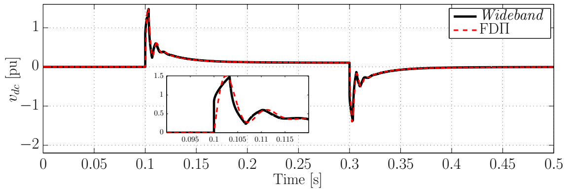
(b) DC Voltage v_{dc}
