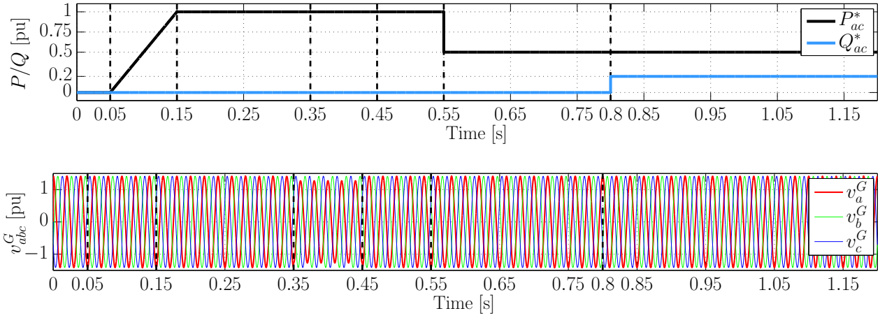
Figure F.6 – Scenario for the evaluation of different MMC High level controllers
