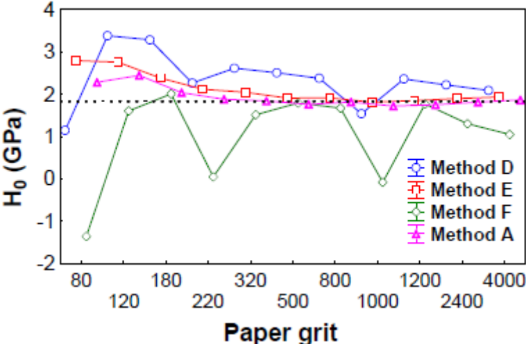
Figure 15: Macro-hardness estimation for each abraded specimen calculated with the method A, D, E or F.
