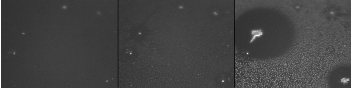
Figure 2.5 – Image recorded by the zoom camera for experiment A–Imm–1 at a cooling rate of 0.5 \text{ K}\cdot\text{min}^{-1} (see Chapter 3 for experiment description) respectively 20s before (left), 20s after (center) and 5min 40s (right) after condensation started on the wafer.
