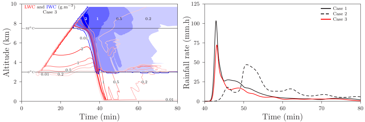
Figure 5.4 – (a, left) Liquid water content ( \text{g.m}^{-3} , red) and ice water content ( \text{g.m}^{-3} , blue) simulated by DESCAM as a function of altitude and time for the case with only homogeneous nucleation active (case 3). (b, right) Time evolution of the rainfall rate ( \text{mm.h}^{-1} ) for the only-liquid case (case 1, black continuous), the all ice processes, all minerals case (case 2, black dashed) and the homogeneous only case (case 3, red continuous).
