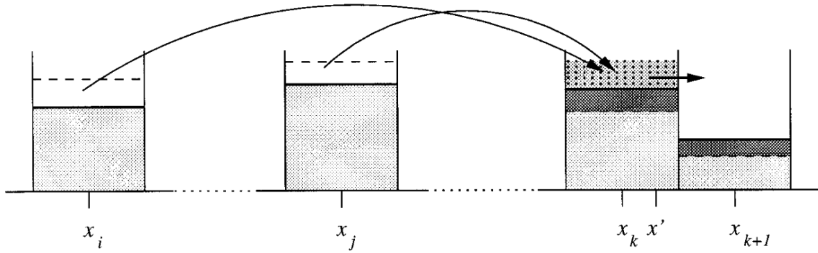
\mathcal{N}_{\text{ation}}\text{setupfont}=\text{footnotesize } \mathcal{N}_{\text{ation}} Schematic illustration of the flux method of redistribution of droplets of mass m_f(x') into bins \mathbf{k}\mathbf{k} and \mathbf{k}\mathbf{k}+1 (from Bott, 1998)
