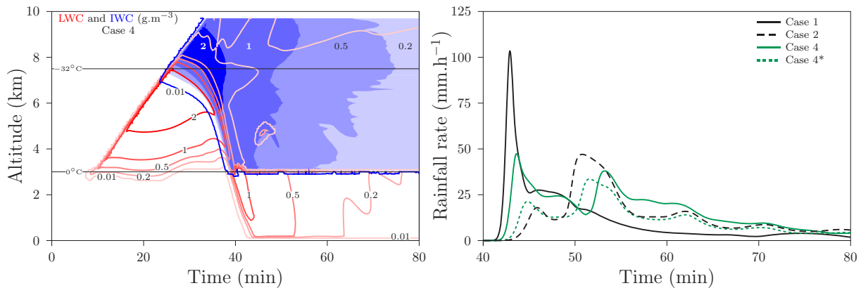
Figure 5.6 – (a, left) Liquid water content ( \text{g.m}^{-3} , red) and ice water content ( \text{g.m}^{-3} , blue) simulated by DESCAM as a function of altitude and time for the case with only immersion freezing active (case 4). (b, right) Time evolution of the rainfall rate ( \text{mm.h}^{-1} ) for the only-liquid case (case 1, black continuous), the all ice processes case (case 2, black dashed) and for immersion freezing with B = 2.9 \cdot 10^{-6} \text{cm}^{-3} \cdot \text{s}^{-1} (case 4, green continuous) and with original Bigg values (case 4*, green dashed).
