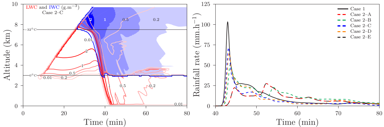
Figure 6.7 – (a, left) Liquid water content ( \text{g}\cdot\text{m}^{-3} , red) and ice water content ( \text{g}\cdot\text{m}^{-3} , blue) simulated by DESCAM as a function of altitude and time for the case with only kaolinite active as INP and all ice nucleation mechanisms active (case 2-C). (b, right) Time evolution of the rainfall rate ( \text{mm}\cdot\text{h}^{-1} ) for the only-liquid case (case 1, black continuous) and the all ice nucleation mechanisms cases for K-feldspar (case 2-A, red dashed), illite (case 2-B, green dashed), kaolinite (case 2-C, blue dashed), quartz (case 2-D, orange dashed) and all minerals (case 2-E, black long dashed).
