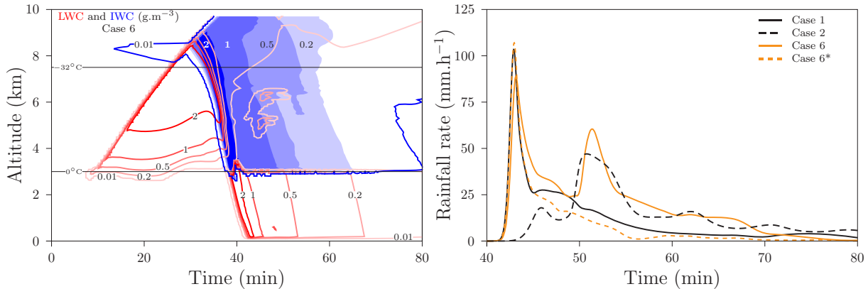
Figure 5.9 – (a, left) Liquid water content ( \text{g.m}^{-3} , red) and ice water content ( \text{g.m}^{-3} , blue) simulated by DESCAM as a function of altitude and time for the case with only deposition nucleation active (case 6). (b, right) Time evolution of the rainfall rate ( \text{mm.h}^{-1} ) for the only-liquid case (case 1, black continuous), the all ice processes case (case 2, black dashed) and for deposition nucleation with r_{\text{IN}} \geq 0.1 \mu\text{m} (case 5, orange continuous) and with r_{\text{IN}} \geq 0.5 \mu\text{m} (case 5*, orange dashed).
