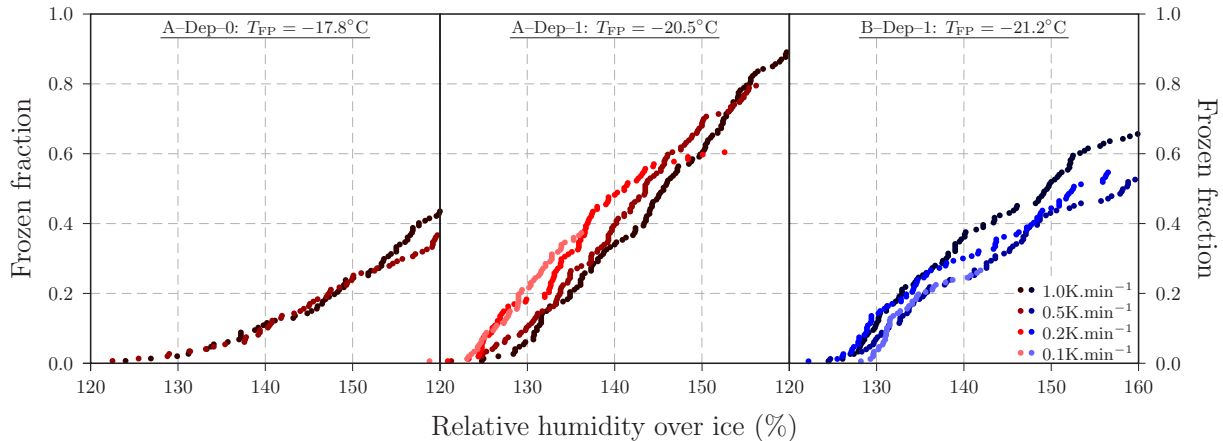
Figure 4.4 – Frozen fraction as a function of relative humidity at different cooling rates ( 1 \text{ K}\cdot\text{min}^{-1} in brown, 0.5 \text{ K}\cdot\text{min}^{-1} in dark red and blue, 0.2 \text{ K}\cdot\text{min}^{-1} in red and blue and 0.1 \text{ K}\cdot\text{min}^{-1} in pink and light blue) for experiments A –Dep–0 (a, left), A –Dep–1 (b, center) and B –Dep–1 (c, right).
