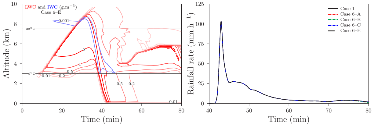
Figure 6.6 – (a, left) Liquid water content ( \text{g.m}^{-3} , red) and ice water content ( \text{g.m}^{-3} , blue) simulated by DESCAM as a function of altitude and time for the case with only deposition nucleation active with all minerals as INP (case 6-E). (b, right) Time evolution of the rainfall rate ( \text{mm.h}^{-1} ) for the only-liquid case (case 1, continuous) and the deposition only cases for K-feldspar (case 6-A, red double dotted-dashed), illite (case 6-B, green double dotted-dashed), kaolinite (case 6-C, blue double dotted-dashed) and all minerals (case 6-E, black long dashed) on top of each other.
