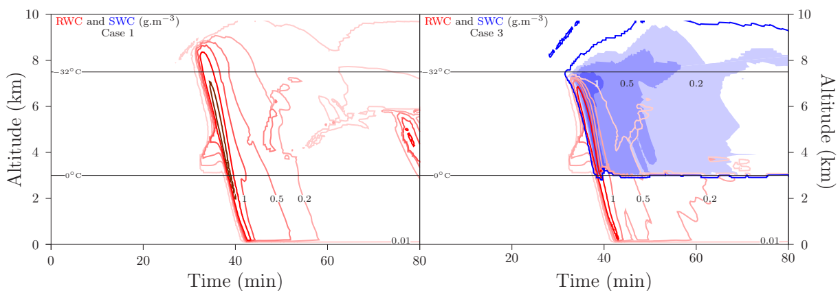
Figure 5.5 – Precipitating liquid water content ( \text{g.m}^{-3} , red) and precipitating ice water content ( \text{g.m}^{-3} , blue) simulated by DESCAM as a function of altitude and time for the case with no ice nucleation mechanisms (a, left — case 1) and for the case with only homogeneous nucleation active (b, right — case 3).
