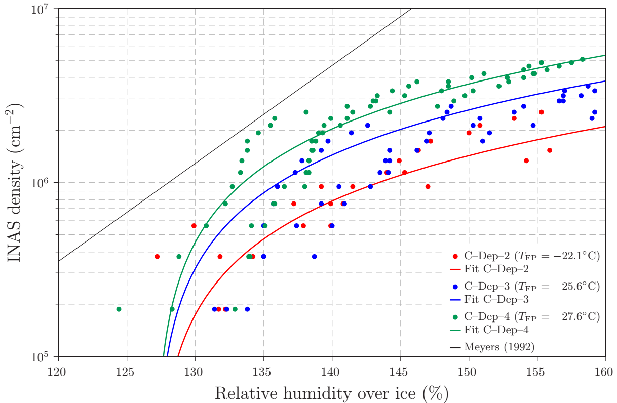
Figure 4.7 – Ice nucleating active site (INAS) density as a function of the relative humidity for the three deposition experiments using suspension C : C-Dep-2 in red, C-Dep-3 in blue and C-Dep-4 in green. In colored solid lines are represented the fit curves for each of these experiments with the fit function defined as: n_{s,\text{dep}}(T, RH_i) = \exp(10.5 - 0.18 \cdot T) \cdot [1 - \exp(0.02 \cdot (127 - RH_i))] . The black solid line corresponds the Meyers parameterization with the assumption of an aerosol surface concentration of S_{\text{aer}} = 2 \cdot 10^{-2} \text{cm} \cdot \text{m}^{-3} .
