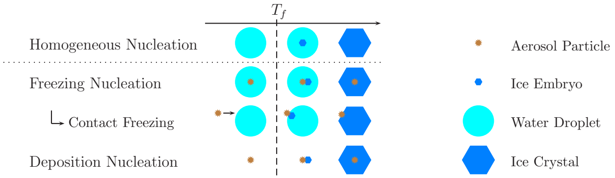
Figure 1.3 – Schematic diagram of ice nucleation mechanisms as depicted by Vali et al. (2015). Freezing nucleation contains immersion, condensation and contact freezing with only the latter depicted here.
