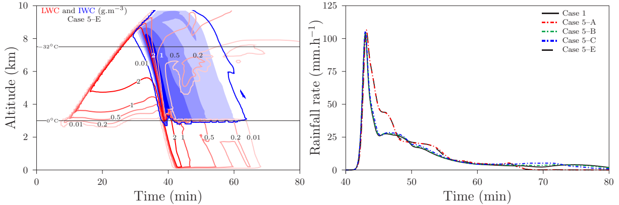
Figure 6.5 – (a, left) Liquid water content ( \text{g.m}^{-3} , red) and ice water content ( \text{g.m}^{-3} , blue) simulated by DESCAM as a function of altitude and time for the case with only contact freezing active with all minerals as INP (case 5-E). (b, right) Time evolution of the rainfall rate ( \text{mm.h}^{-1} ) for the only-liquid case (case 1, continuous), the contact freezing only cases with r_{\text{IN},\text{lim}} = 0.1\mu\text{m} for K-feldspar (case 5-A, red dotted-dashed), illite (case 5-B, green dotted-dashed), kaolinite (case 5-C, blue dotted-dashed) and all minerals (case 5-E, black long dashed).
