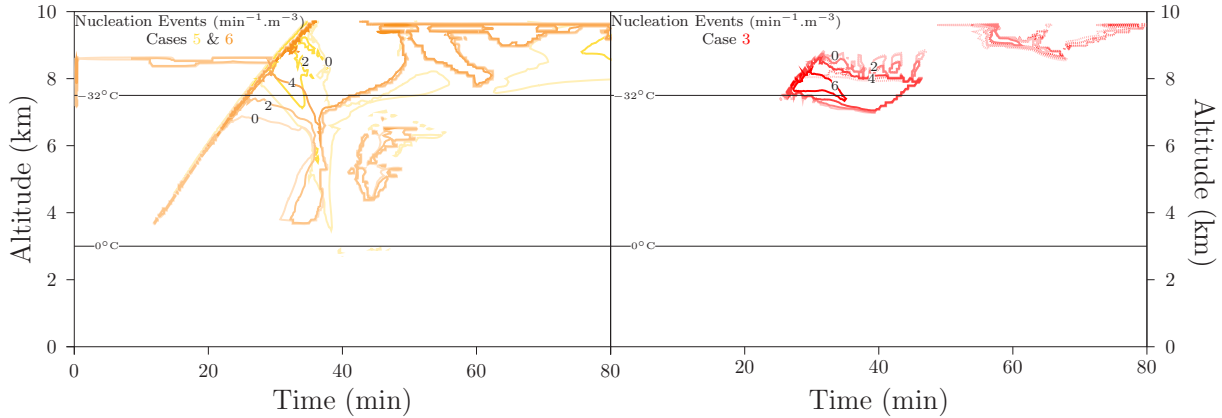
Figure 5.13 – Ice nucleation rate (decimal logarithm of the number of events per cubic meter and per minute) simulated by DESCAM as a function of altitude and time ( a , left) for the cases with only deposition nucleation active (orange contours) and only contact freezing active (yellow contours), and ( b , right) for the case with only homogeneous nucleation active (red contours) on droplets (continuous) and on aerosol particles (dotted).
