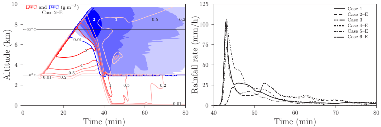
Figure 6.8 – (a, left) Liquid water content ( \text{g.m}^{-3} , red) and ice water content ( \text{g.m}^{-3} , blue) simulated by DESCAM as a function of altitude and time for the case with all minerals active as INP and all ice nucleation mechanisms active (case 2-E). (b, right) Time evolution of the rainfall rate ( \text{mm.h}^{-1} ) for the only-liquid case (case 1, continuous), homogeneous nucleation (case 3, short dashed-dotted) and all minerals cases for all ice processes (case 2-E, dashed), immersion freezing (case 4-E, short dashed), contact freezing (case 5-E, dotted-dashed) and deposition nucleation (case 6-E, double dotted-dashed).
