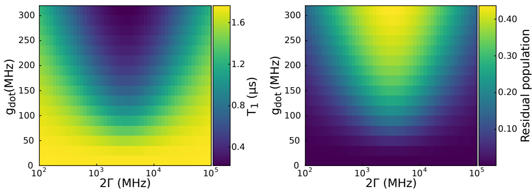
FIGURE 5.1: Transmon relaxation and equilibrium excited population:
