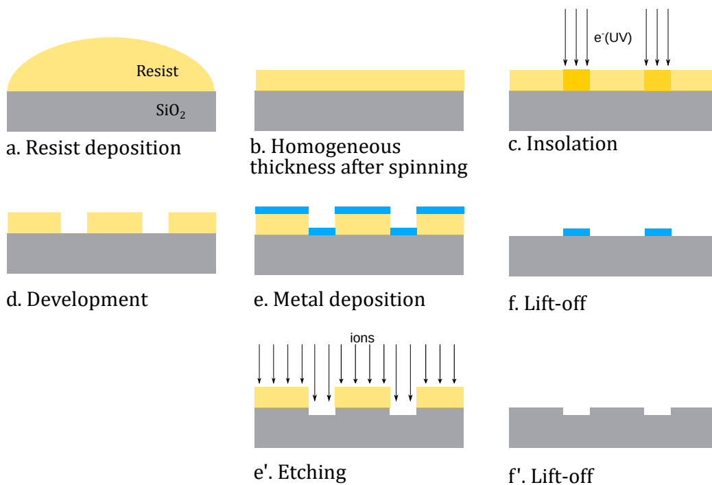
FIGURE 3.9: Lithography principle:
