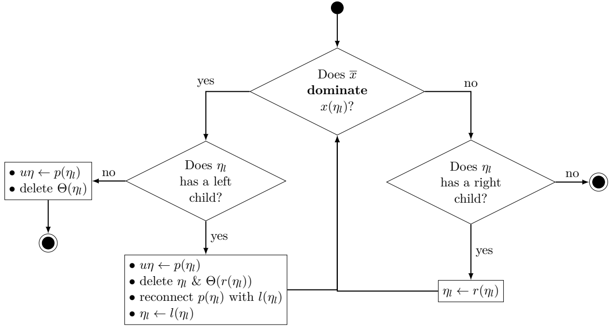
Figure 3.4 – The LeftPruning procedure of an AVL-Archive called from a node \eta_l \in \Theta(l(\eta)) with a candidate solution \bar{x} \in X .
