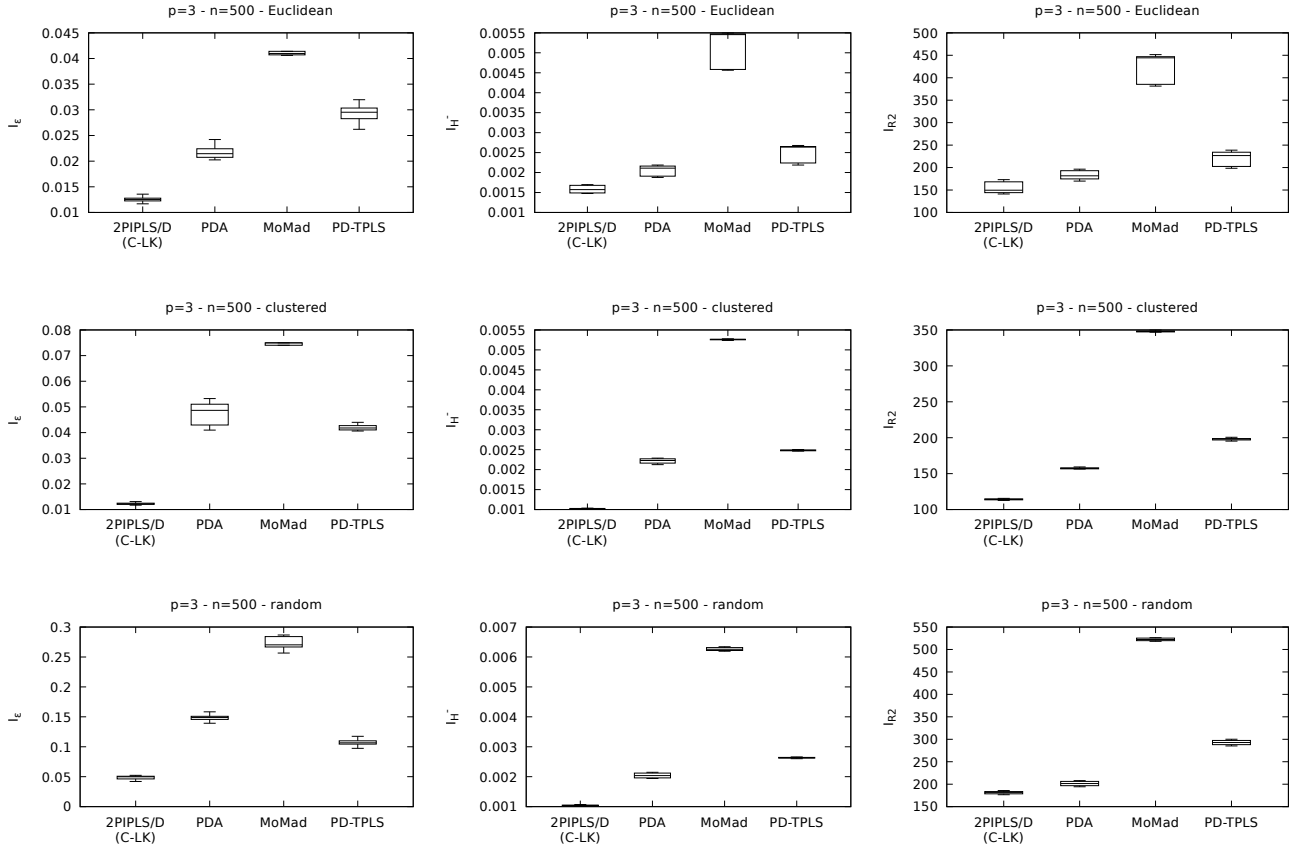
Figure 5.19 – I_\epsilon (left), I_H^- (middle) and I_{R2} (right) performance comparison between 2PIPLS/D (with C-LK optimizer), PDA, MoMad and PD-TPLS on tri-objective instances of size 500.
