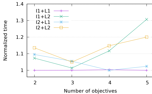
Figure 3.16 – Evolution of the running time of different combinations of splits in function of the number of objectives.
