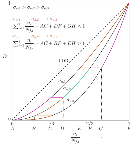
Figure 1.8: Comparison between LDR and NLDR
