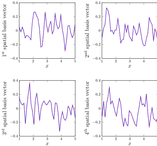
Figure 3.4: First four spatial basis vectors using SVD ( \rightarrow ) and KLE ( \dashrightarrow )
