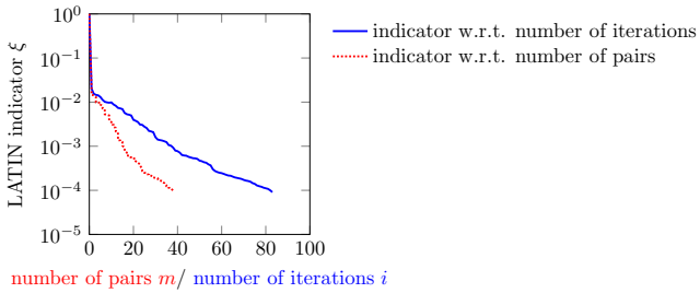
Figure 4.15: Evolution of the LATIN indicator with respect to the number of PGD pairs or LATIN iterations for the pre-damaged structure
