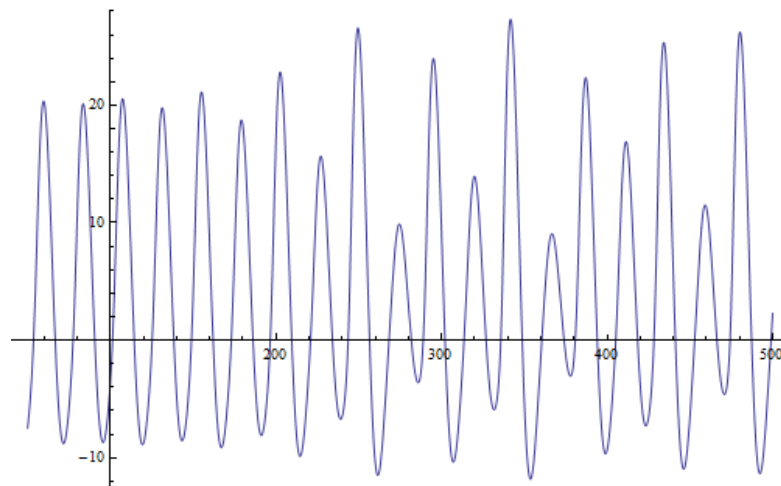
FIGURE 2.8: The chaotic motion of u . a = 0.7, b = 0.3, \epsilon = 7.17, \nu = 4.09, \zeta = 0.5, \rho = 1.9, u_0 = 0.3, v_0 = 0.2, m_0 = 0.3/
