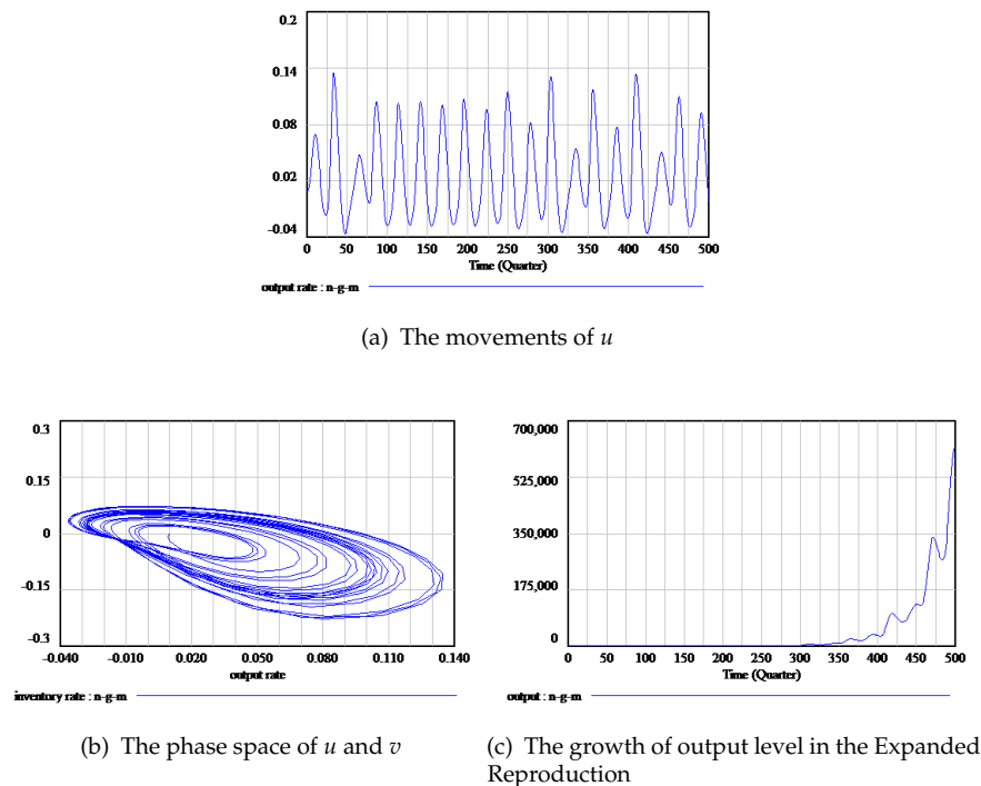
FIGURE 2.13: Expanded Reproduction with the chaotic motion(System dynamic modeling): a = 0.7, b = 0.3, \epsilon = 5, \nu = 5.3, \zeta = 0.025, \rho = 0.675, u_d^t u_0 = 0.01, v_0 = 0, m_0 = 0.03
