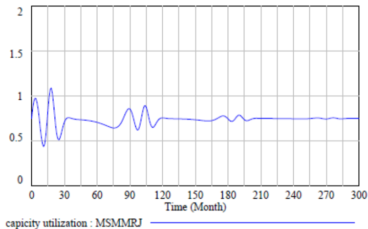
FIGURE 4.14: Enhancing stability, \zeta = 2.25
