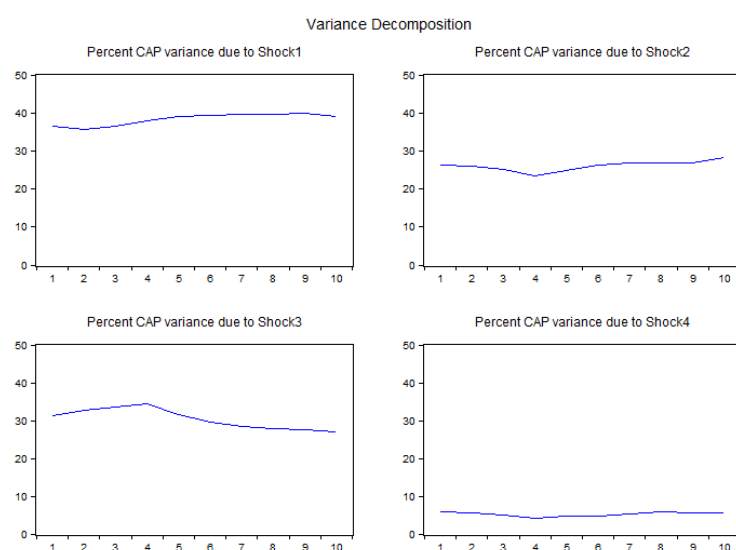
FIGURE 8.14: Variance decomposition of 1980-2005 SVAR with DSTR
