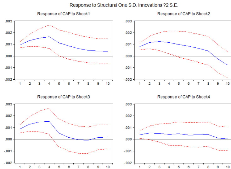
FIGURE 8.12: Structural impulse response: 1980-2005 SVAR with DSTR
