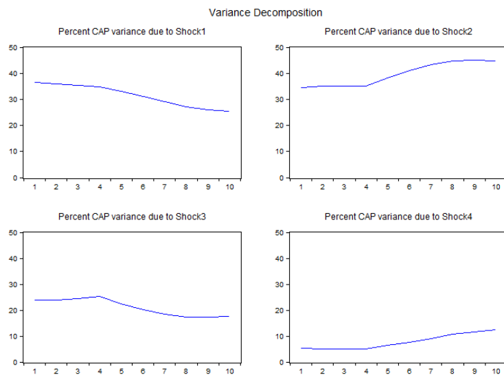
FIGURE 8.13: Variance decomposition of 1980-2005 SVAR without DSTR
