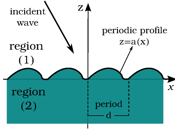
Figure 4.12 – The general situation considered for the C-method.
