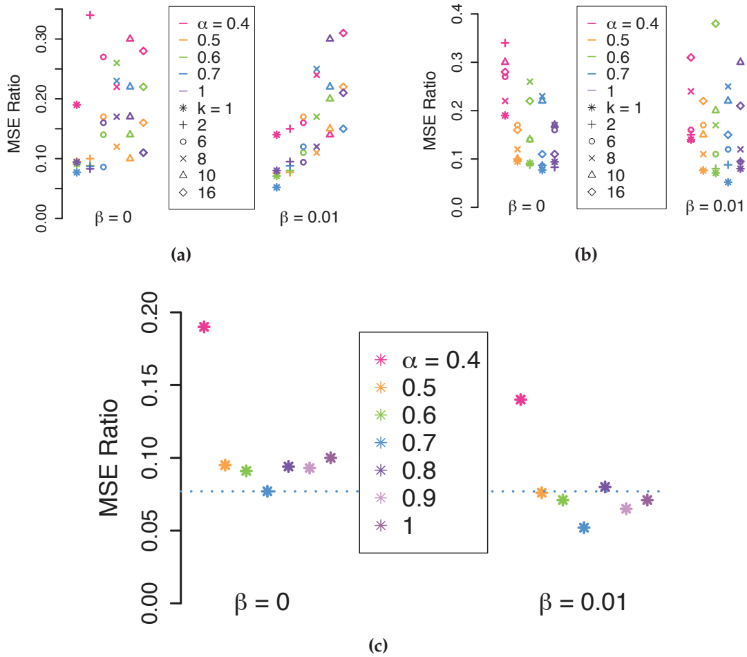
FIGURE 3.4: MSE ratios obtained with \beta = 0 and 0.01 . (a) and (b) both represent the same MSE ratios but differ on the arrangement of the points. Each color corresponds to a value of \alpha and each shape corresponds to a value of k , (a) each vertical alignment of five points corresponds to a fixed value of k for five different values of \alpha , (b) each vertical alignment of six points corresponds to a fixed value of k for six different values of \alpha . (c) MSE ratios obtained with k = 1 and different values of \alpha . The horizontal dotted blue line represents the lower MSE ratio obtained with k = 1 and \beta = 0 among different values of \alpha . See main text for details about k , \alpha and \beta .
