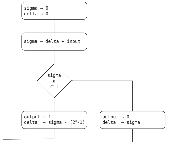
FIGURE 2.28 – Algorithme d'un DAC \Sigma/\Delta
