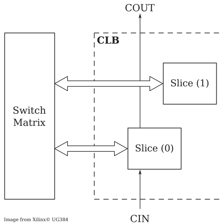
FIGURE 3.1 – Organisation d'un Configurable Logic Block
