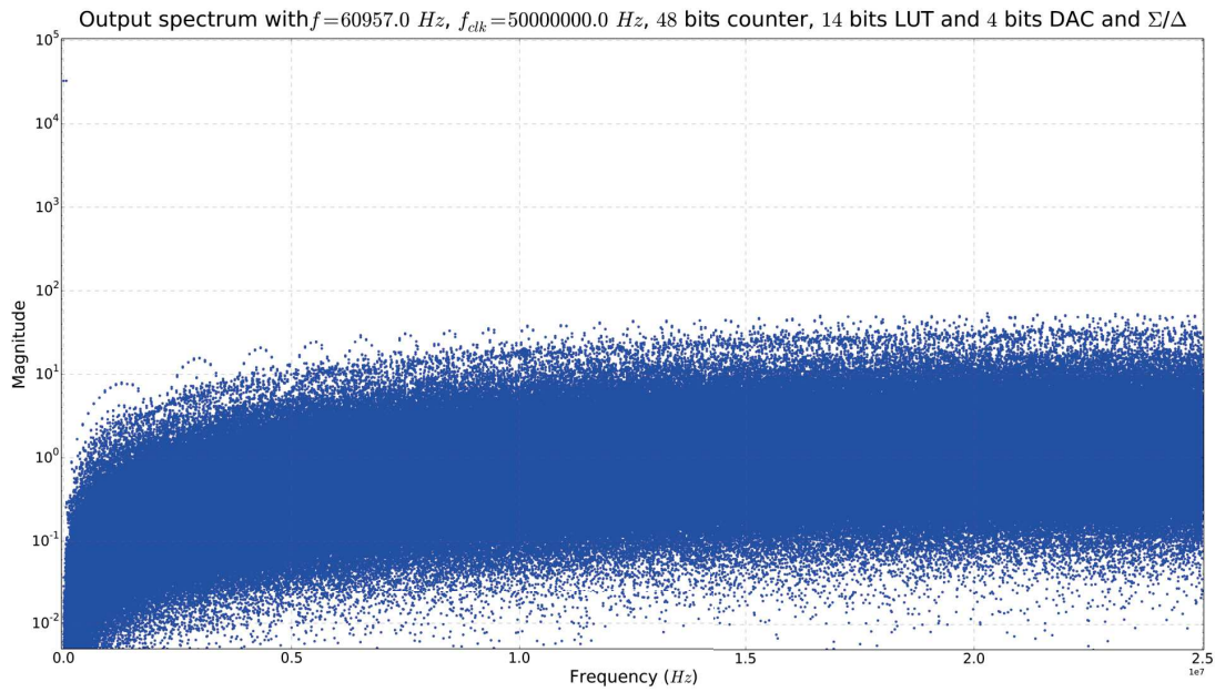
FIGURE 2.32 – Spectre du signal de la figure 2.31
