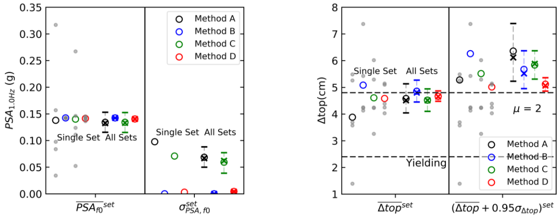
Figure 3.3.2: Distribution of PSAs at 1.00 Hz and \Delta_{top} with a single set versus all sets for each GMSM method. The spectrum compatible selection is explained in Figure 3.2.1. Each grey dot shows the value of a GM. The mean of the set distribution is plotted with the unfilled circles. The median is shown with the cross markers. The 16 th and 84 th percentiles are plotted with the horizontal bars. The color code shows the method in the legend box.
