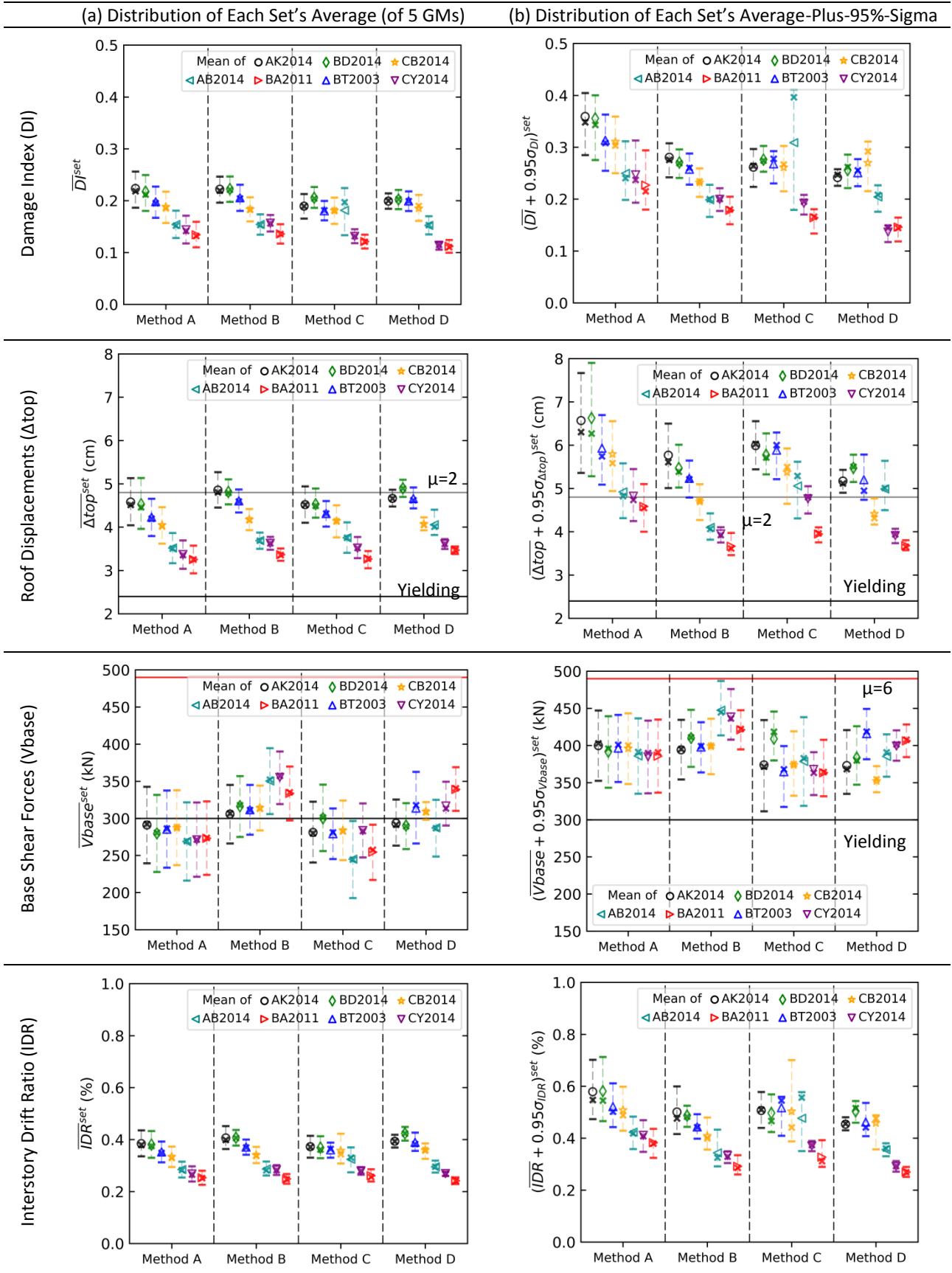
Figure 3.3.4: Distribution of structural response (on column-wise) with all GM sets considering intraset variability with the symmetric tolerances. Each set includes five ground motions. The upper and lower amplitude tolerances are -30% and +30% of the target for Methods A, B, and C, and between -5% and +5% of for Method D. (continued)
