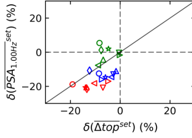
(h) S8b: SDOF-R2 at 1.00 Hz
