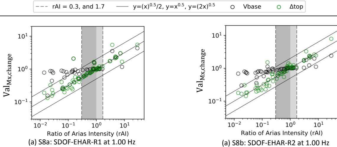
Figure 2.5.2: Comparison of the ratio of Arias intensity (rAI) in Method C and the corresponding change in structural responses. The x and y-axes are in the logarithmic scale. The change in the base shear forces (Vbase) at the corresponding rAI is plotted with the black circles. The change in the roof displacements ( \Delta_{top} ) at the corresponding rAI is plotted with the green circles. The change is defined according to Equation 2.3.1. rAI greater than the unity implies an amplification of the Arias intensity and vice versa. The ratio of the response greater than the unity implies an increase in the structural response and vice versa. Each data represents a loosely spectrum matched GM according to the target, which is the median of AK2014 for the scenario of M7.0R40, Vs450, and normal fault. The permitted level of rAI is between 0.3 and 1.7. The S8a model is designed to resist the lateral design forces linearly. The S8b model is designed for half of the lateral design forces and exhibits more inelastic behavior.
