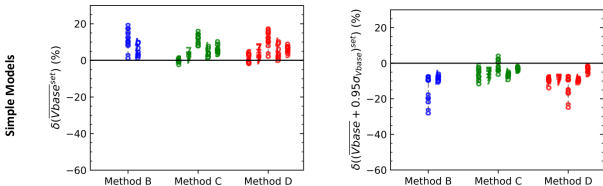
Figure C.2.11: The difference in mean of base shear force ( V_{base} ) distributions with asymmetric tolerances. The spectrum compatible selection is made as explained in the caption of Figure C.2.9. The markers are shown with the ID of the structural model given in the legend above the subfigures. The differences are quantified according to Equations 3.4.1 and 3.4.2. Methods B, C, and D are shown with blue, green, and red colors, respectively. The negative values represent the underprediction relative to Method A and vice versa.
