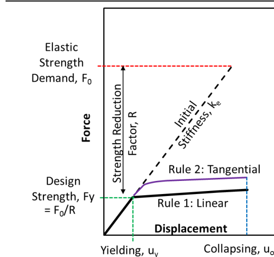
Figure 2.4.1: Material behavior models of simple models and the employed design concept.
