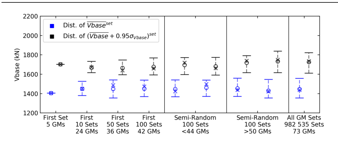
Figure A.7.2: Distribution of Vbase of SDOF's (R2) displacements ( \Delta_{top} ) with the inclusion of the various amount of GM sets. First set, first 10 sets, first 50 sets, and first 100 sets are taken from the previous graph and are included for comparison. They are the sets that are commonly selected in the current practice. They have 5 GMs, 24 GMs, 36 GMs, and 42 GMs, respectively. All GM sets have 982 535 GM sets and use 73 GMs. There is a difference in the amount of GMs and the distribution of GM sets. As a result, two different approaches are used to retrieve four semi-random 100 GM sets. The first approach is to select two semi-random 100 sets having less than 44 GMs, which cover 60% of all GMs. The second approach is to select two semi-random 100 sets with at least 50 GMs, which cover 75% of all GMs.
