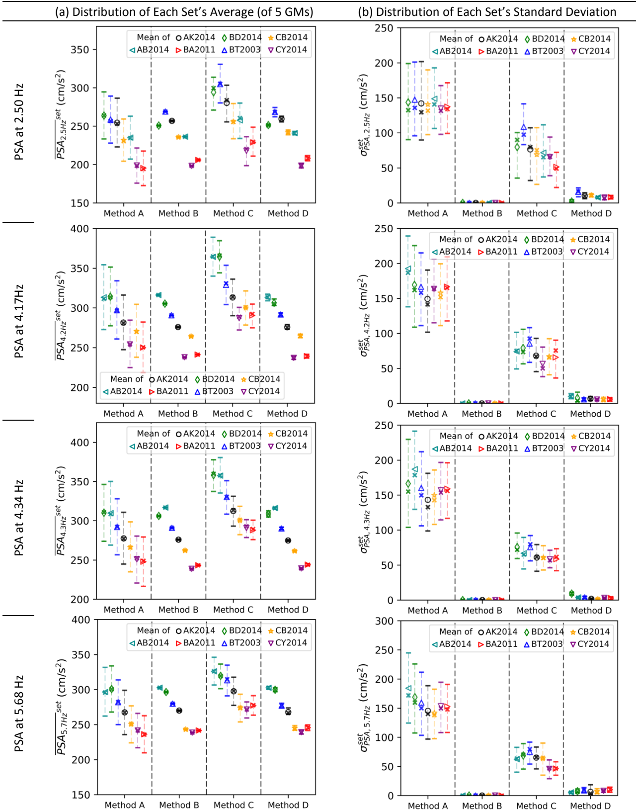
Figure C.1.1: Distribution of pseudo-spectral accelerations (PSA) at f_0 (in row-wise) with all GM sets considering each set's average in column (a) and each set's standard deviation in column (b) with the symmetric tolerances. Each set includes five ground motions. The upper and lower amplitude tolerances are -30% and +30% of the target for Methods A, B, and C, and between-5% and +5% of the target for Method D. The frequency range is from 0.50 Hz and 20.0 Hz. The target is obtained for the scenario of M7.0R40, Vs450, and normal fault as explained in Section 1.4. Means are demonstrated with the markers and colors in the legend box for corresponded GMPEs. Medians are shown with the cross markers. The 16 th and 84 th percentiles are plotted with the horizontal bars.
