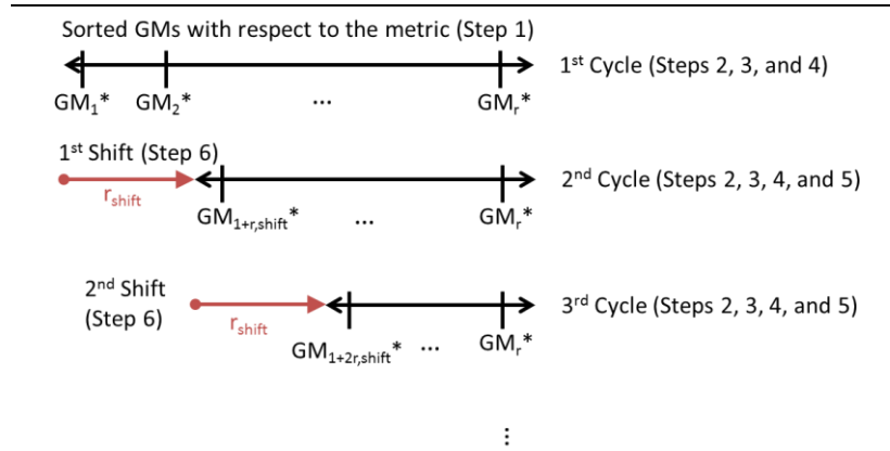
Figure 1.11.4: Sketch of the cycle-and-shift algorithm. *GMs are sorted in an increasing metric value, i.e., GM_1 gives the least metric distance.
