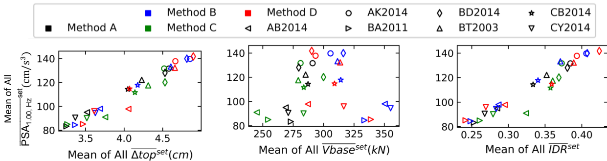
Figure C.1.6: Mean of PSA distributions at f_0 (y-axis) versus mean of structural response distributions (x-axis) such as \Delta top , Vbase , and IDR for the S1 model (8-Story RC). The means of all set distribution are obtained from Figures C.1.1, C.1.2, C.1.3, and C.1.4. Each point represents the mean \Delta top estimate from a GMPE used as a target given in the legend box. Methods B, C, and D are plotted with blue, red, and red, respectively.
