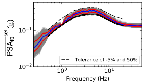
Method B: Linearly Scaled Records to PSA at 1.0 Hz
