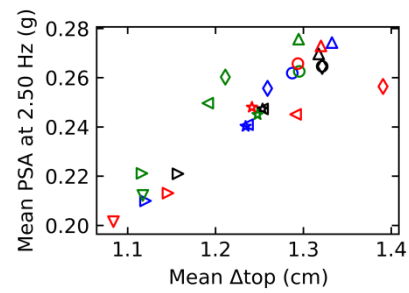
(i) S9: SDOF-R2 at 2.50 Hz
