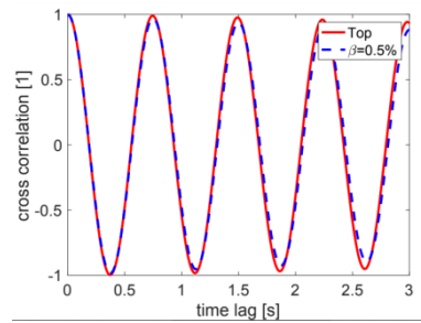
(b) S2: 7-Story RC Building
