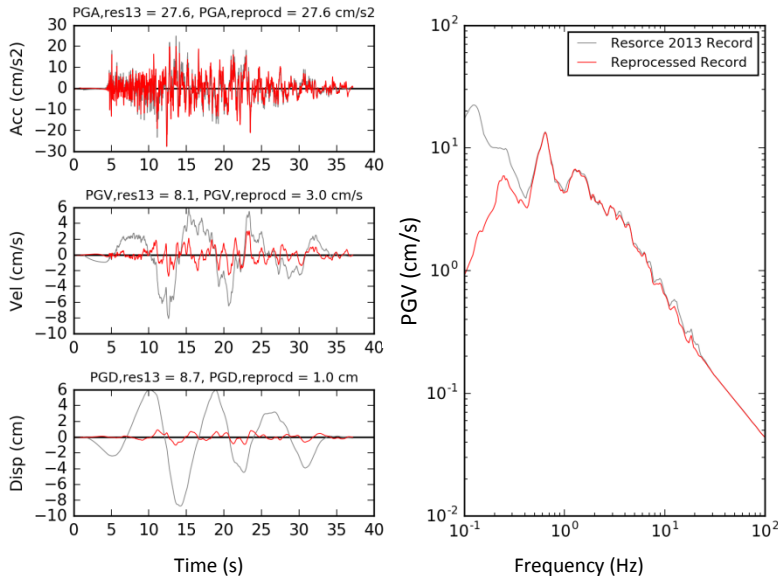
Figure A.2.9: Time- and frequency-domain characteristics of the differently processed records. The record is from the Duzce earthquake (station no 9900) with Mw 7.1, R_{hypo} 49 km and Vs30 455 m/s. Column (a) shows the acceleration, velocity, and displacement time-histories of the processed record in Collection of Databases in grey and the processed record in this study in red. In column (b), the comparison of the spectral shapes is shown. In column (c), the signal processing is explained.
