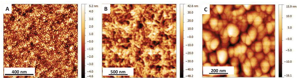
Figure S7. Atomic force microscopic images of (A) Spheres (PMAA 47 -PMMA 185 , 15 w/w %) (B) Worms (PMAA 47 -PMMA 356 , 15 w/w %) (C) Vesicles (PMAA 47 -PMMA 356 , 15 w/w %) blended with INPs coated with PMAA 47 -PQDMAEMA 50 .
