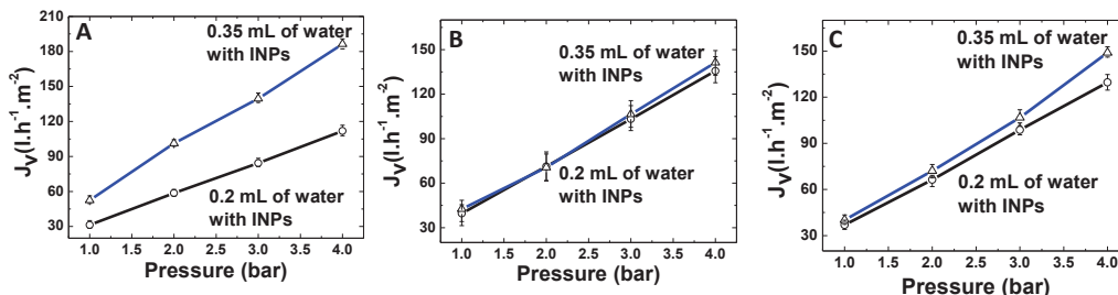
Figure 4.6. The flux and profile for membranes containing (A) PMAA 47 (B) PMAA 47 -PQDMAEMA 50 (C) DMSA coated iron oxide nanoparticles prepared using spin coating procedure.
