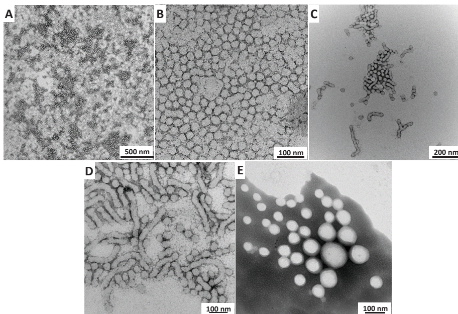
Figure S4. TEM images of PMAA 27 -PMMA y at 15 w/w% total solids content where (A) y=71 ; Spheres (B) y=106 ; Spheres (C) y=130 ; Spheres + Short worms (D) y=194 ; Spheres + Short worms (E) y=230 ; Vesicles.
