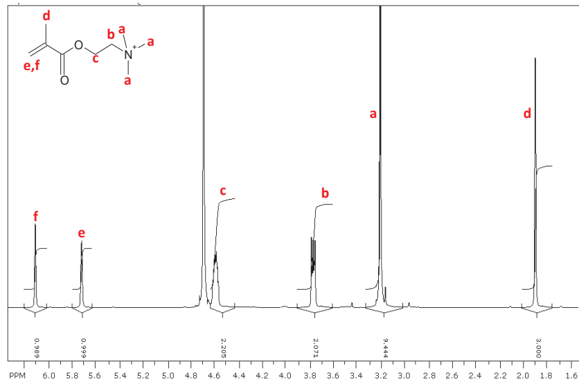
Figure S4. NMR Spectra of QDMAEMA monomer in \text{D}_2\text{O} .
