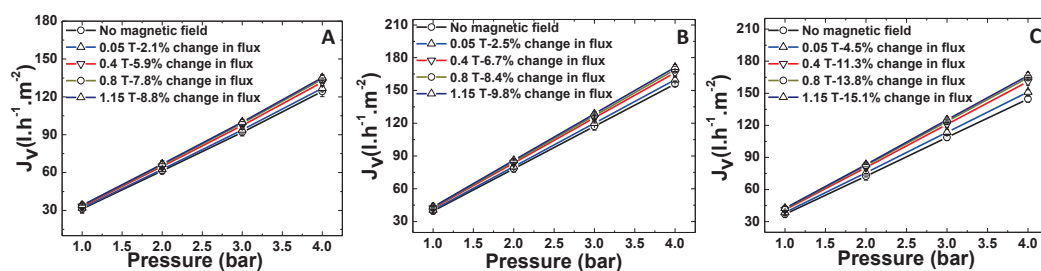
Figure S7. The flux and profile for membranes containing 0.2 mL of (A) PMAA 47 (B) PMAA 47 -PQDMAEMA 50 (C) DMSA coated iron oxide nanoparticles prepared using spin coating procedure (Filtration carried out under magnetic field strength of 0 T to 1.15 T).
