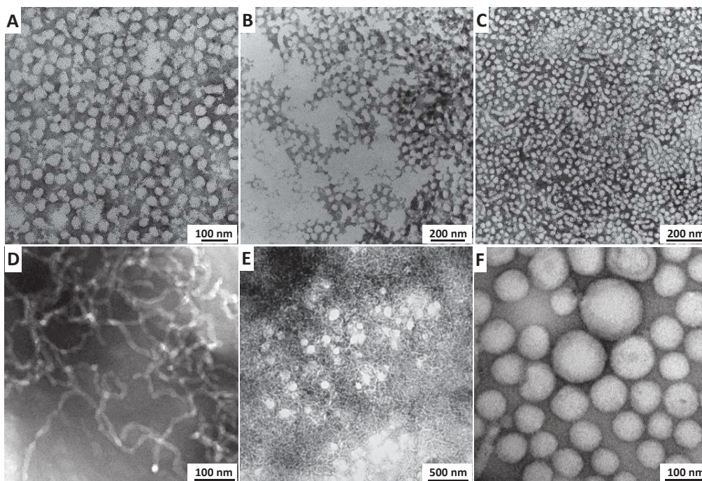
Figure S12. TEM images of PMAA 47 -PMMA y at 27.5 w/w% total solids content where (A) y = 122 ; Spheres (B) y = 192 ; Spheres (C) y = 207 ; Spheres + Short worms (D) y = 256 ; Worms (E) y = 315 ; Worms + Vesicles (F) y = 359 ; Vesicles.
