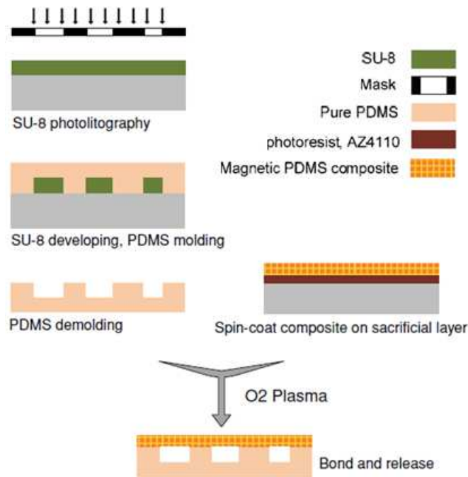
Figure 1.2.8. Synthesis of magnetic membrane (Reprinted from Pirmmoradi et al. , J. Micromech. Microeng. 20 (2010) 1-8)
