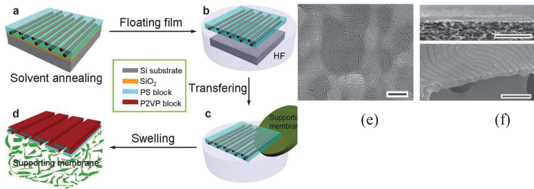
Figure 1.1.2. (a-d) Schematic illustration of the preparation of composite membranes using block copolymer films with slitted pores as selective layers.(e-f) SEM images of the morphologies obtained. Reprinted with permission from Ref. 22.
