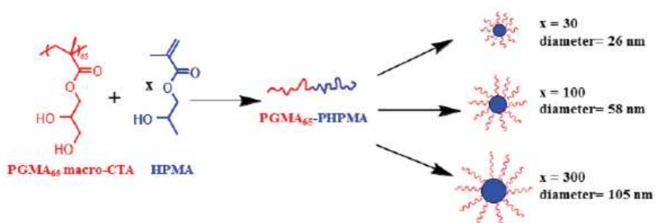
Figure 1.3.8. In situ formation of sterically stabilised PGMA-HPMA nanoparticles by RAFT aqueous dispersion polymerization of HPMA at 70°C. Increasing the degree of polymerization of the core-forming block leads to larger nanoparticles, as judged by dynamic light scattering and transmission electron microscopy. 65
