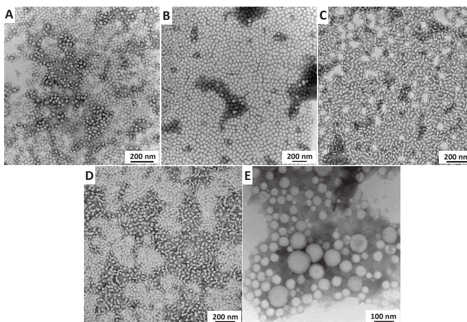
Figure S5. TEM images of PMAA 27 -PMMA y at 25 w/w% total solids content where (A) y=69 ; Spheres (B) y=89 ; Spheres (C) y=106 ; Spheres + Short worms (D) y=187 ; Spheres + Short worms (E) y=251 ; Vesicles.
