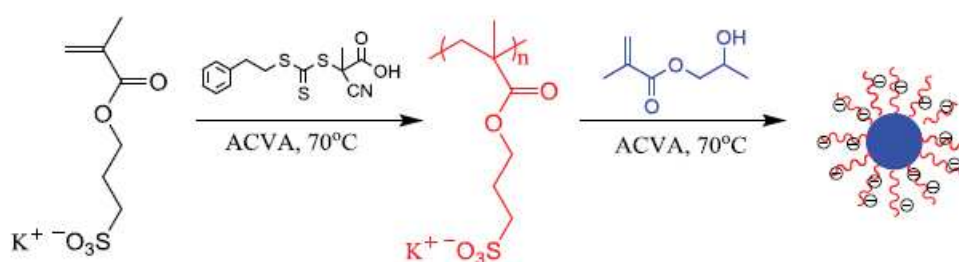
Figure 1.3.11. Reaction scheme for the synthesis of poly(potassium 3-sulfopropyl methacrylate–poly(2-hydroxypropyl methacrylate) (PKSPMA-HPMA) diblock copolymers by RAFT aqueous dispersion polymerization at 70°C. 67
