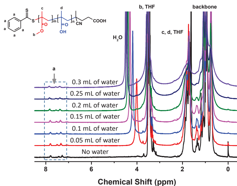
Figure 4.1. ^1\text{H} NMR spectra for PMAA 47 - b -PMMA 69 in a mixture of \text{C}_4\text{D}_8\text{O} (THF- d 8) and \text{D}_2\text{O} .
