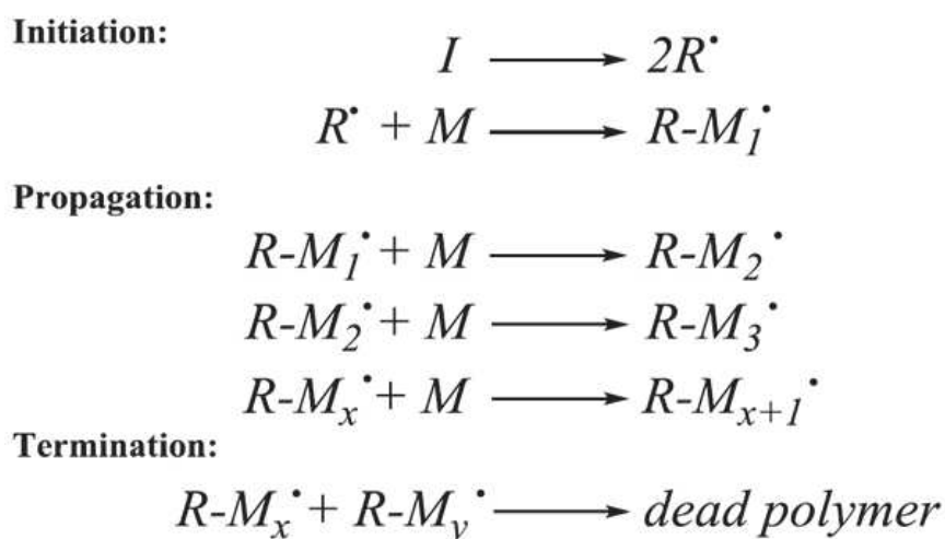
Figure 1.3.2. Mechanism of free radical polymerization. 13
