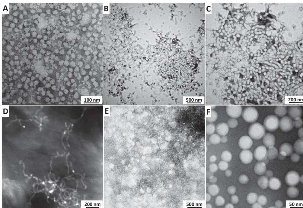
Figure S11. TEM images of PMAA 47 -PMMA y at 25 w/w% total solids content where (A) y = 119 ; Spheres (B) y = 208 ; Spheres + Short worms (C) y = 241 ; Spheres + Short worms (D) y = 257 ; Worms (E) y = 318 ; Worms + Vesicles (F) y = 356 ; Vesicles.
