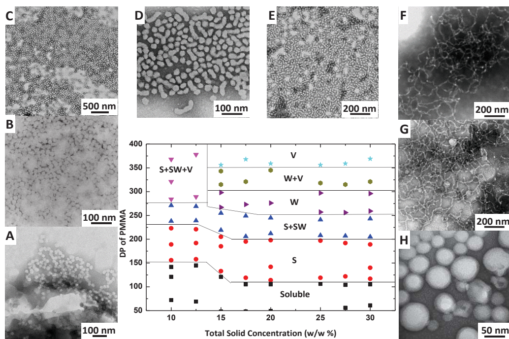
Figure 2.3. Phase diagram constructed for PMAA 47 -PMMA γ diblock copolymer nano-objects prepared by RAFT ethanolic dispersion polymerization at 70 °C. Post mortem TEM images obtained at 20 w/w % varying the length of PMMA block showing the evolution from spheres to vesicles. (A) Y=114, Spheres (B) Y=142, Spheres (C) Y=198, Spheres (D) Y=212, Spheres + Short worms (E) Y=245, Spheres + Short worms), (F) Y=276, Worms (G) Y=345, Worms + Vesicles (H) Y=359, Vesicles. (S denotes Spheres, SW- denotes Short worms, W- denotes Worms, V- denotes Vesicles).
