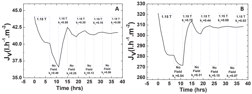
Figure S5. The magnetic ON/OFF cycle after fouling at (A) 0.5 bars and (B) 3 bars of pressure for membrane from Vesicles – Strategy 2.
