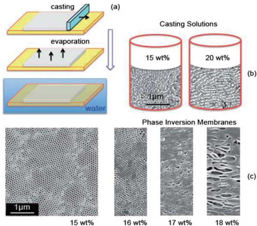
Figure 1.1.1 (a) SNIPS method for membrane fabrication based on PS- b -P4VP in DMF: THF: DOX solvent mixture (b) Cryo- FESEM image of the casting solution (c) FESEM images of top surface of membrane prepared with different block copolymer concentration. Reprinted with permission from Ref. 18.
