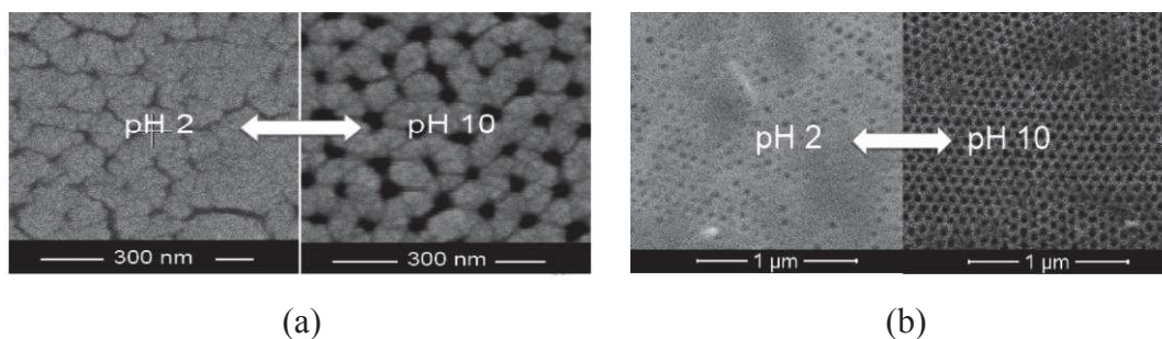
Figure 1.1.11. (a) Cryo-field emission scanning electron microscopy and (b) environmental scanning electron microscopy of PS-b-P4VP membranes casted from a copolymer solution in DMF/THF/Cu ++ , immersed in HNO 3 (pH 2) and NH 4 OH (pH 10) aqueous solutions. Reprinted with permission from Ref. 33.
