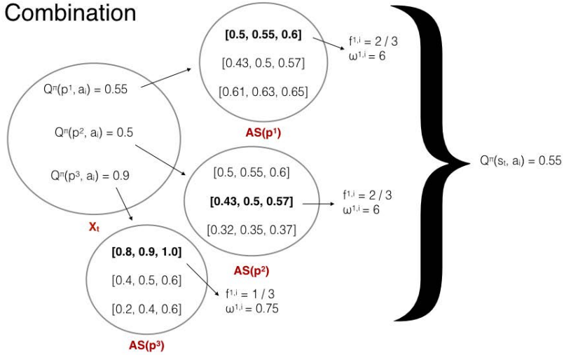
Figure 7.6: Computing the Q -value for a state action pair (s_t, a_i) with GSDMRL.
