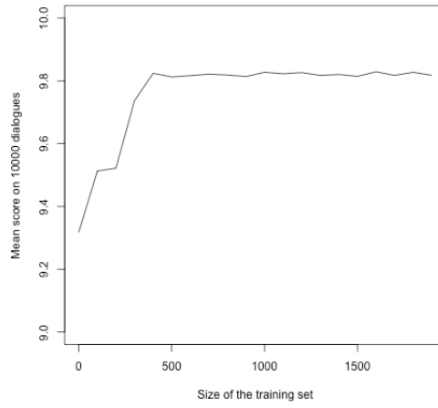
Figure 5.9: Result of the learning with SARSA( \lambda ) of a user behaviour for the appointment scheduling simulator.
