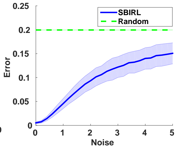
Figure D.2: Distance minimisation error as \sigma grows
