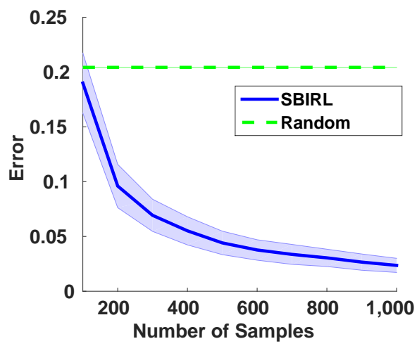
Figure D.1: Distance minimisation error as N_T grows
