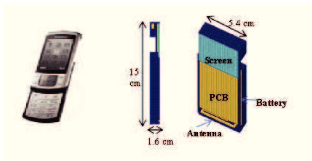
Figure 2.9: Example of digital model of mobile phone
