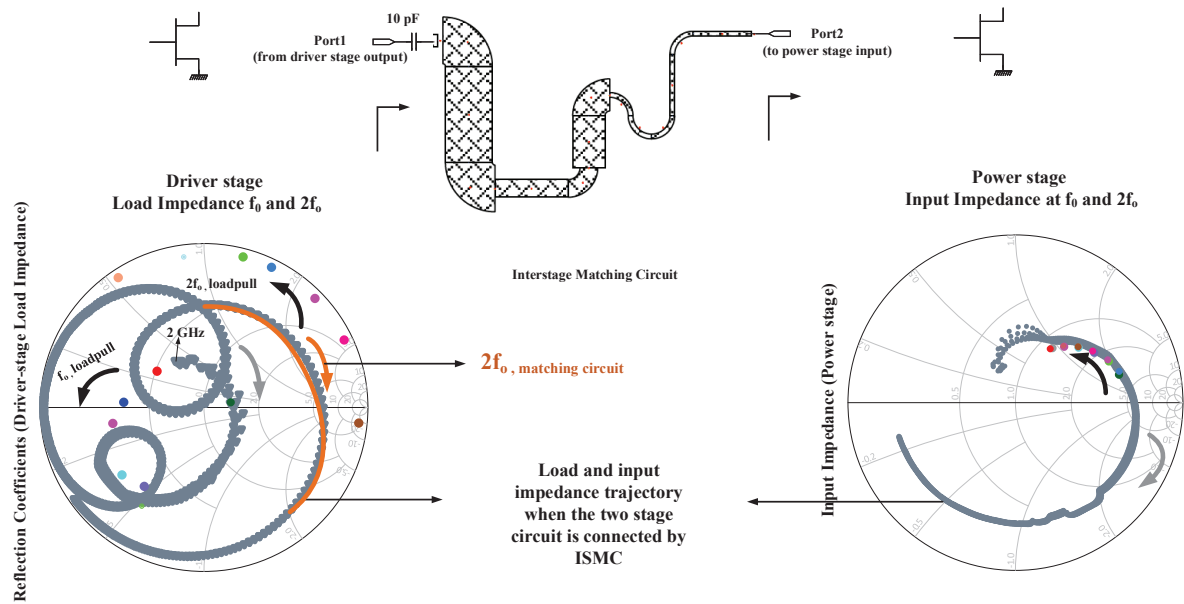
Figure IV.7: Newly optimized inter-stage matching circuit for the new power modulator circuit. The optimum load impedances of the driver stage and the input impedances of the power stage as a function of frequency obtained from loadpull simulations and the impedance trajectory when the inter-stage matching circuit is connected to the two-stage circuit are highlighted.
