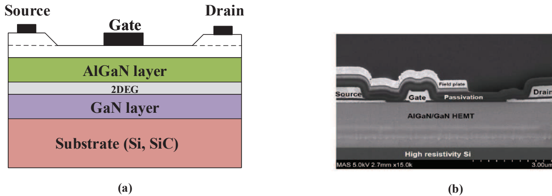
Figure I.18: (a) Simplified cross-section of AlGaN/GaN-HEMT and (b) Cross-section of AlGaN/GaN-HEMT on a Silicon substrate seen with a scanning electron microscope.
