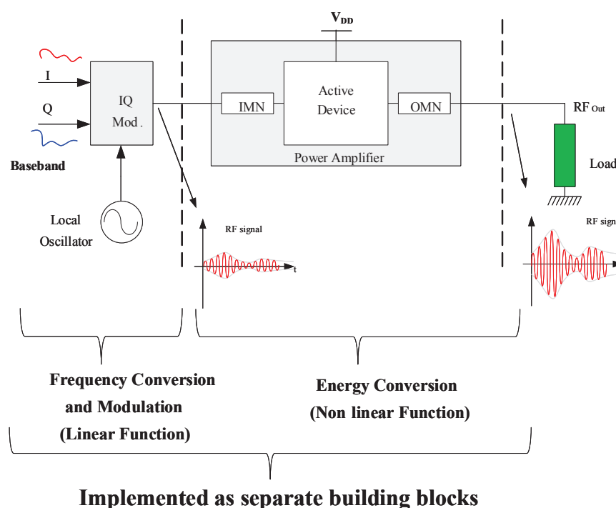
Figure III.1: Conventional transmitter architecture.
