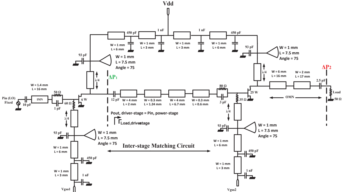
Figure III.28: Electrical design schematic of the two-stage SVG circuit
