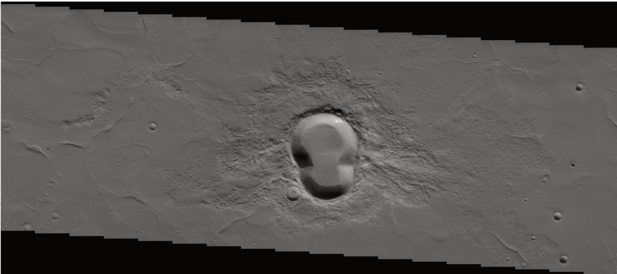
Figure 1.17 – Mars doublet crater. Image credit: NASA/JPL/ASU
