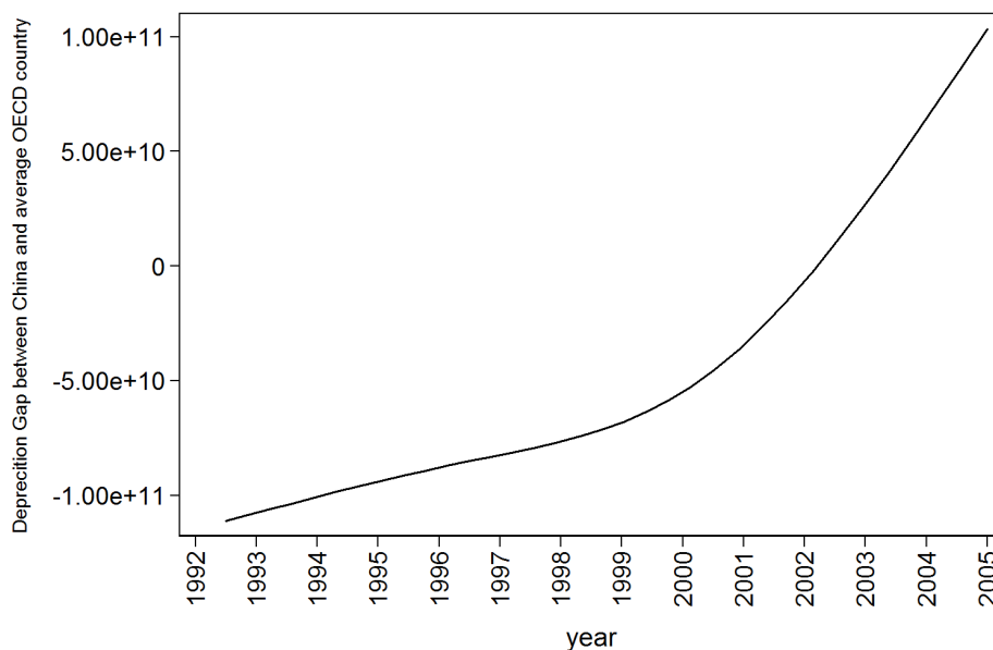
Figure 3.25: Depreciation gap in level \delta_{CHINA} - \delta_{Average\ OECD}
