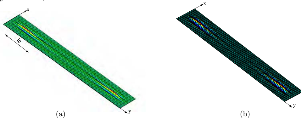
Figure 2.10: Wrinkling patterns near the bifurcation of a rectangular membrane under uniaxial stress load for full shell model (a) and new reduced model (b), N_y = 6.6 \text{ N/mm} .
