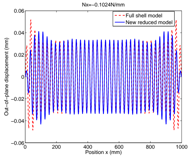
Figure 2.6: Central cross section ( Y=100 \text{ mm} ) of a rectangular membrane under biaxial load further after bifurcation point, N_y = 10 \text{ N/mm} , N_x = -0.1024 \text{ N/mm} .
