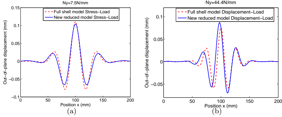
Figure 2.13: Central cross section ( Y=168 mm) of rectangular membrane under uniaxial stress load (a), displacement load (b).
