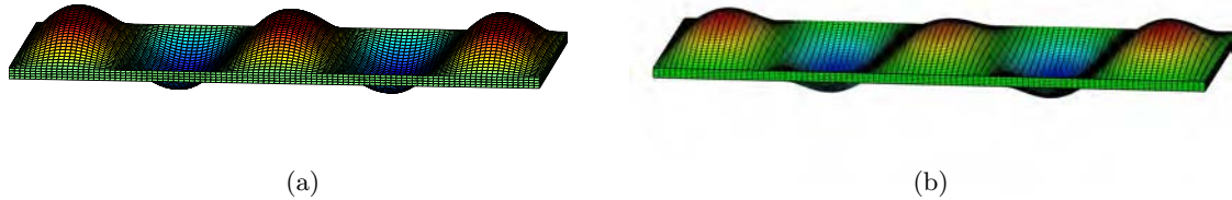
Figure 5.5: The wrinkling patterns obtained by (a) the 2D macroscopic sandwich plate model and (b) the 3D FEM model.
