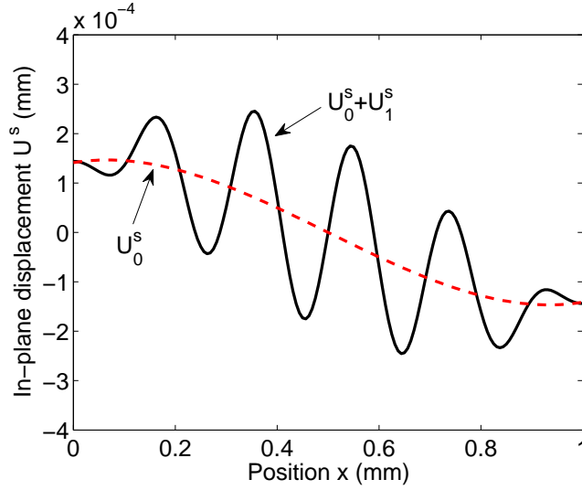
Figure 3.6: Axial displacement distribution along x at z = 0.95 mm after bifurcation point in the substrate. Problem II.
