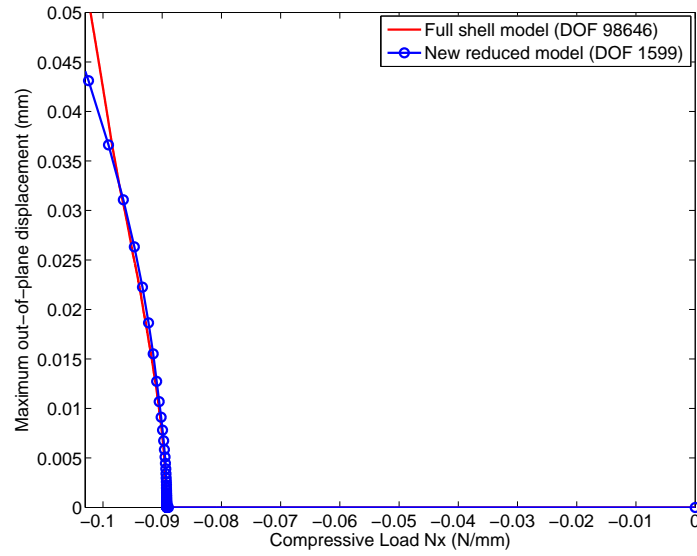
Figure 2.4: Bifurcation path of a rectangular membrane under biaxial load with tensile load N_y = 10 \text{ N/mm} .
