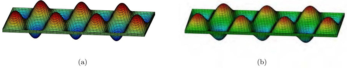
Figure 5.7: The antisymmetrical wrinkling patterns obtained by (a) the 2D macroscopic sandwich plate model and (b) the 3D FEM model.
