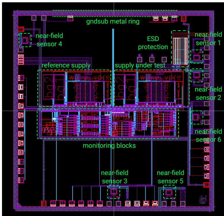
Figure 3.19: Top-cell layout
