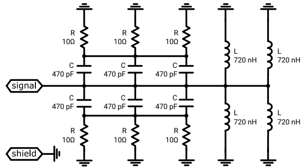
Figure 2.22: Shaping-filter schematic
