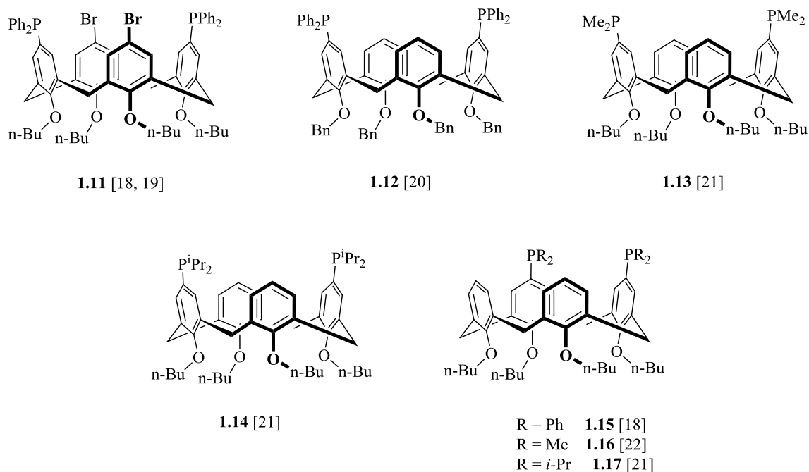
Figure. 1.2. Obtained calix[4]arenyl-diphosphines 1.11-1.17 .
