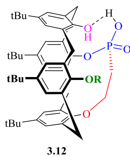
Figure. 3.11. Chiral Brønsted phosphorus acids in “closed” conformation.
