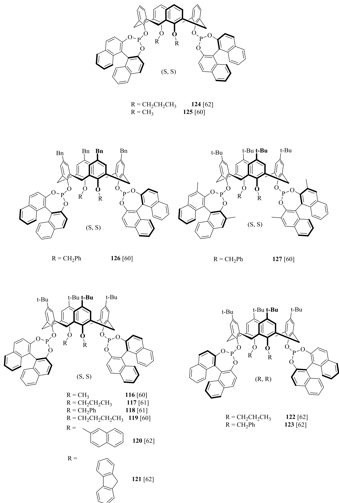
Figure. 1.9. Diphosphites 1.108 – 1.127 .
