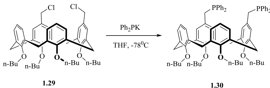
Scheme 1.7. Synthesis of the proximally functionalised calix[4]arene 1.30 .
