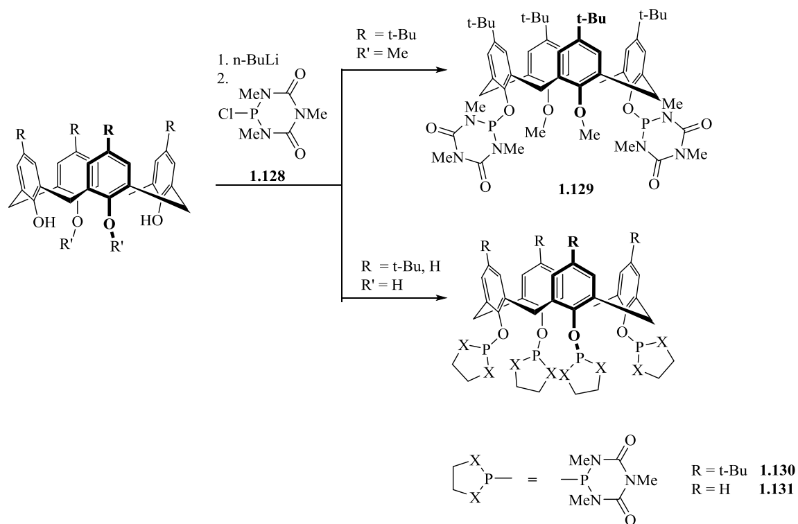
Scheme 1.26. Oxy-phosphorus diamides 1.129-1.131 .
