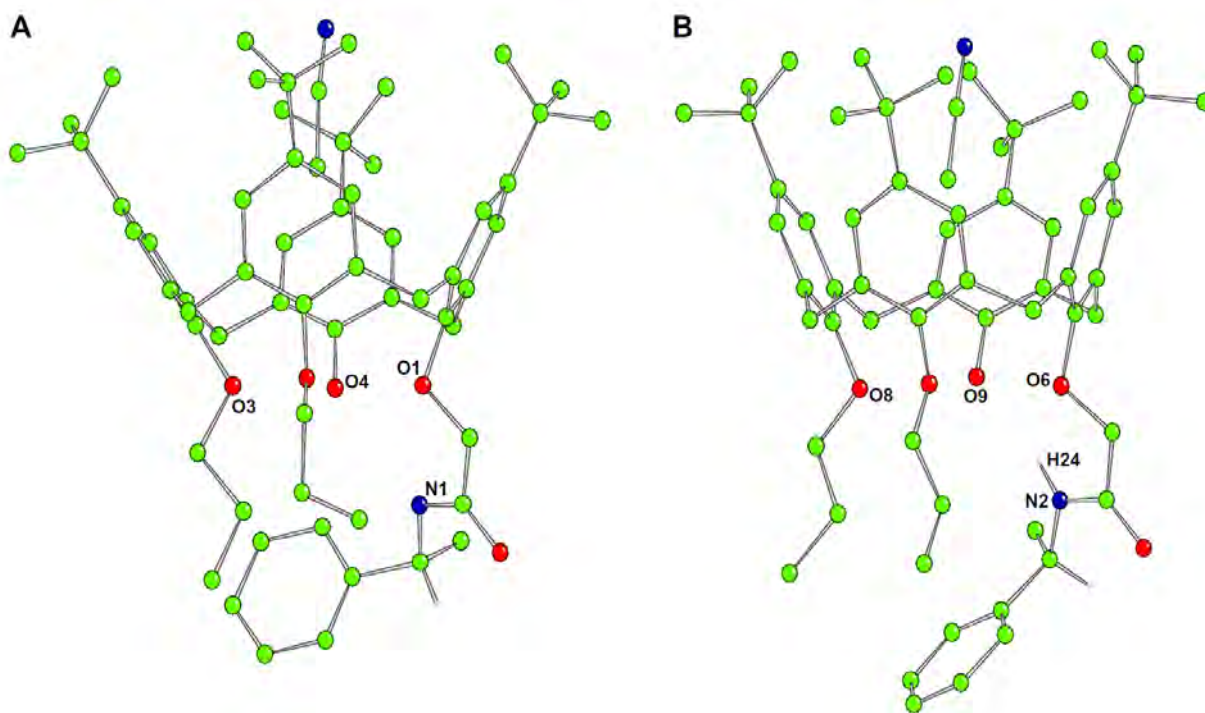
Figure. 3.7. X-ray molecular structure of conformers A and B of calixarene
