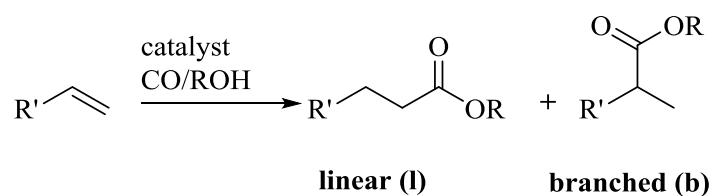
Scheme 1.35. Olefin hydroalkoxycarbonylation.
