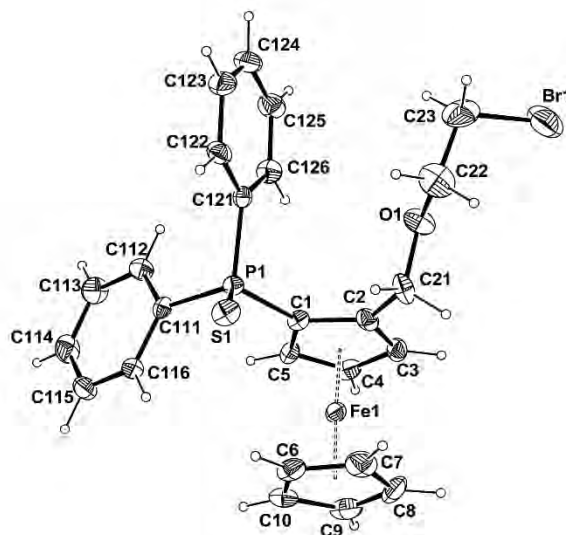
Figure. 2.4. Molecular view of compound 2.7 with the atom labeling scheme. Ellipsoids are drawn at the 50% probability level. H atoms are represented as small circle of arbitrary radii.
