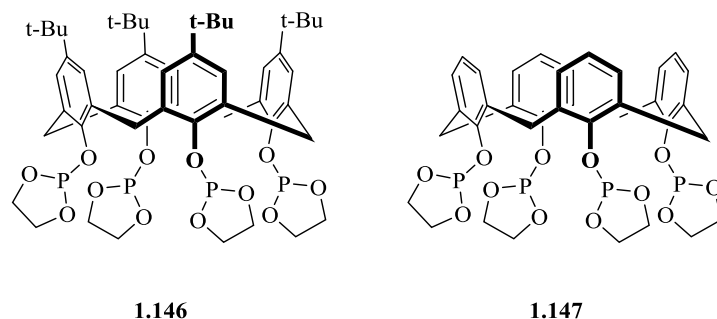
Figure. 1.10. Diphosphites 1.146 and 1.147 .
