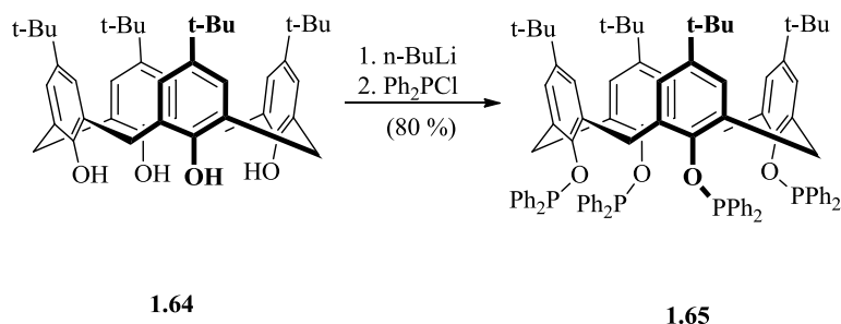
Scheme 1.16. Synthesis of tetraphosphinite 1.65 .
