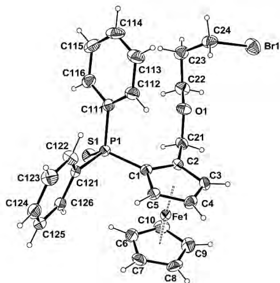
Figure. 2.3. Molecular view of compound 2.6 with the atom labeling scheme. Ellipsoids are drawn at the 50% probability level. H atoms are represented as small circle of arbitrary radii.
