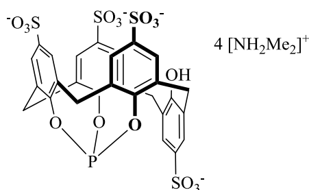
Figure. 1.6. Water-soluble phosphite 1.80 .
