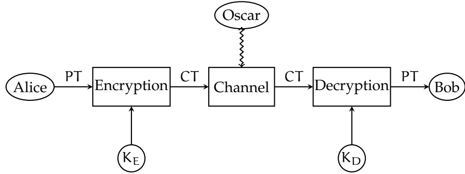
Figure 11: Basic communication scheme studied in cryptography.
