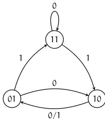
Figure 48: Transition graph for the finite state automaton realizing \delta .
