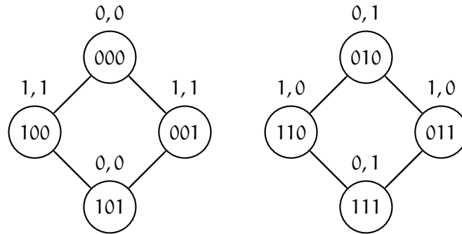
Figure 49: Graph representation of the pairwise balanced bipermutive rules 90 and 150.
