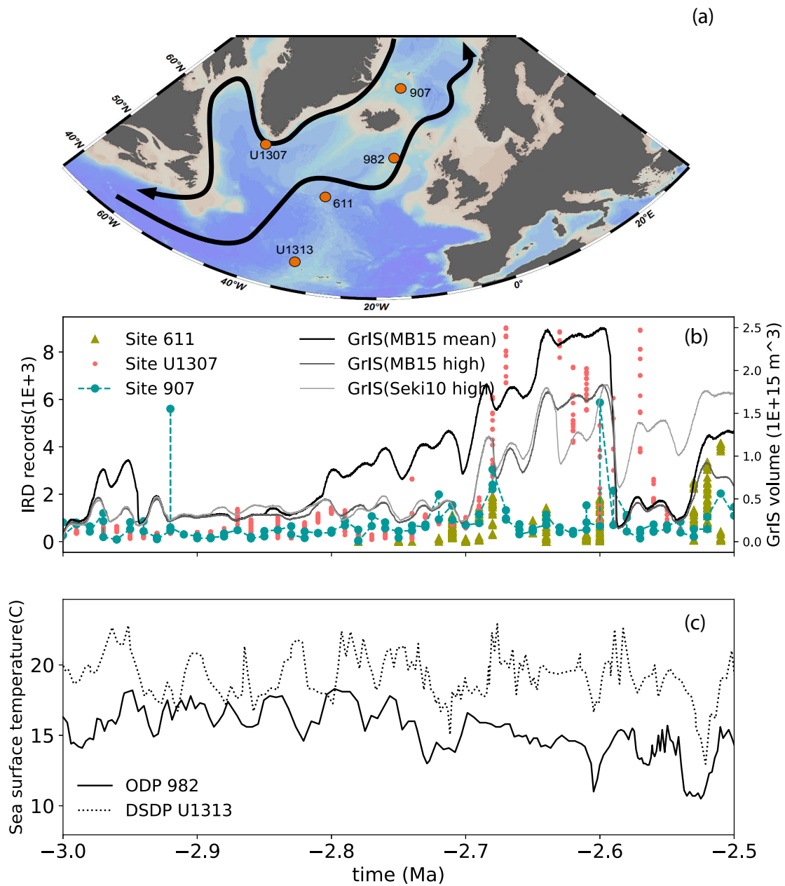
Figure 5.9 – (a) Map showing simplified main ocean currents in NATL and ocean deep drilling sites referenced in this study (Ocean Data View, Schlitz et al.,2012) (b) Related IRD records in the North Atlantic regions: site 907 (Jansen et al., 2000); site U1307 (Sarnthein et al.,2009); site 611 (Bailey et al. 2013) and simulated GrIS volume with the pCO 2 reconstructions of Martinez-Boti et al., 2015 mean and high estimates and Seki et al., 2010 high estimate.; (c) Reconstructed sea surface temperature at ODP site 982 by Lawrence et al. (2009) and IODP site U1313 by Naafs et al. (2010).
