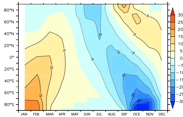
Figure. A.4 Difference in incoming solar radiation at the top of atmosphere between 3.313 Ma and Pre-industrial level (W/m 2 ).
