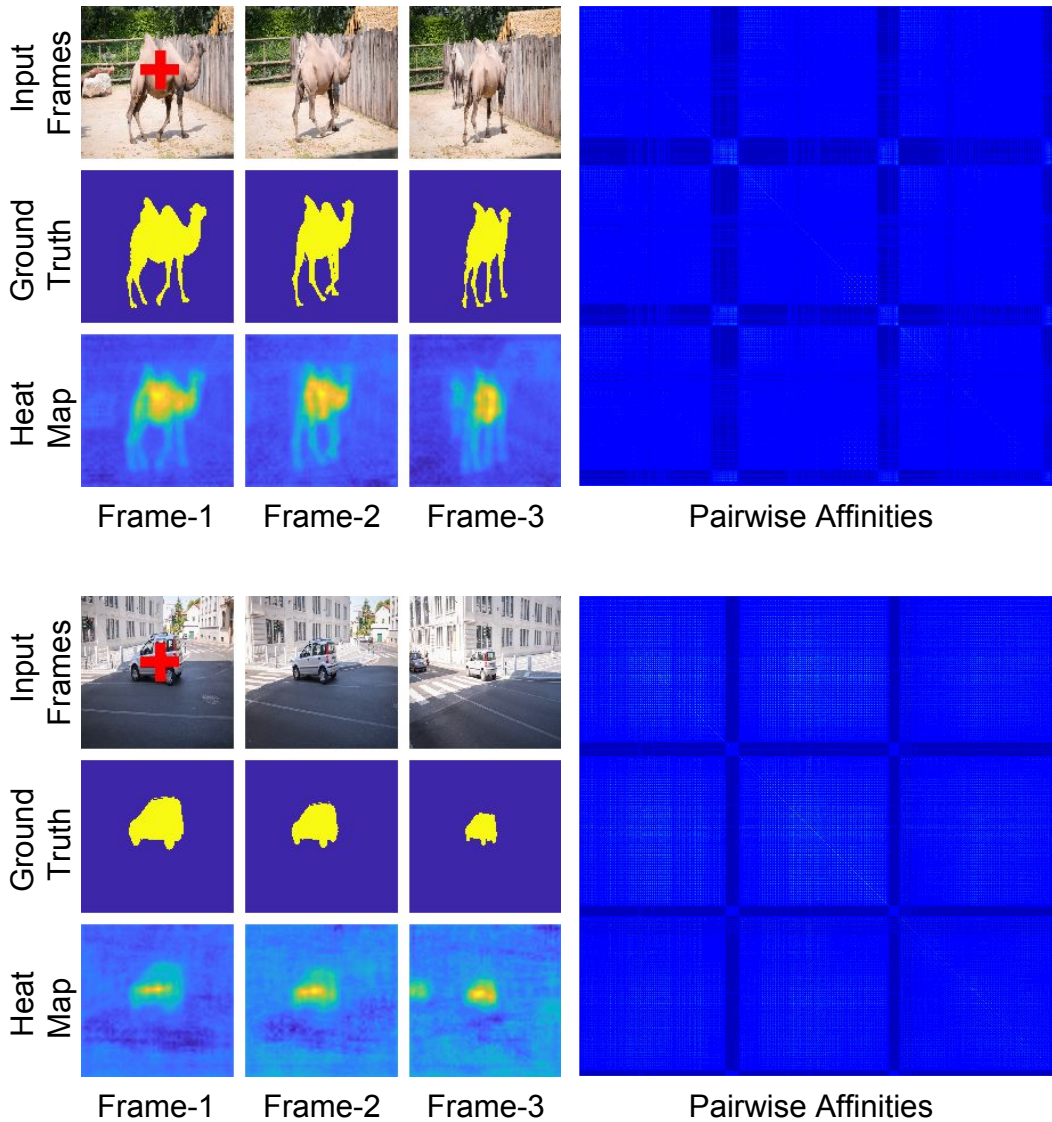
Figure 4.7: Visualization of G-CRF embeddings on 2 videos in the DAVIS dataset. The pairwise affinity between two pixels in the image is given by the dot product of the feature embeddings computed at these two pixels. We choose a reference pixel from the Frame-1 (marked by the red cross). We show the heat-map produced by computing the dot-product of the embedding at the reference pixel, with other pixels in the same frame, as well as in two other frames from the video. We also plot the pairwise affinities between every pair of pixels as a heatmap in the 3 frames of the video in the last column of the figure. Here the pixels are ordered according to their class (background followed by object). The bright areas indicate high affinity between pixels belonging to the same class, and the dull areas indicate low affinity between pixels belonging to different classes.
