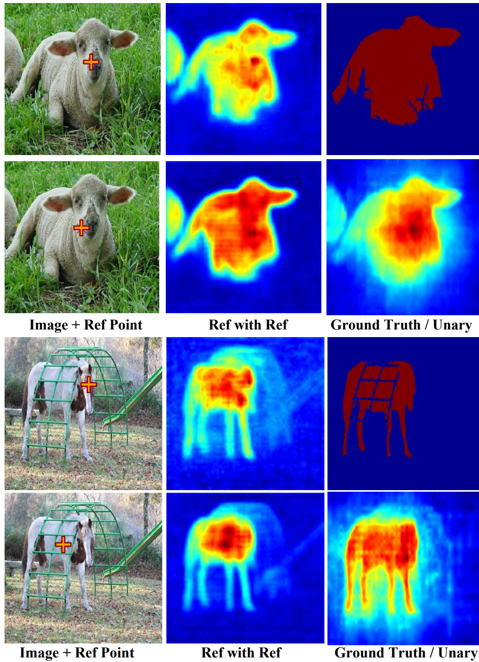
Figure 3.5: Here we visualize how the pairwise terms change as we vary the reference point. These pairwise terms are obtained by our G-CRF embeddings trained for the semantic segmentation task. Column 1 shows the reference pixel ( p^* ), marked with a plus sign, on the image. In column 2, we show the heatmap of the pairwise terms corresponding to p^* taking the ground truth label l^* and other pixels p taking the label l^* , given by A_{p^*,p}(l^*, l^*) = \langle \mathcal{A}_p^{l^*}, \mathcal{A}_{p^*}^{l^*} \rangle . In column 3, we show the ground truth, followed by the heatmap of unary terms delivered by the network.
