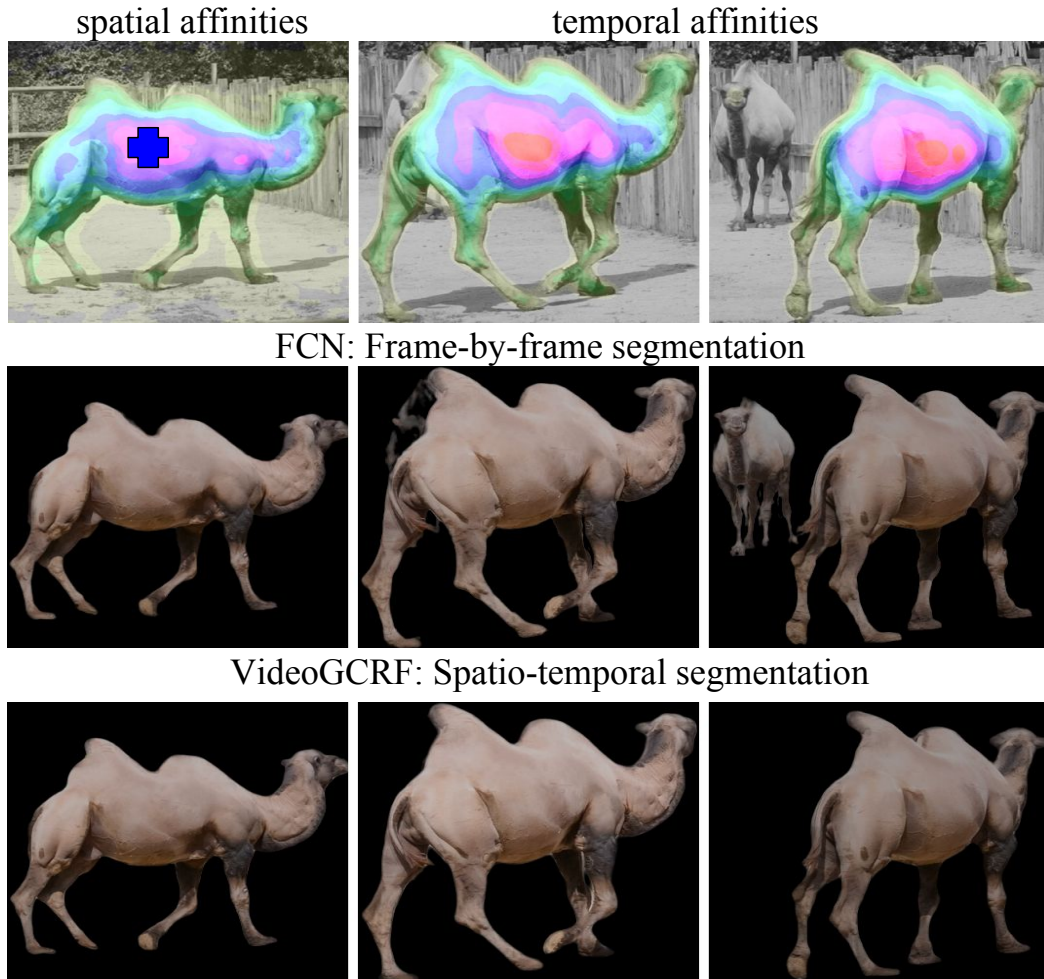
Figure 4.3: Visualization of instance segmentation through VideoGCRF: In row 1 we focus on a single point of the CRF graph, shown as a cross, and show as a heatmap its spatial (inter-frame) and temporal (intra-frame) affinities to all other graph nodes. These correspond to a single column of the linear system in Eq. 4.2. In row 2 we show the predictions that would be obtained by frame-by-frame segmentation, relying exclusively on the FCN’s unary terms, while in row 3 we show the results obtained after solving the VideoGCRF inference problem. We observe that in frame-by-frame segmentation a second camel is incorrectly detected due to its similar appearance properties. However, VideoGCRF inference exploits temporal context and focuses solely on the correct object.
