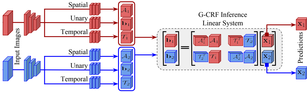
Figure 4.2: VideoGCRF schematic for 2 video frames. Our network takes in 2 input images, and delivers the per frame unaries \mathbf{b}_1, \mathbf{b}_2 , spatial embeddings \mathcal{A}_1, \mathcal{A}_2 , and temporal embeddings \mathcal{T}_1, \mathcal{T}_2 in the feed-forward mode. Our VideoGCRF module collects these and solves the inference problem in Eq. 4.2 to recover predictions \mathbf{x}_1, \mathbf{x}_2 . During backward pass, the gradients of the predictions are delivered to the VideoGCRF model. It uses these to compute the gradients for the unary terms as well as the spatio-temporal embeddings and back-propagates them through the network.
