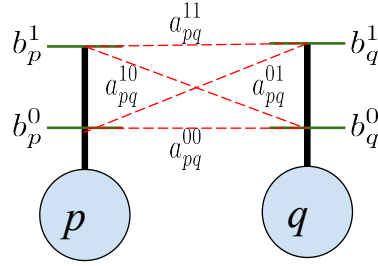
Figure 1.9: 2 pixels, 2 labels toy example. The green solid lines indicate unary terms, and the red dashed lines indicate pairwise terms.
