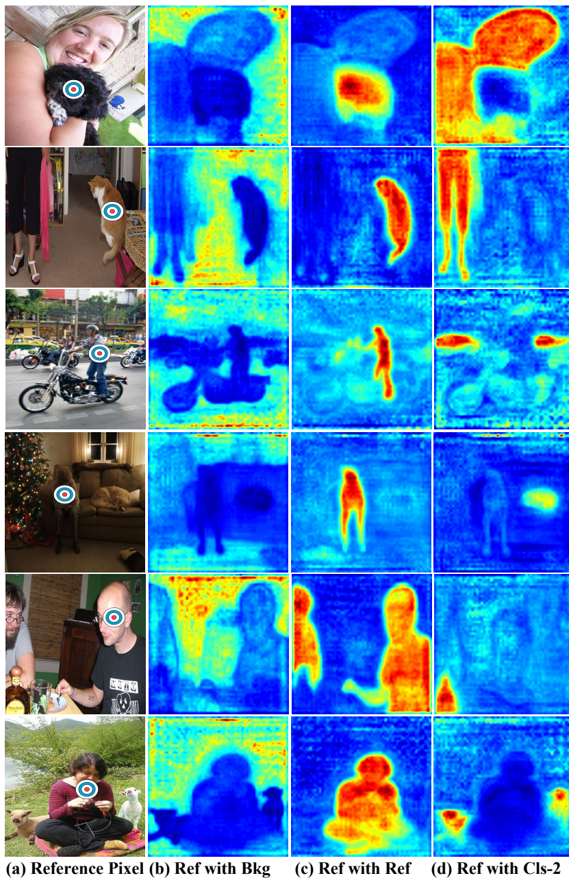
Figure 3.4: Visualization of pairwise terms obtained by our G-CRF embeddings trained for the semantic segmentation task. Column (a) shows the reference pixel ( p^* ), marked with a dartboard, on the image. The pairwise term corresponding to p^* taking the ground truth label l^* and any other pixel p taking the label l is given by the inner product A_{p^*,p}(l^*, l) = \langle \mathcal{A}_p^l, \mathcal{A}_{p^*}^{l^*} \rangle . We show the pairwise terms A_{p^*,p}(l^*, bkg) in (b), A_{p^*,p}(l^*, l^*) in (c), and A_{p^*,p}(l^*, l_2) in (d), where l_2 is the most dominant class in the image besides l^* .
