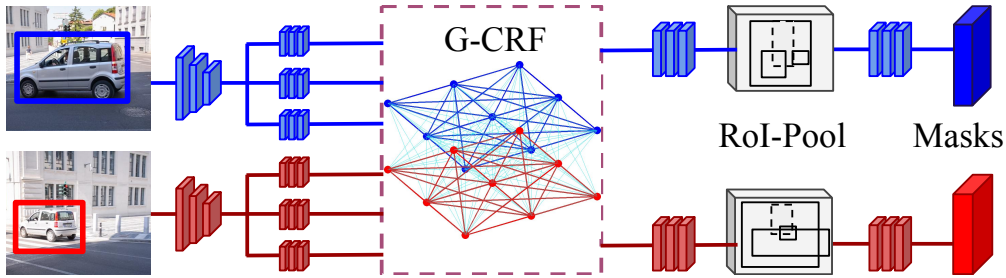
Figure 4.5: Spatio-temporal structured prediction in Mask-RCNN. Here we use CRFs in the feature learning stage before the ROI-Pooling (and not as the final classifier). This helps learn mid-level features which are better aware of the spatio-temporal context.
