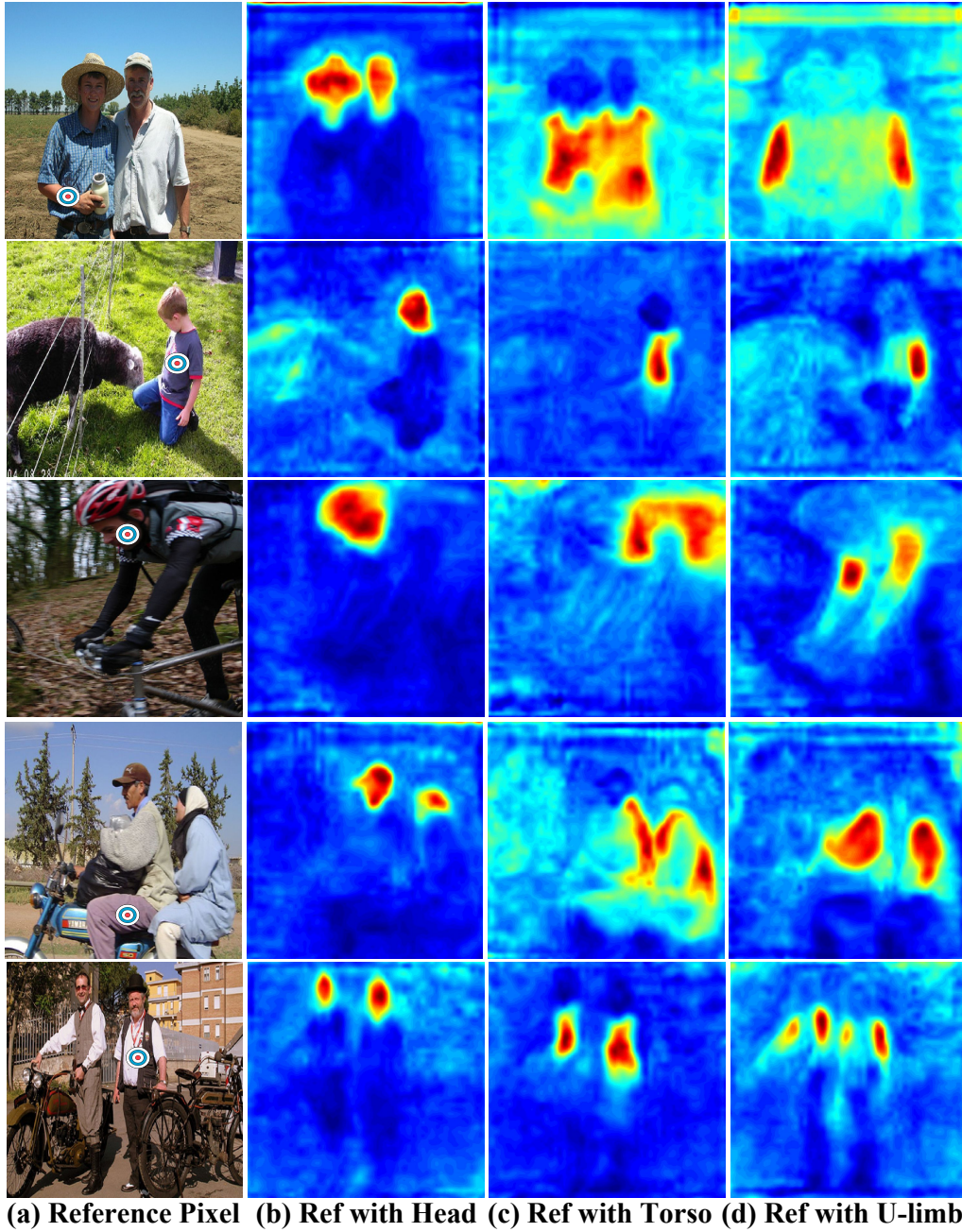
Figure 3.3: Visualization of pairwise terms obtained by our G-CRF embeddings trained for the human part segmentation. Column (a) shows the reference pixel ( p^* ), marked with a dartboard, on the image. The pairwise term corresponding to p^* taking the ground truth label l^* and any other pixel p taking the label l is given by the inner product A_{p^*,p}(l^*,l) = \langle \mathcal{A}_p^l, \mathcal{A}_{p^*}^{l^*} \rangle . We show the pairwise terms A_{p^*,p}(l^*, head) in (b), A_{p^*,p}(l^*, torso) in (c), and A_{p^*,p}(l^*, upper-limb) in (d).
