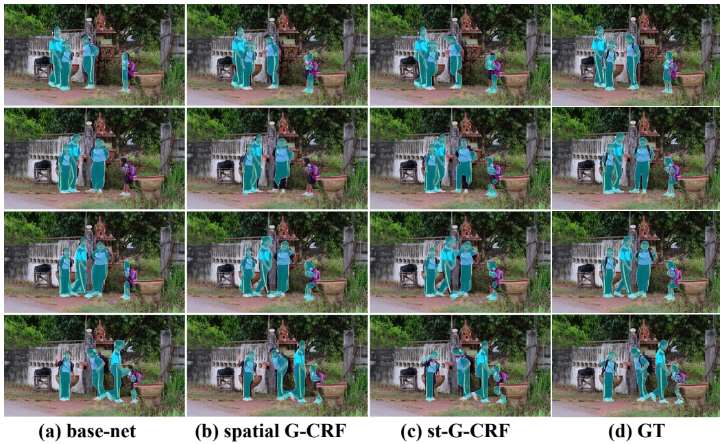
Figure 4.8: Qualitative results for instance segmentation on the DAVIS Person Dataset. We notice that the base-net and the spatial G-CRF in (a),(b) miss the school-girl on the right in the second frame. Temporal context from spatio-temporal G-CRFs in (c) helps recover her.
