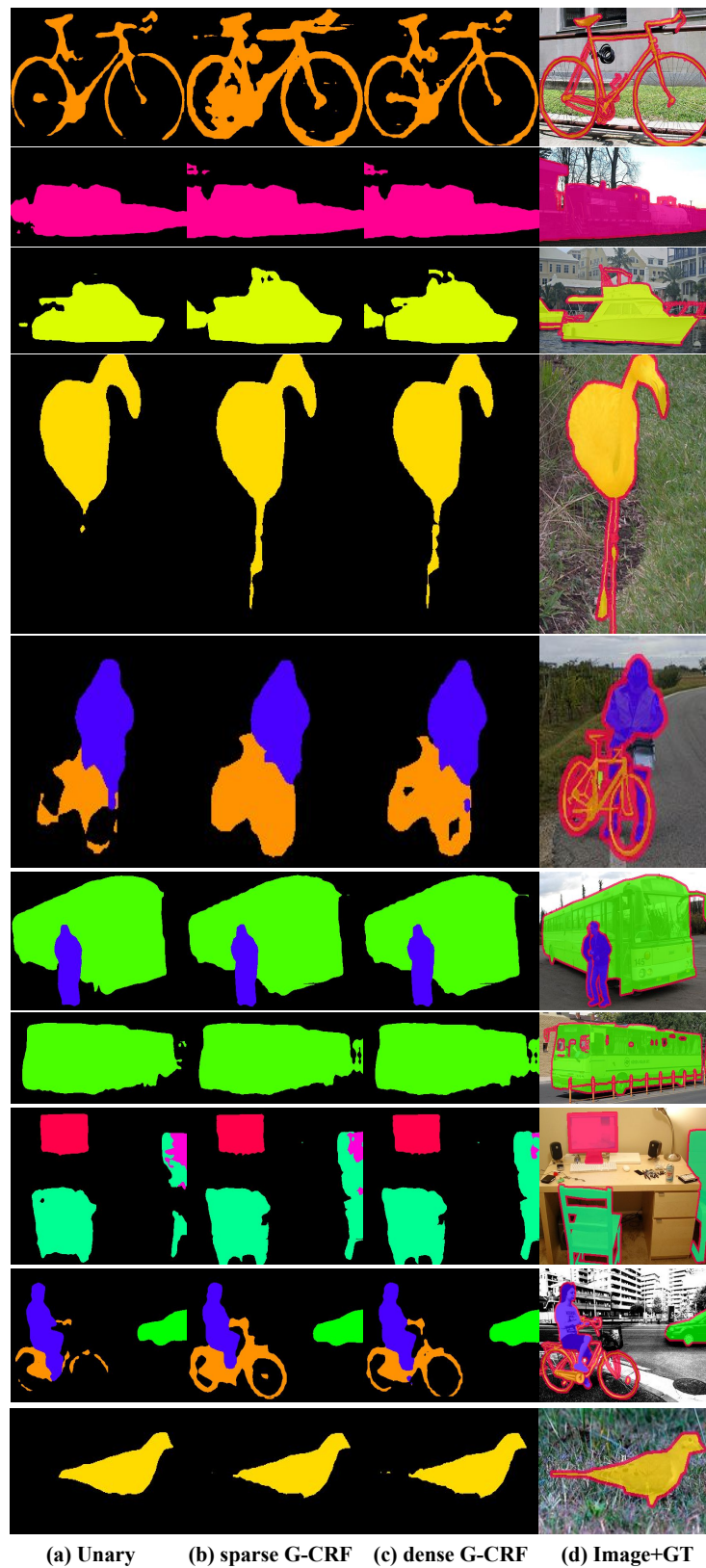
Figure 3.7: Qualitative Results of Semantic Segmentation. (a) shows the unary network output, (b) shows the sparsepotts-G-CRF output, (c) shows the densepotts-G-CRF output, and (d) shows the input image and ground truth.
