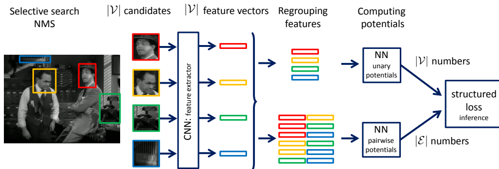
Figure 1.13: Context-aware CNNs for person head detection [Vu 2015]: Schematic visualization of the end-to-end trainable CRFs for object detection. The authors use QPBO and TRW-S for approximate CRF inference.
