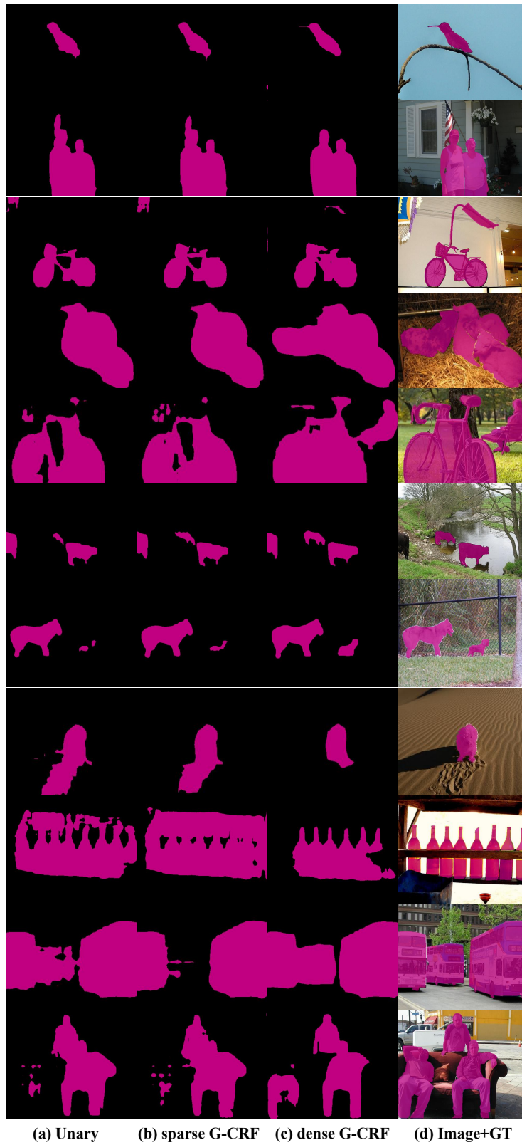
Figure 3.9: Qualitative Results of Saliency Estimation. (a) shows the unary network output, (b) shows the sparsepotts-G-CRF output, (c) shows the densepotts-G-CRF output, and (d) shows the input image and ground truth.
