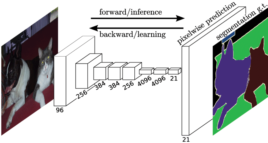
Figure 1.4: Fully Convolutional Networks (FCNs): FCNs were used in [Long 2015] for semantic segmentation. FCNs are CNNs that do not use any fully connected layers (in contrast with Fig. 1.3). This allows them to produce outputs that spatially correspond to patches in the input image.
