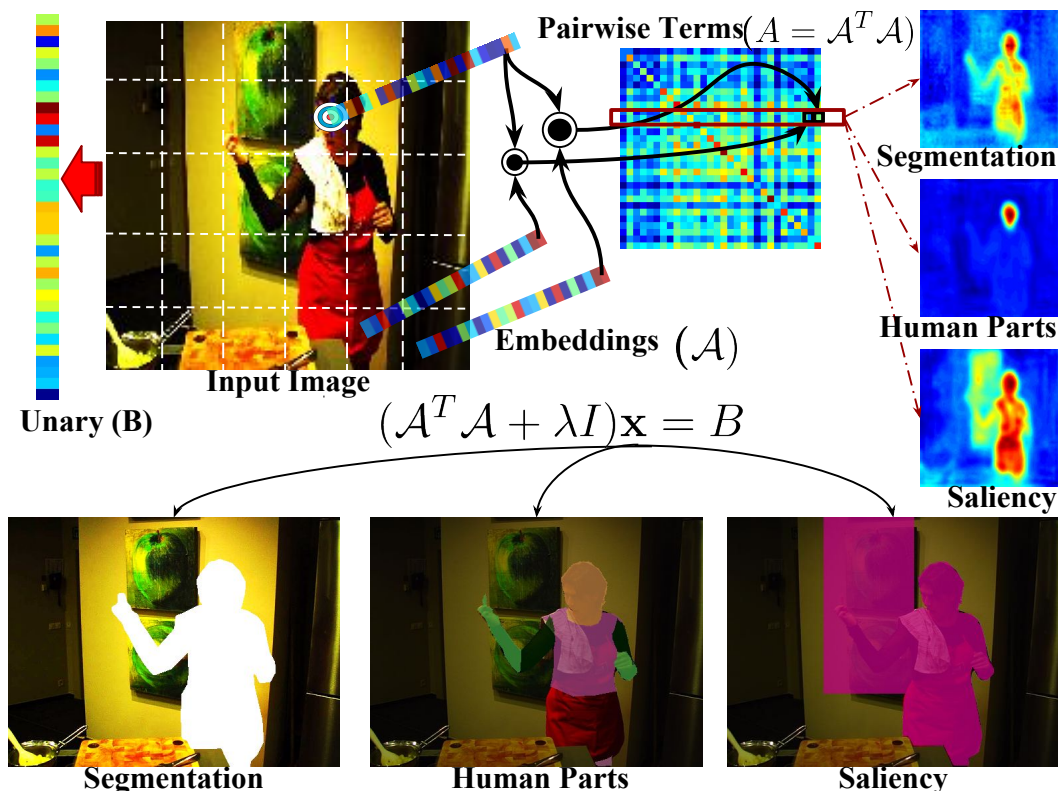
Figure 3.1: Method overview: each image patch amounts to a node in our fully-connected graph structure. As in the G-CRF model, we infer the prediction \mathbf{x} by solving a system of linear equations A\mathbf{x} = B , based on CNN-based unary ( B ) and pairwise ( A ) terms. We express pairwise terms as dot products of low-dimensional embeddings ( A_{i,j} = \langle \mathcal{A}_i, \mathcal{A}_j \rangle ), delivered by a devoted sub-network. This ensures that A is low-rank, allowing for efficient, conjugate gradient-based solutions. The embeddings are optimized in a task-specific manner through end-to-end training.
