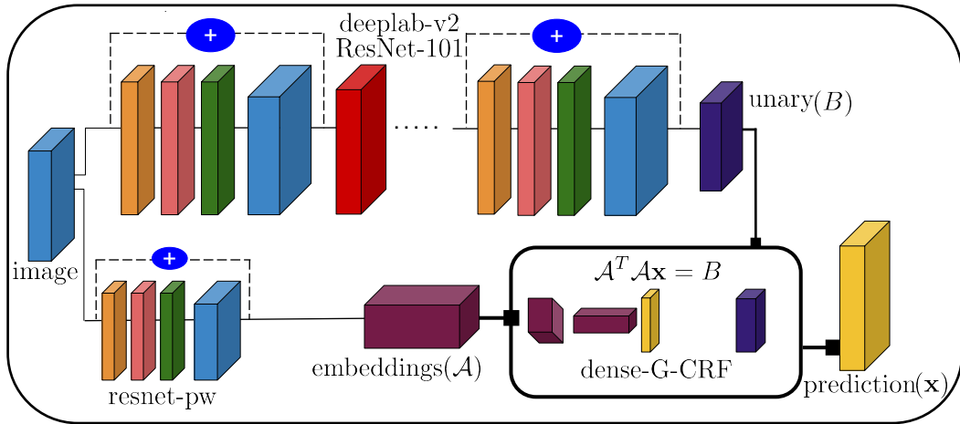
Figure 3.2: Illustration of our end-to-end trainable, fully convolutional network employing a dense-G-CRF module. We get our unary terms from Deeplab-v2 (we only show one of its three ResNet-101 branches, for simplicity). Our pairwise (pw) terms are generated by a parallel sub-network, resnet-pw, which outputs the pixel embeddings of our formulation. The unary terms and pairwise embeddings are combined by our fully connected G-CRF module (dense-G-CRF). This outputs the prediction \mathbf{x} by solving the linear system \mathcal{A}^T \mathcal{A} \mathbf{x} = B .
