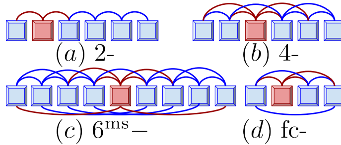
Figure 4.4: Illustration of the various temporal neighbourhoods we consider in our ablation study. Each box denotes a video frame and the arcs connecting them are pairwise connections. We show a frame in red with all neighbours present in the temporal context.
