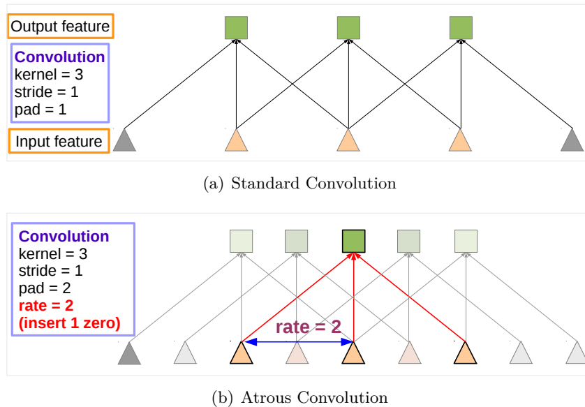
Figure 1.5: Comparison of standard convolution with atrous convolution [Chen 2014a] on a 1-D feature image. (a) shows the standard convolution with a 3 \times 1 kernel where the input features (yellow triangles) are padded by 1 pixel (gray triangles) on either side to obtain an output feature map (outputs shown as green squares) of the same size. (b) shows the atrous convolution with a 3 \times 1 kernel with a dilation rate of 2 where the input features are padded by 2 pixels on either side. The rate parameter denotes the stride with which the input features are sampled, and allows ‘holes’ in the convolution kernel. This allows computing an output feature map with the same size as the input feature map without increasing the number of convolution parameters. Further, atrous convolutions can be viewed as dilated convolutions since holes in the convolution kernel expand the field of view of the filter allowing a larger context to be captured.
