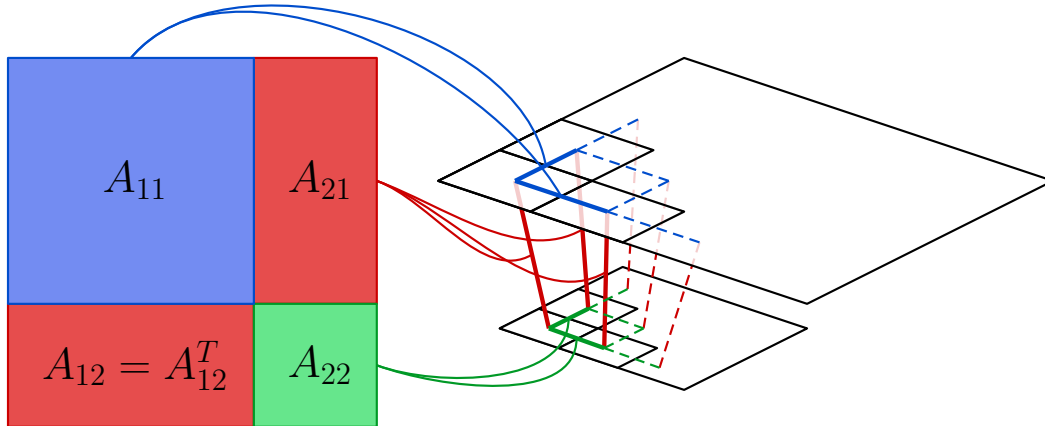
Figure 2.4: Schematic diagram of matrix A for the multi-resolution formulation in Sec. 2.4.2. In this example, we have the input image at 2 resolutions. The pairwise matrix A contains two kinds of pairwise interactions: (a) neighbourhood interactions between pixels at the same resolution (these interactions are shown as the blue and green squares), and (b) interactions between the same image region at two resolutions (these interactions are shown as red rectangles). While interactions of type (a) encourage the pixels in a neighbourhood to take the same or different label, the interactions of type (b) encourage the same image region to take the same labels at different resolutions.
