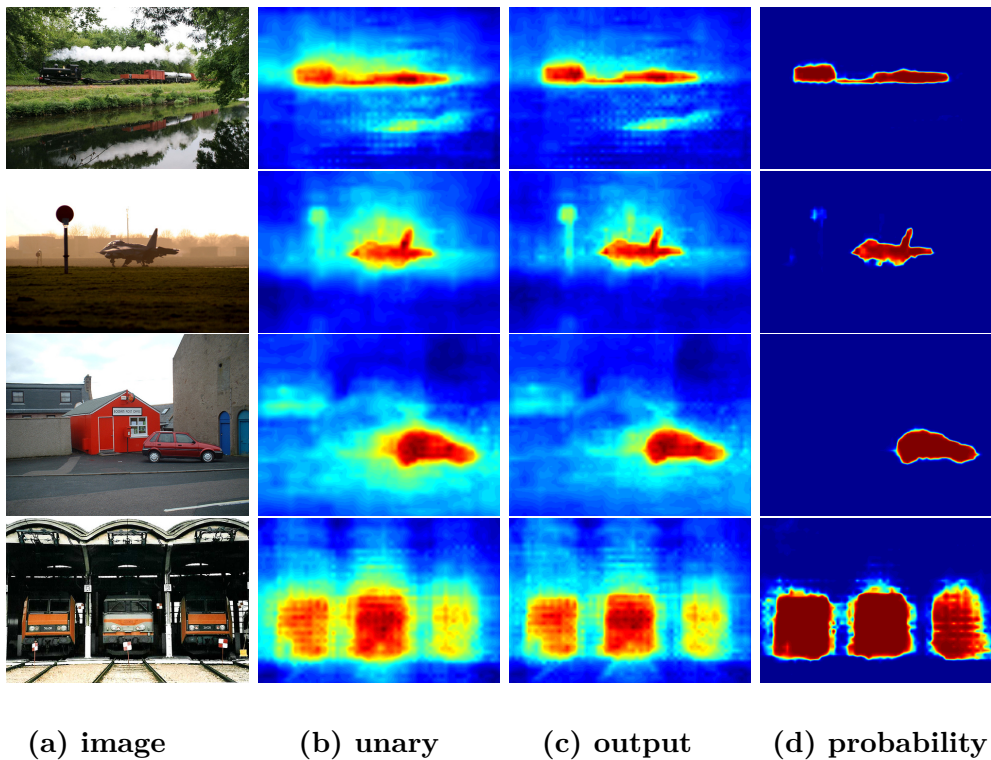
Figure 2.5: Qualitative results when our Potts type pairwise terms are used in combination with the deeplab-V2 Resnet-101 network. Column (a) shows the input image, (b) shows the heatmap of the unary scores, (c) shows the heatmap of the scores after inference, and (d) shows the softmax probabilities. We notice that the object boundaries are significantly finer after incorporating cues from the pairwise terms.
