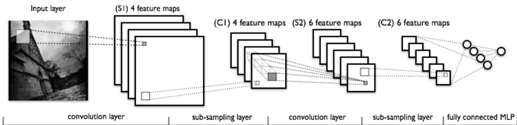
Figure 1.3: Convolutional Neural Network: A schematic representation of the LeNet-5 CNN from [Lecun 1998], showing the common deep learning modules, namely convolution and sub-sampling. The convolutional backbone of the network performs local, patch-based feature extraction. This network also employs fully-connected layers to obtain a global image-representation from these local features.
