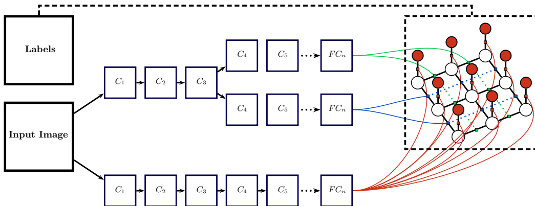
Figure 2.1: Schematic of a fully convolutional neural network with a G-CRF module: we show a detailed schematic representation of our fully convolutional neural network with a G-CRF module. The G-CRF module is shown as the box outlined by dotted lines. The factor graph inside the G-CRF module shows a 4-connected neighbourhood. The white blobs represent pixels, red blobs represent unary factors, the green and blue squares represent vertical and horizontal connectivity factors. The input image is shown in (b). The network populates the unary terms (c), and horizontal and vertical pairwise terms. The G-CRF module collects the unary and pairwise terms from the network and proposes an image hypothesis, i.e. scores (d) after inference. These scores are finally converted to probabilities using the Softmax function (e), which are then thresholded to obtain the segmentation.
