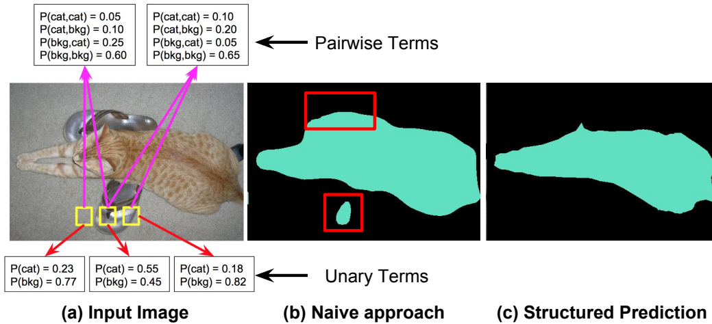
Figure 1.8: Naive approach vs Structured Prediction: The input image is shown in (a). We also show the unary terms for some patches, and pairwise terms computed for pairs of patches. The unary terms consist of two scores per patch. These two scores indicate the model’s confidence in the patch belonging to ‘cat’ and ‘background’ categories when the patch is viewed in isolation. The pairwise terms are computed by looking at two patches at a time. These consist of four scores, one for each combination of classes which can be assigned to the two patches. In (b) we show the output of Deeplab Large-FOV network [Chen 2014a] on the input image, obtained by using the unary terms alone. We mark the false ‘cat’ predictions using red boxes. The image in (c) shows the output of our method which uses structured prediction and uses both the unary and pairwise terms to make a decision about the label taken by each patch: the model is able to eliminate isolated patches of false predictions and better capture object boundaries by capturing interdependencies between the two labels.
