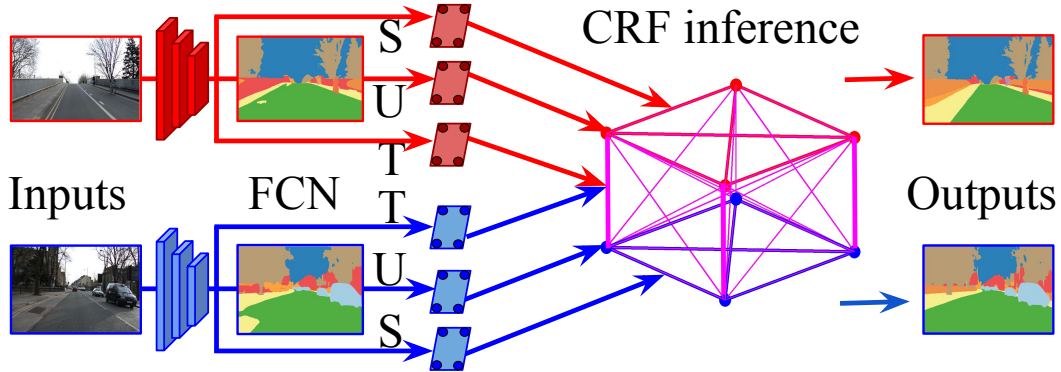
Figure 4.1: Overview of our VideoGCRF approach: we jointly segment multiple images by passing them firstly through a fully convolutional network to obtain per-pixel class scores (‘unary’ terms U), alongside with spatial (S) and temporal (T) embeddings. We couple predictions at different spatial and temporal positions in terms of the inner product of their respective embeddings, shown here as arrows pointing to a graph edge. The final prediction is obtained by solving a linear system; this can eliminate spurious responses, e.g. on the left pavement, by diffusing the per-pixel node scores over the whole spatio-temporal graph. The CRF and CNN architecture is jointly trained end-to-end, while CRF inference is exact and particularly efficient.
