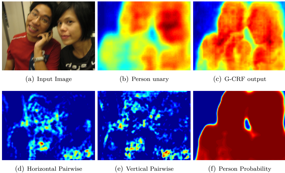
Figure 2.2: G-CRF Inference: This figure compares the unary terms with the G-CRF prediction for semantic segmentation. It can be seen that the unary scores in (b) miss part of the torso because it is occluded behind the hand. The flow of information from the neighbouring region in the image, via the pairwise terms, encourages pixels in the occluded region to take the same label as the rest of the torso (c). It can also be seen that the person boundaries are more pronounced in the output (c) due to pairwise constraints between pixels corresponding to the person and background classes. We also show heatmaps of the horizontal and vertical pairwise terms learnt by our network in (d) and (e). These heatmaps show spikes in image regions where the model thinks that the horizontally and vertically adjacent pixels are likely to belong to different classes. Finally, we show the posterior probability of the person class in (f).
