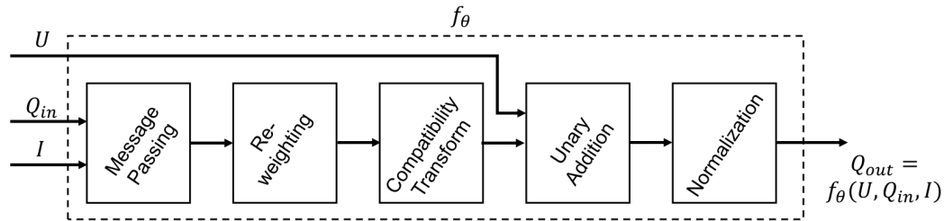
Figure 1.12: CRF-as-RNN: The authors of [Zheng 2015] reformulate a single mean-field iteration as a stack of common CNN modules. With this rephrasing, approximate CRF inference can be achieved with an RNN, allowing end-to-end learning via back-propagation.
