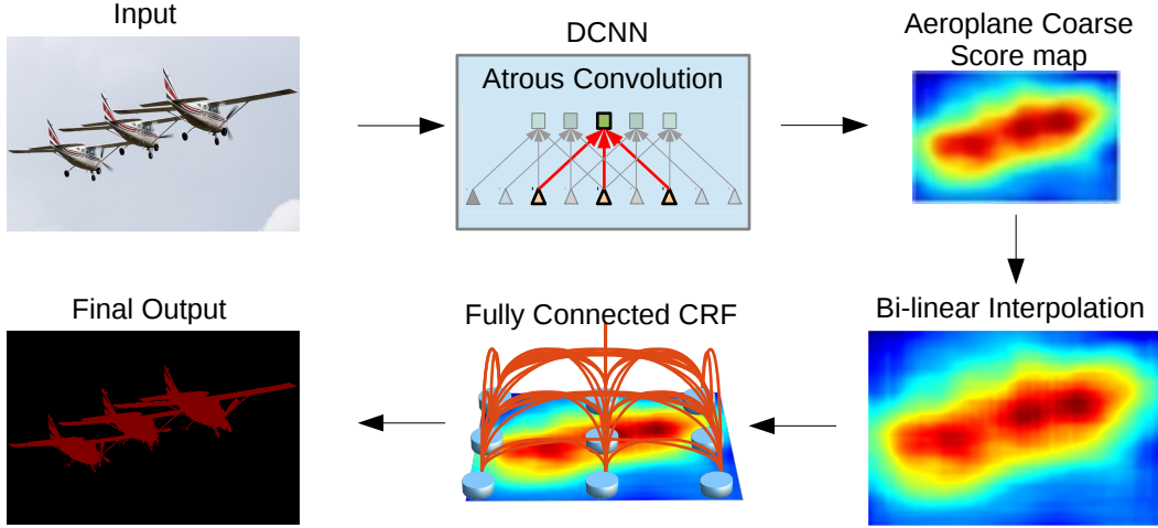
Figure 1.11: Illustration of the Deeplab [Chen 2014a] pipeline: The CNN generates unary scores, and these are upsampled to the original resolution via bilinear interpolation. These unary scores are fed to a fully-connected CRF alongside hand-crafted pairwise terms. The Dense-CRF algorithm is used as a post-processing step to obtain a sharper segmentation map which better captures finer details in the image.
