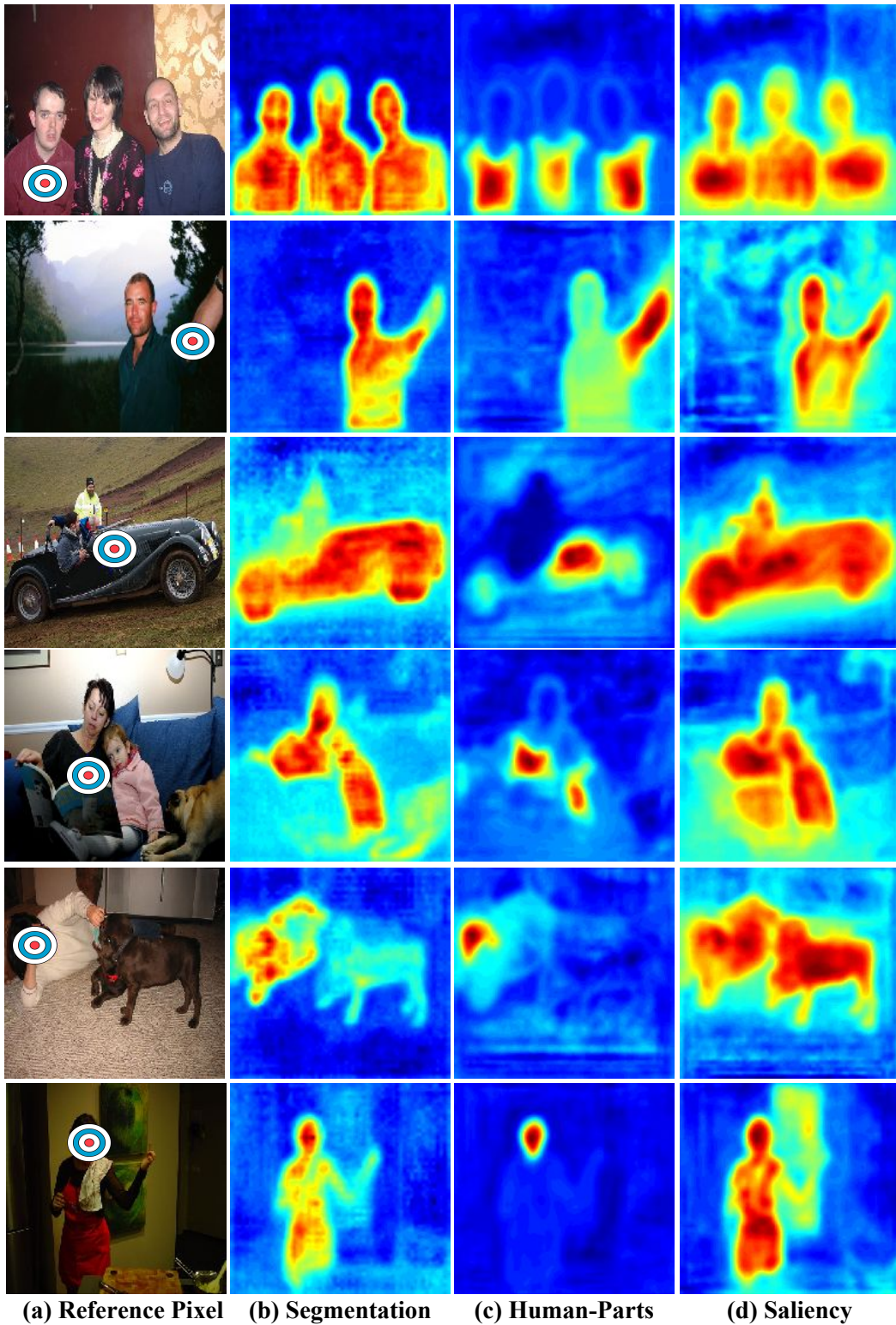
Figure 3.6: Visualization of pairwise terms obtained by our Potts-Type task-specific G-CRF embeddings. The first column shows the reference pixel ( p^* ), marked with a dartboard, on the image. The pairwise term between p^* and any other pixel p is given by the dot product A_{p^*,p} = \mathcal{A}_p^T \mathcal{A}_{p^*} . We show the pairwise terms A_{p^*,p} for the (b) segmentation task, (c) human part estimation, (d) and saliency estimation.
