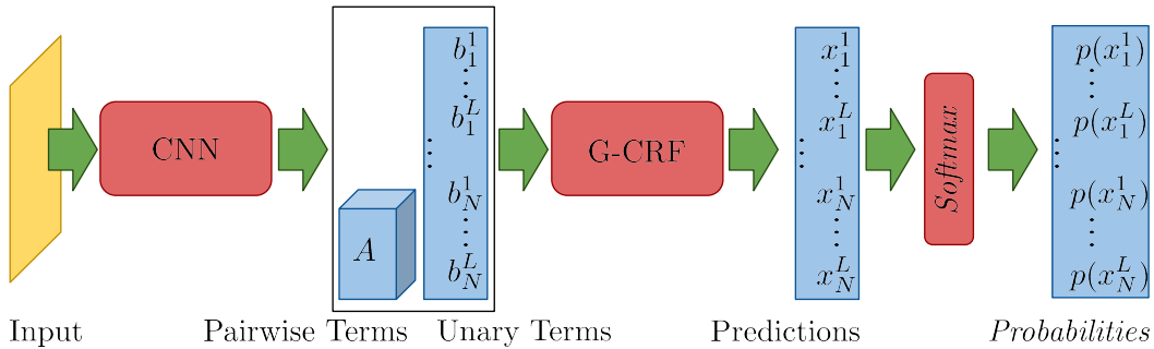
Figure 1.10: G-CRFs for discrete labeling tasks: The G-CRF module receives unary and pairwise terms ( A ) from a CNN. b_i^u denotes the unary score for pixel i taking the label u . The G-CRF module performs structured prediction and outputs the predictions: x_i^u denotes the prediction score for pixel i taking the label u . These predictions are fed as input to a Softmax module which converts these predictions to probabilities: p(x_i^u) denotes the probability of pixel i taking the label u .
