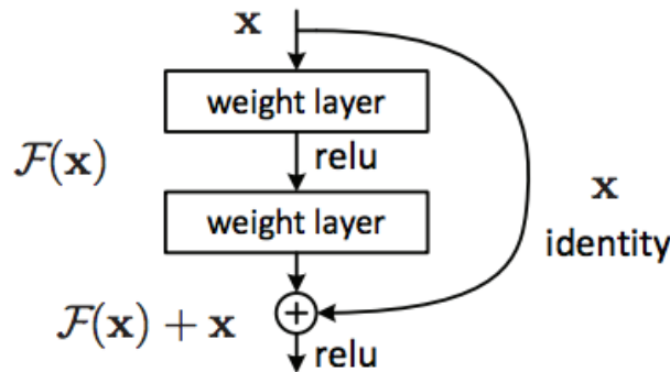
Figure 1.6: A residual block: fundamental unit of a residual network [He 2016]. In parallel to a stack of layers that perform non-linear mapping of the input data, the residual block contains a shortcut connection of identity mapping without adding any extra parameter or computational complexity. In simpler terms, a residual block recasts the original mapping as F(x) + x . It is hypothesized that optimizing the residual mapping is easier than optimizing the original, unreferenced mapping.
