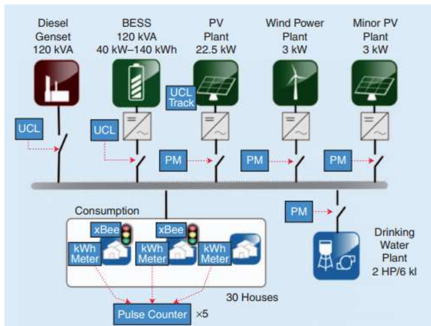
Fig. 2.26. Microgrid diagram [65]
