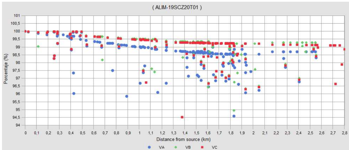
Fig. 4.42. Voltage Profile
