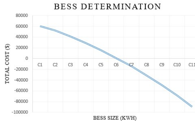
Fig. 4.22 Total Cost for different batteries’ sizes considering different TOU for batteries.
