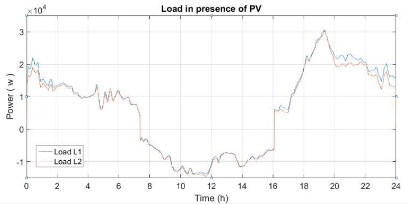
Fig. 4.20 Load in each phase in the presence of PV generation.
