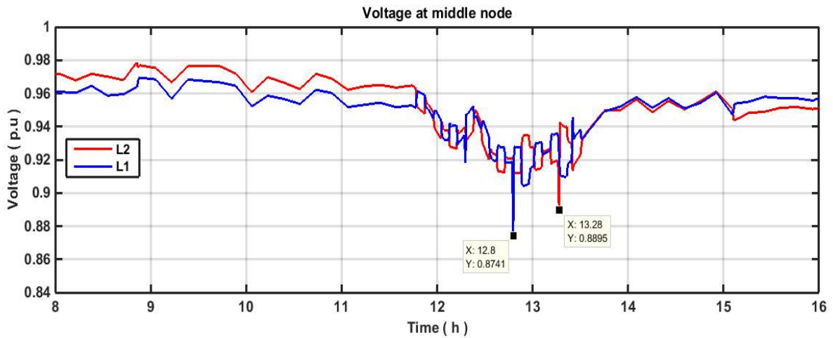
Fig. 4.35. Lowest voltages during the switching
