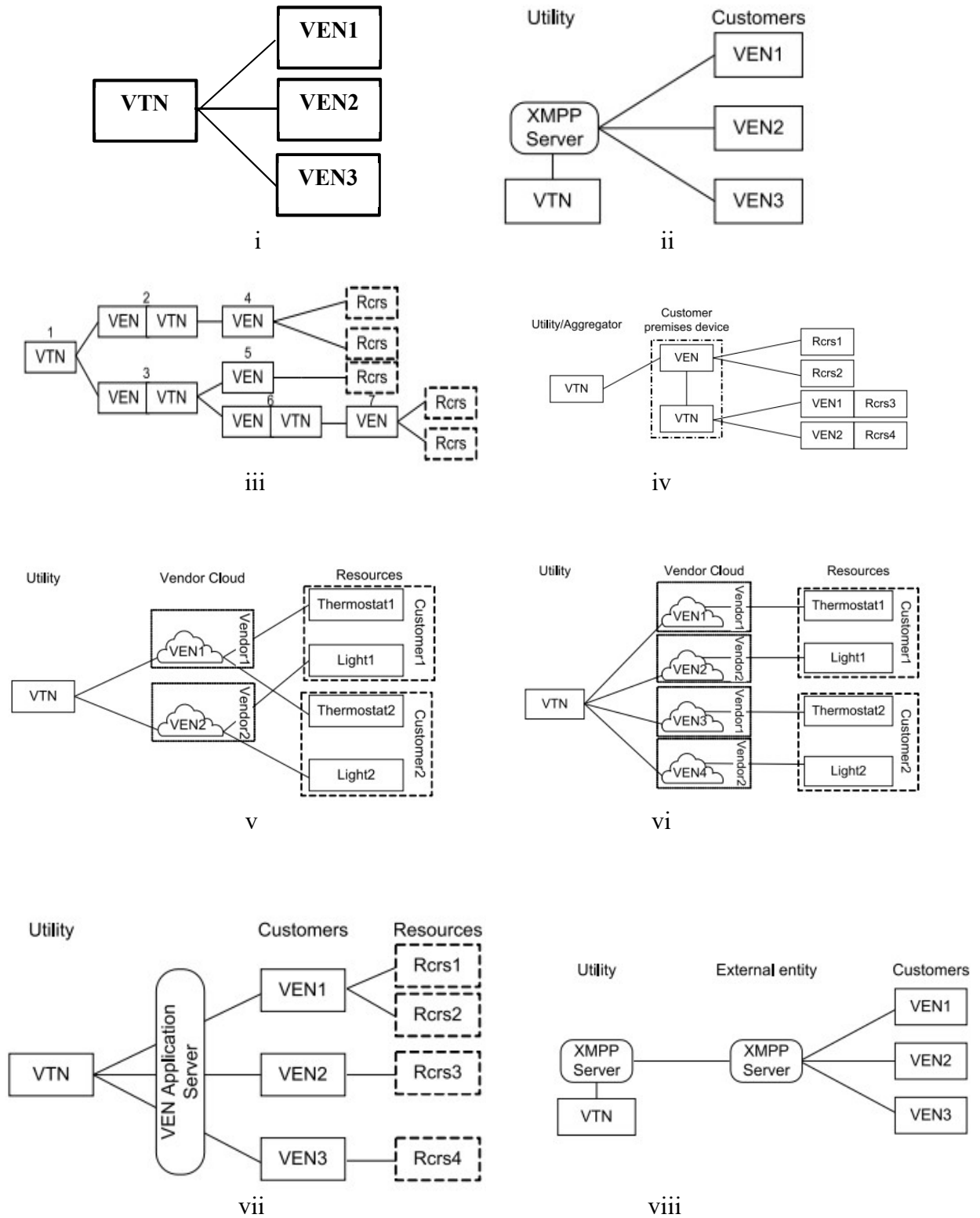
Fig. 6.14. OpenADR architectures
