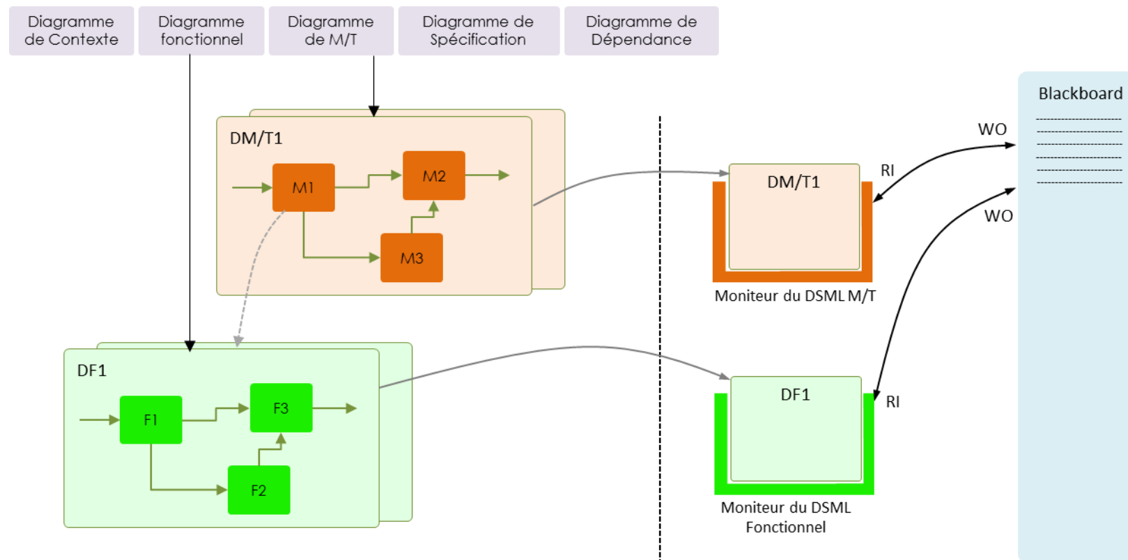
Figure 35: Illustration DSML / Moniteur / Blackboard
