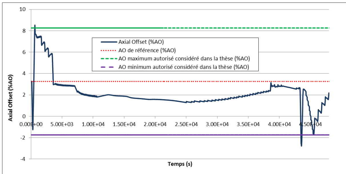
Figure 152: Simulation Mode T – Axial Offset - Rampe 100-60-100%PN à 5%/min
