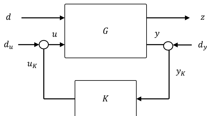
Figure 122: Marge de robustesse MIMO
