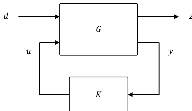
Figure 12: Forme standard de commande
