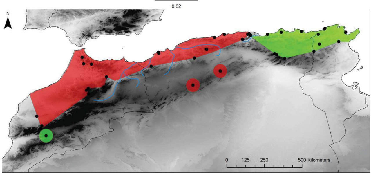
Fig 7. Bayesian inference Phylogenetic trees and posterior probabilities of relevant nodes and the map of the repartition of the eastern (green) and western (red) clades of Podarcis vaucheri .
