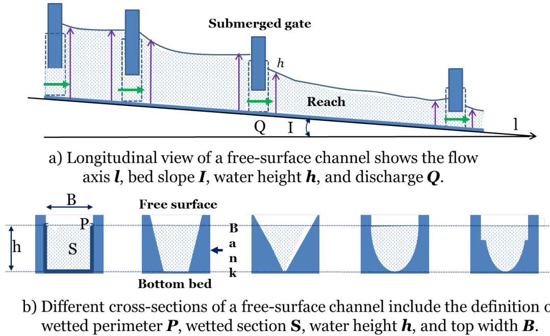
Fig. 1.1 The common parameters and variables are used to characterize a free-surface channel.
