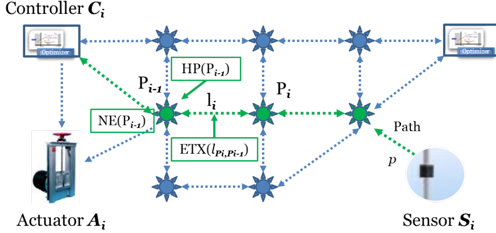
Fig. 2.4 An example of the data communication from level sensor S_i to controller C_i in the hybrid network: a path p(S_i, \dots, P_i, \dots, P_1, C_i) is taken as an example. For a node P_i on the path p , the path cost from P_i to C_i is calculated by: c(P_i, C_i) = c(P_i, P_{i-1}) + c(P_{i-1}, C_i) .
