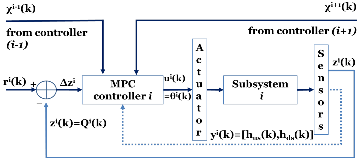
Fig. 4.3 Variables are involved in the flow rate control of a reach using the MPC method.
