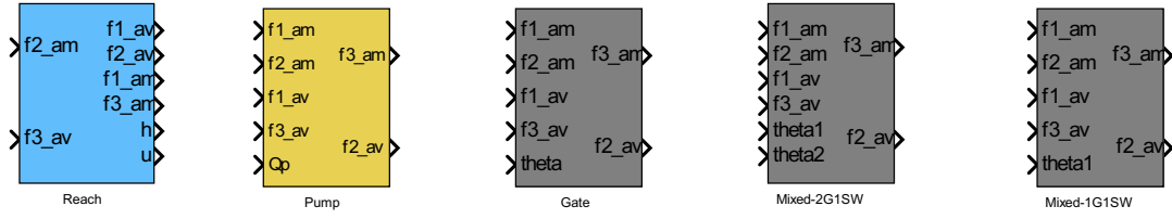
Fig. 1.7 A Simulink/MatLab Model Library is created for the modeling and the simulation of an irrigation channel.
