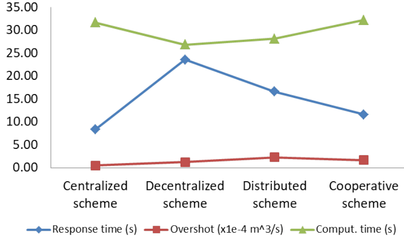
Fig. 4.6 Performance comparison of four MPC settings: centralized, decentralized, distributed and distributed cooperative control.
