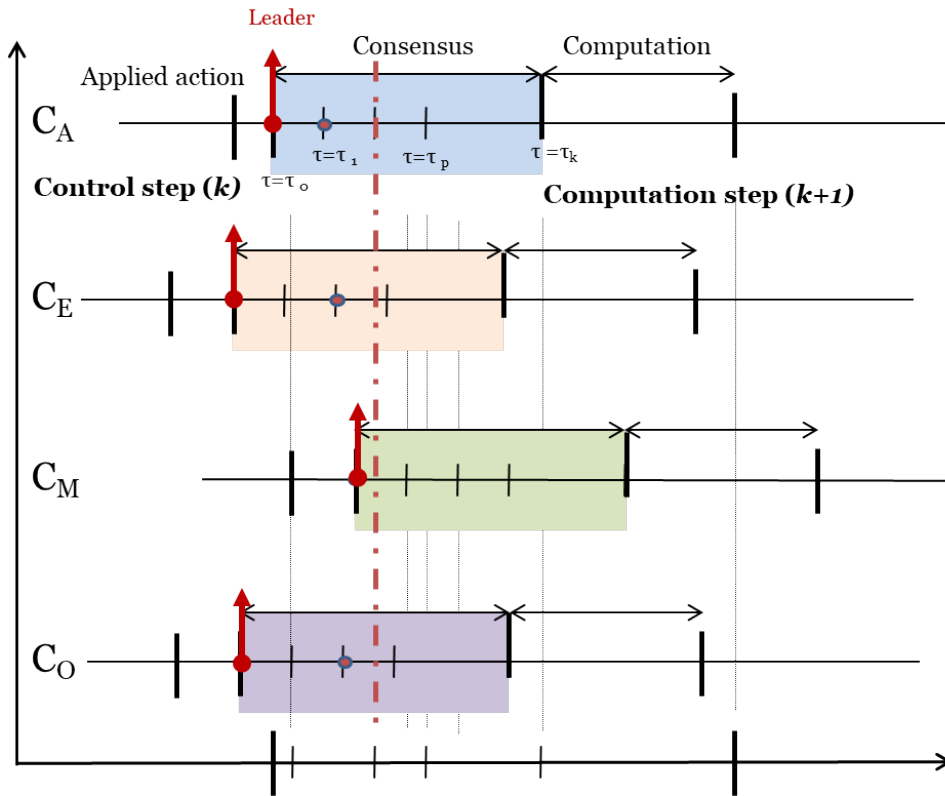
Fig. 4.5 Asynchronous framework for consensus problem in distributed control of irrigation channels. Four controllers C_A, C_E, C_M, C_O are involved in DCMPC scheme. After applying the computed optimal action to the subsystem, the corresponding controller becomes the actual leader and starts a consensus process.
