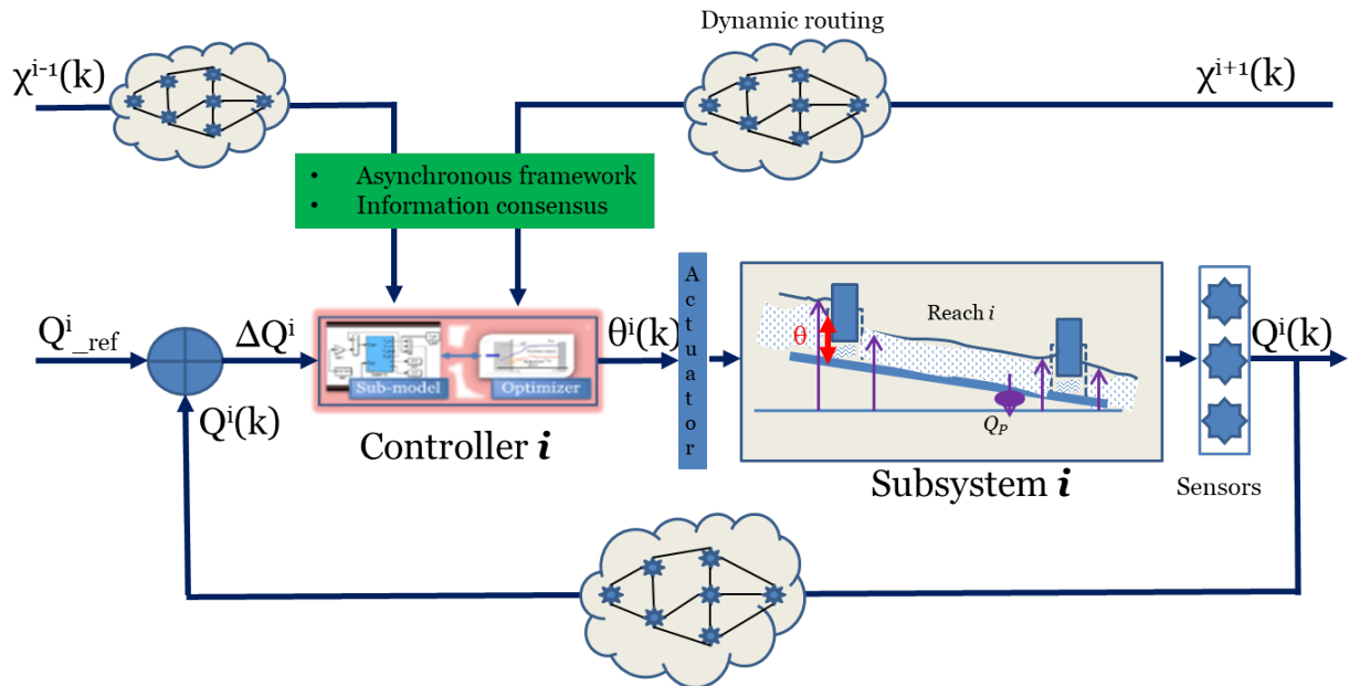
Fig. 3.5 Approach to the problem of divergent information shared among controllers by an information consensus problem. This problem is then solved by an asynchronous consensus protocol designed to achieve the convergence of information states of controllers.
