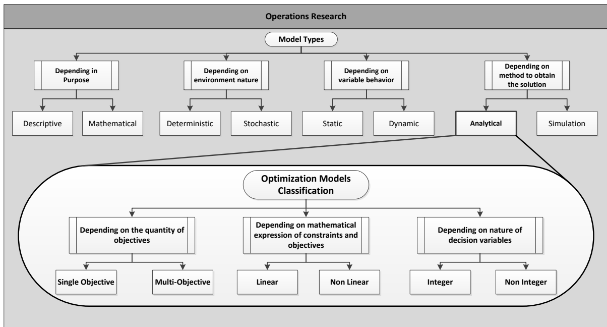
Figure 3. 2. Optimization model classification resumed.
