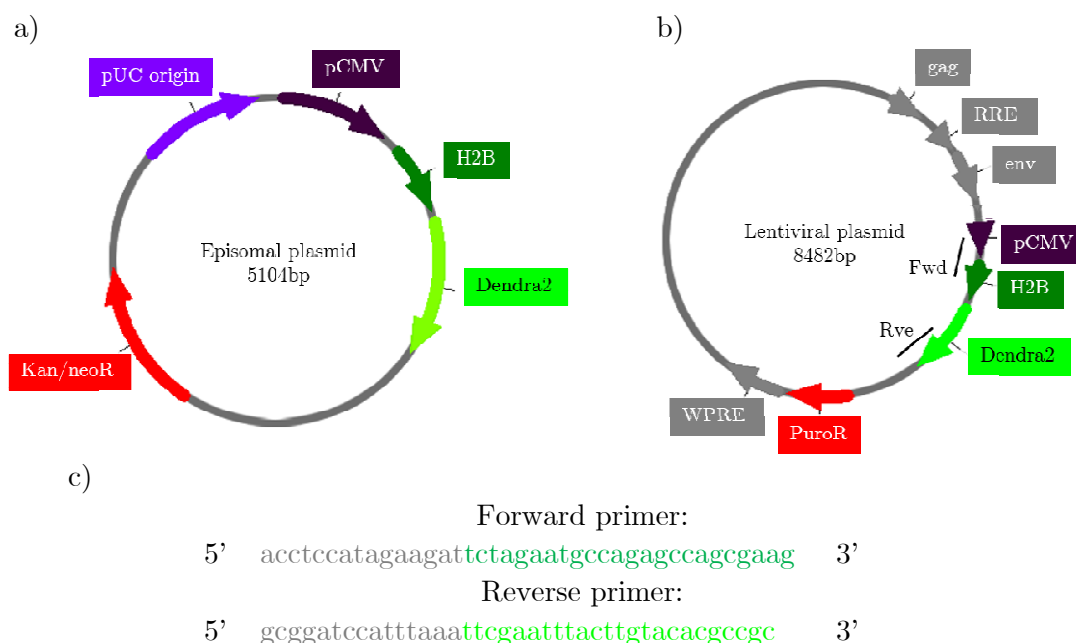
Figure 5.1 Episomal and lentiviral plasmids used for the establishment of H2B Dendra2 stable cell lines
