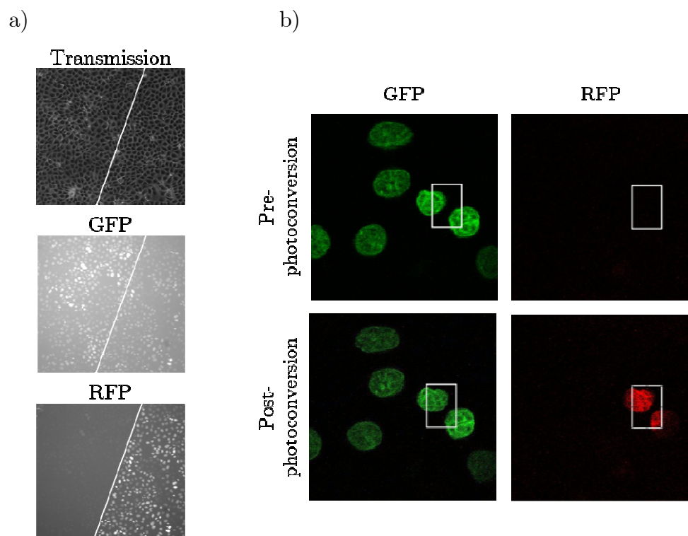
Figure 7.8 H2B Dendra2 green-to-red photoconversion in MDCK cells
