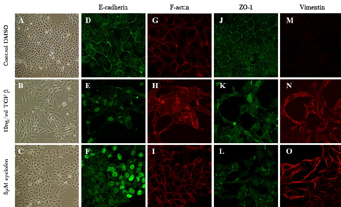
Figure 7.7 EMT induction in MDCK-SnailERT2 H2B Dendra2 cells
