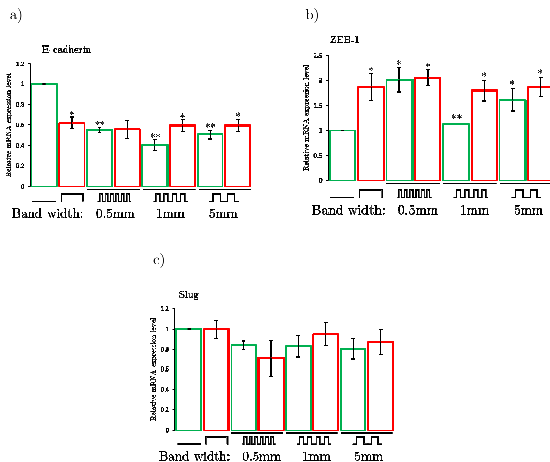
Figure 8.3 mRNA expression levels of EMT markers following band patterned distribution of EMT
