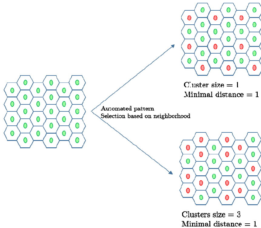
Figure 7.15 Automated generation of neighborhood patterns
