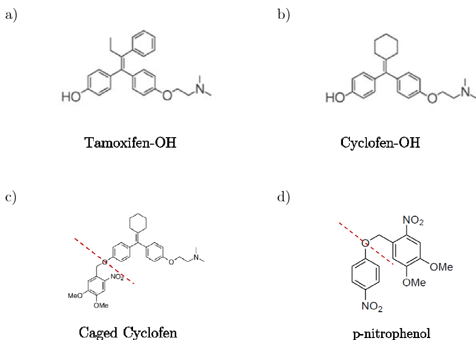
Figure 7.1 Chemical Structure of ERT2 ligands
