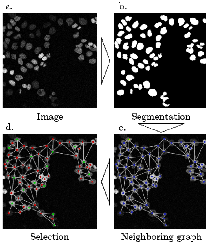
Figure 7.16 Generation of patterns for phenotypic induction
