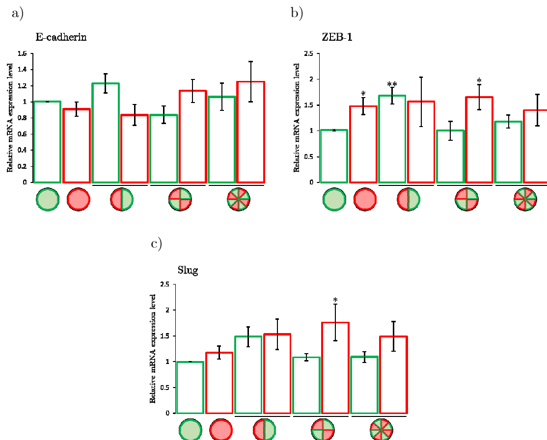
Figure 8.1 mRNA expression levels of EMT markers following radial distribution of EMT
