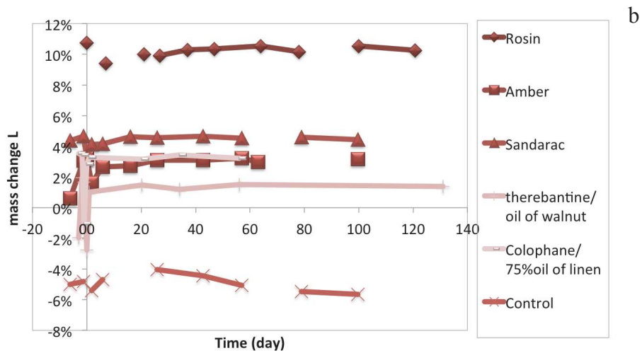
Fig. C.12 Variation of mass in R (a) and L (b) direction.
