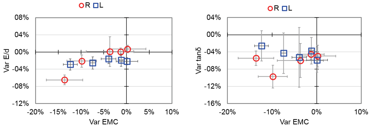
(a) (b) Fig. B.5. Correlation between variations of E'/d vs EMC (a), and \tan \delta vs EMC (b).
