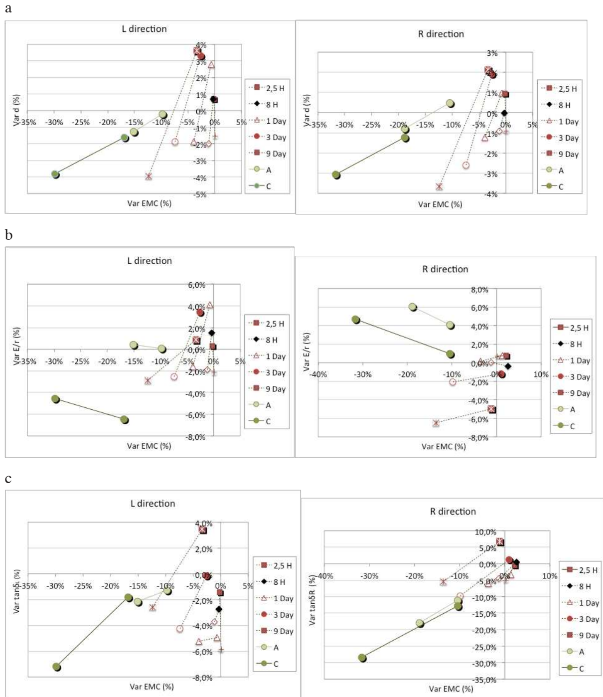
Fig. B.17 Relations between the (relative) variations in EMC and those of others properties, after thermal treatment and then after reconditioning: (a) density (b) specific modulus of elasticity (c) damping. Empty symbols correspond to values after thermal treatment; filled symbols correspond to values after reconditioning.
