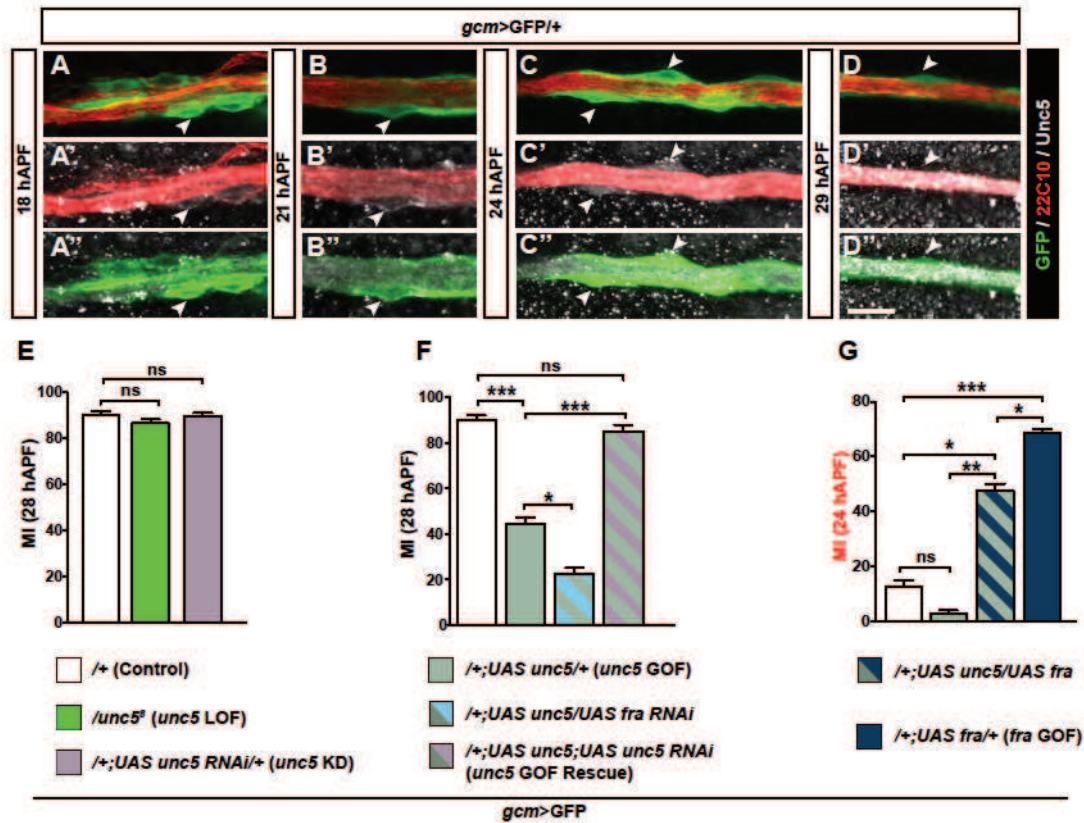
Figure 7: Unc5 acts as a repellant in glia migration. (A-D'') Wing immunolabelled with anti-22c10 (neurons, red), anti-Unc5 (grey) and anti-GFP (glial cells, green) in the transgenic line gcm>GFP/+ at different migratory stages. Unc5 transiently starts to express both in glia and neurons at around 18 hAPF and fades away by 29 hAPF. (E-G) Graphs represent the MI of the indicated genotypes. Scale bars: (A-D''), 10 \mu m.
