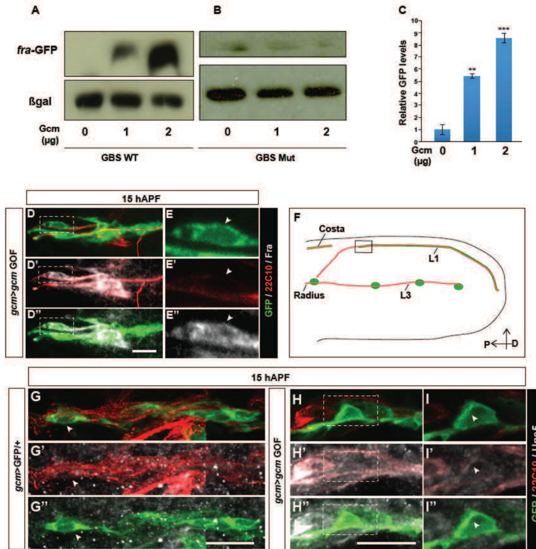
Supplementary Figure 5: Western blot and gcm GOF analysis confirms fra is a direct Gcm target and early Unc5 expression. (A) Immunoblot analysis of a WT Fra plasmid containing the GBS's monitored for an increase in the level of GFP (representative Western Blot out of a sample of 3). An increasing GFP level suggests that Fra is a direct target of Gcm . WB on total protein extracts from transfected S2 cells using anti GFP for Fra detection (top part) and anti \beta gal (lower part). No antibody was used for the detection of Gcm because of the use of WT Gcm plasmid. LacZ was used as a loading control. (B) Same WB was performed using a mutated Fra plasmid; detection of no GFP level upon using the gradients of Gcm confirms our analysis of Fra being a direct target of Gcm . (C) Quantification of the Western blot, Y-axis indicates the relative GFP levels of Fra upon S2 cells co-transfection assay. X-axis indicates the used gradients of Gcm in ( \mu g). (D-E'') Expression profile of Fra in gcm GOF animals at 15 hAPF. Note that the blown up region in panels (E-E'') is highlighted by a dashed white bracket in (D-D''). See the enhanced protein levels in panels (D-E'') as compared to the panels in
