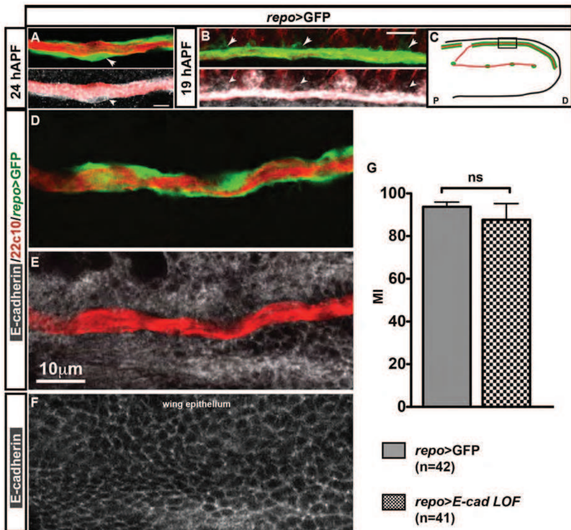
Figure S1: N- and E-cadherin expression profiles
