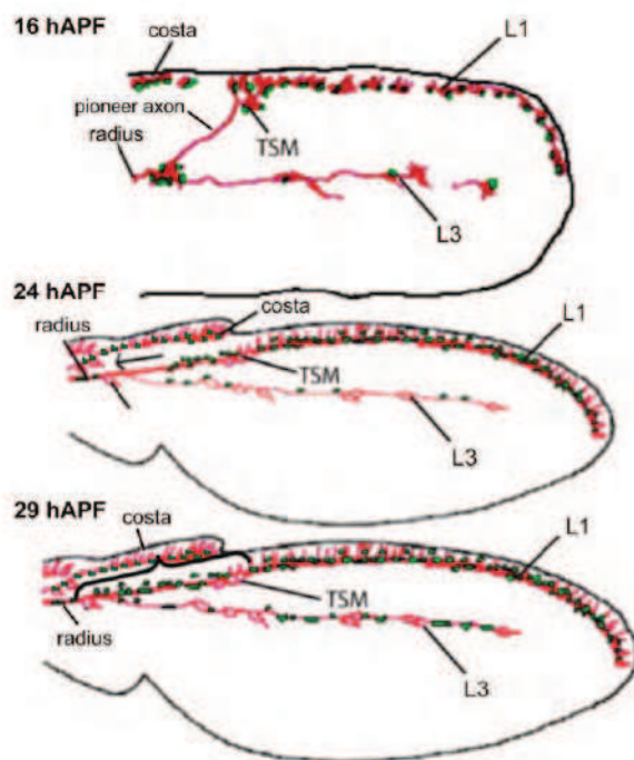
Figure 14: Glial cell migration. Schematic representation of the developing Drosophila wing. Glia is in green and neurons are in red, TSM: Twin sensilla of the Margin. Glia do not move at 16 hAPF and are closely located to their place of birth, however, L1 and L3 neurons have already form a continuous nerve. By 24 hAPF glia has already moved along both L1 and L3 nerves. Glia completes migration by 28-29 hAPF
