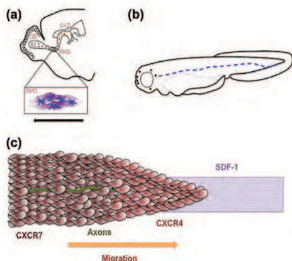
Figure 1. Collective cell migration in vertebrates. (a) In the rostral migratory stream (RMS), neuroblasts (purple) born in the adult subventricular zone (SVZ) migrate towards the olfactory bulb (OB), forming a chain that is flanked by astrocytes (blue) serving as a tunnel for the collective (shown in the inset) (modified from Woong et al., 2010). (b) The zebrafish posterior lateral line system. In a 2-day-old embryo, the neuromasts of the posterior lateral line (PLL) (large black dots) are deposited by a primordium that migrates along a stereotyped path (blue dashed line). (c) The lateral line primordium contains hundreds of cells moving to the right, towing, or directing along a bundle of axons (green). Collective movement of these cells depends largely on the activity of SDF1 and its receptor CXCR4. SDF1 defines a migratory path for the cells expressing CXCR4 mostly at the front, whereas the cells at the rear express CXCR7. Without CXCR4, cells are motile, but the PLL does not move forward (modified from Rorth, 2009).
