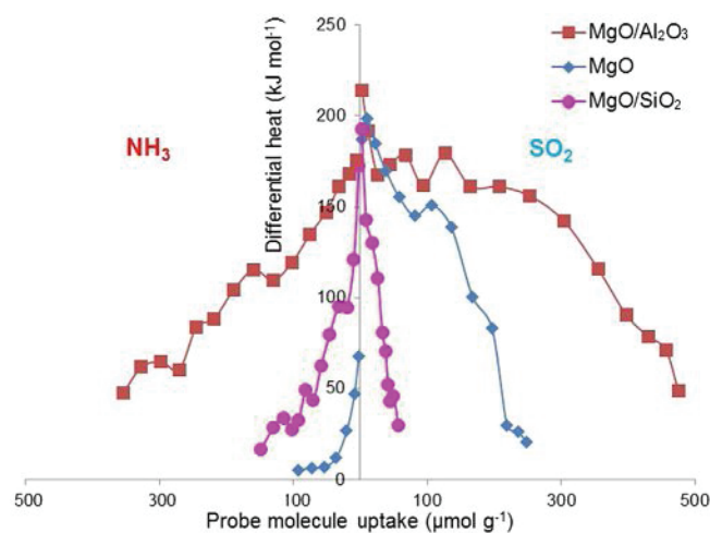
Figure 11. Differential heats of \text{NH}_3 and \text{SO}_2 adsorption versus coverage for \text{MgO}/\text{SiO}_2 , MgO, and \text{MgO}/\text{Al}_2\text{O}_3 samples.
