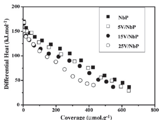
Figure 3.2.5. Differential heats vs. coverage for \text{NH}_3 adsorption over NbP and \text{V}_2\text{O}_5/\text{NbP} catalysts. [45]
