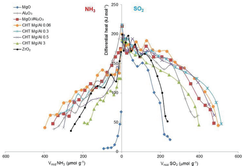
Figure 5. Differential heats \text{NH}_3 and \text{SO}_2 adsorption as a function of surface coverage on basic and amphoteric catalysts.
