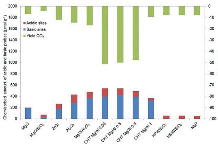
Figure 12. Correlation between acid/base properties of catalysts as determined by adsorption calorimetry and CO x yield (300 °C, GHSV = 10000 h -1 ).
