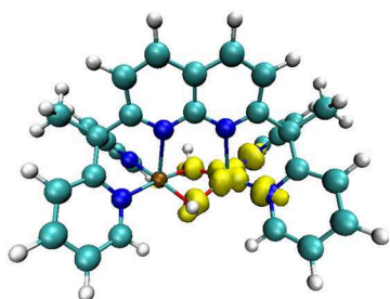
Figure 4. Spin-density plot for \text{I}^{3+} (yellow).
