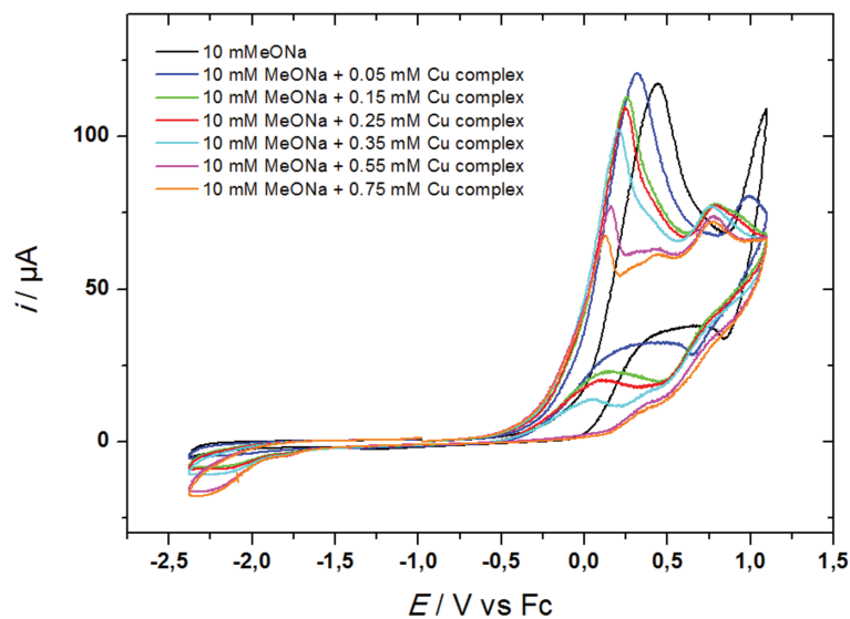
Figure IV.20. CVs at a glassy carbon electrode in DMF / \text{NBu}_4\text{PF}_6 0.1 M under Ar ( \nu = 0.1 \text{ V s}^{-1} ) of MeONa (10 mM) before (black) and after (blue) addition of 0.05 mM (blue), 0.15 mM (green), 0.25 mM (red), 0.35 mM (cyan), 0.55 mM (pink), 0.75 mM (orange) of complex 5 .
