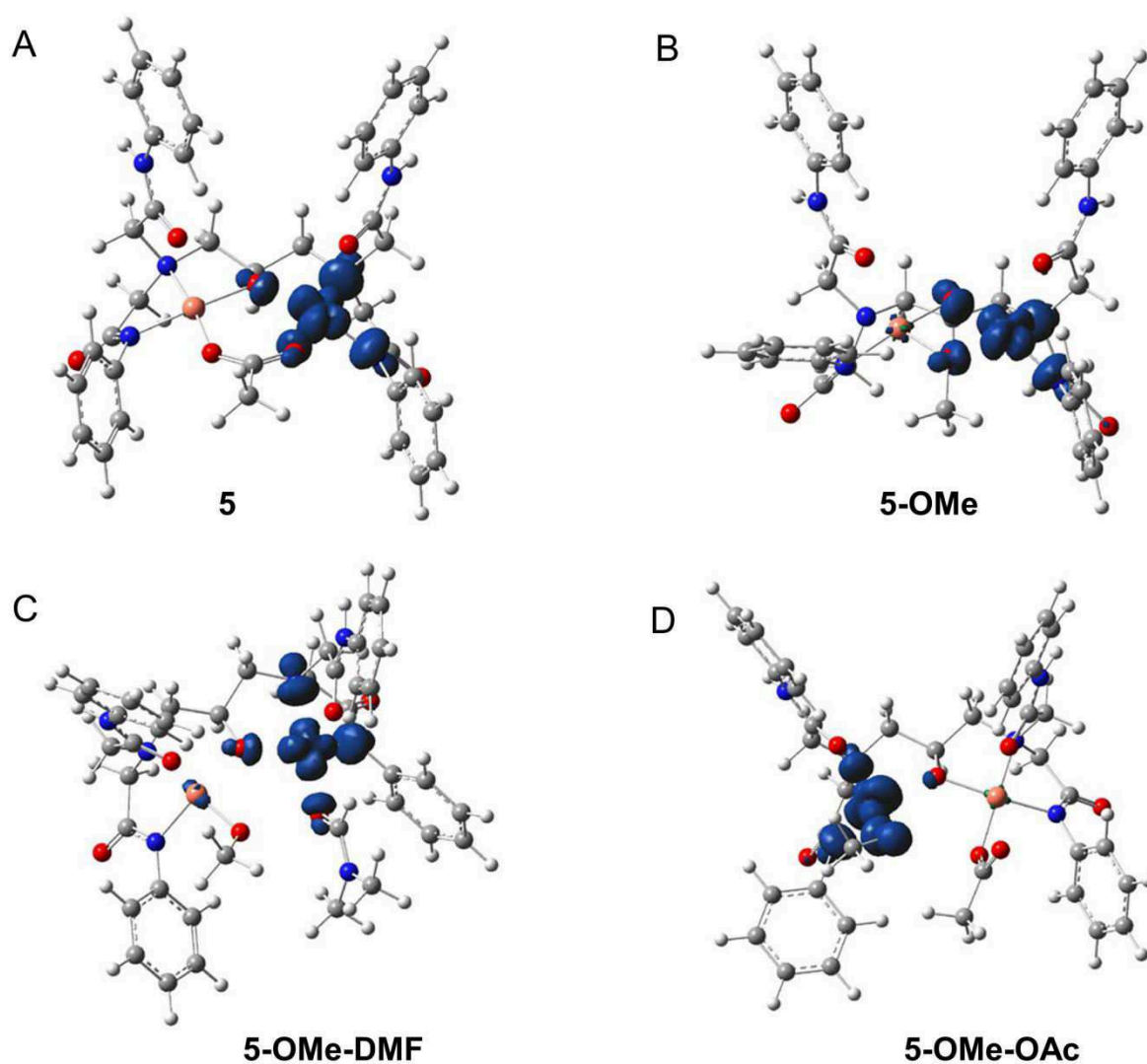
Figure IV.26. Spin density plot for mono-oxidized form of complexes A) 5 , B) 5-OMe , C) 5-OMe-DMF , and D) 5-OMe-OAc .
