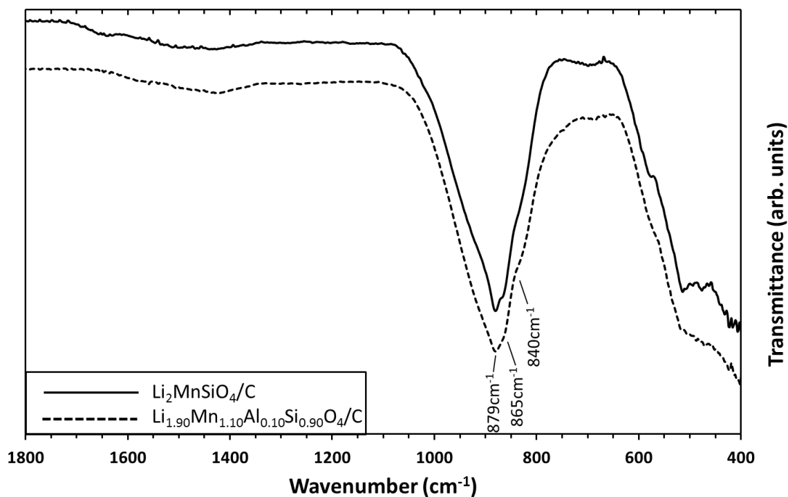
Figure 3-36. ATR-FTIR spectra of Li 2 MnSiO 4 /C (straight line) and Li 1.90 Mn 1.10 Al 0.10 Si 0.90 O 4 /C (dashed line). The spectra were recorded in inert atmosphere.
