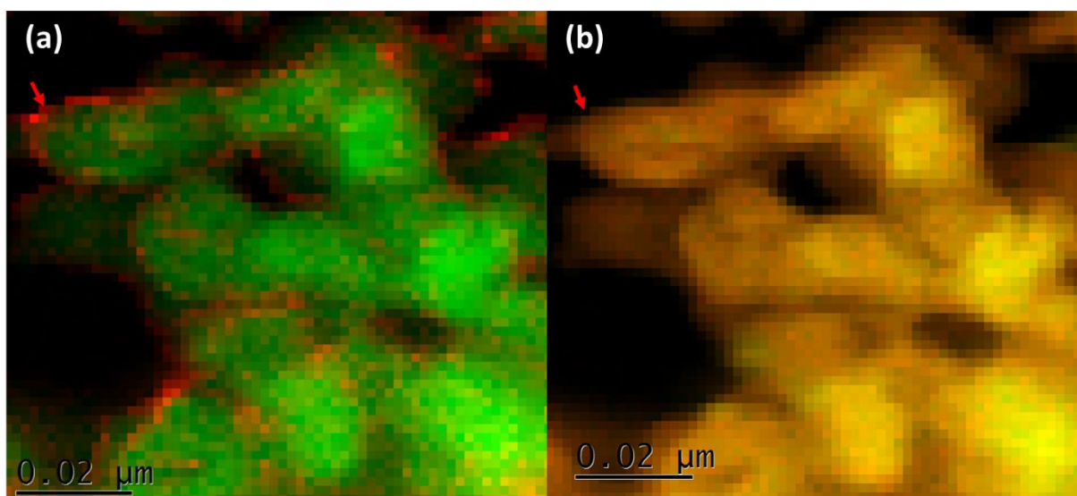
Figure 3-44. STEM-EELS mapping of O (a) and C (b) in HAADF mode of LMS/C 81 exposed 4.5 days to air. C and O are respectively colored in red in (a) and (b), while the LMS/C image are both colored in green.
