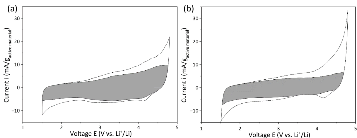
Figure 4-39. Cyclic voltammetry scan at 50\mu\text{V}\cdot\text{s}^{-1} of (a) oxidized MgMnSiO 4 /C and (b) oxidized MgMnSiO 4 /C treated in molten salts, between 1.5V and 4.8V at room temperature. The representation is inspired from [297].
