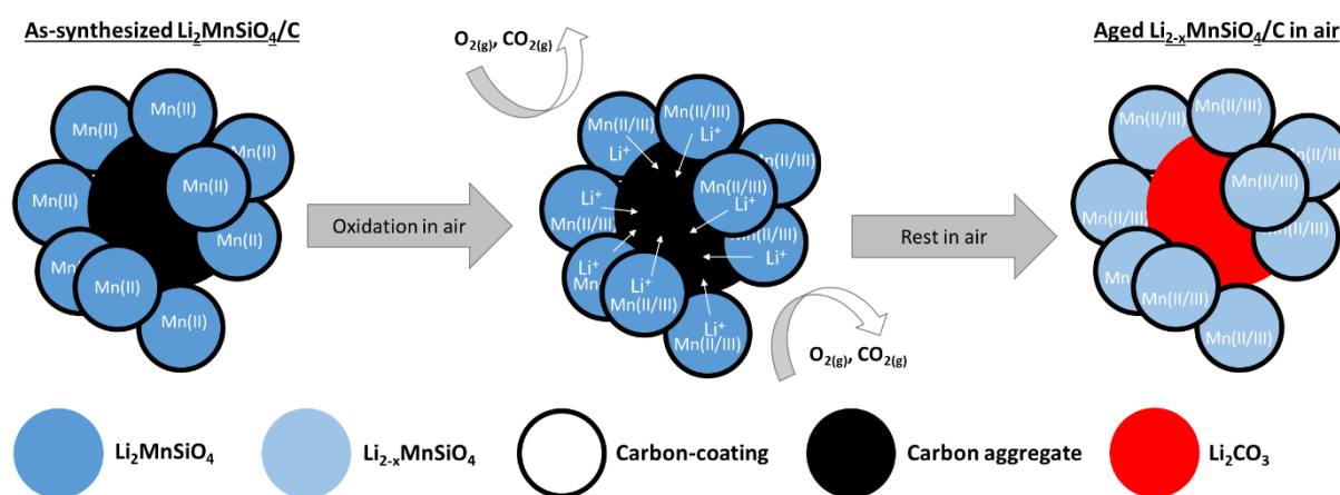
Figure 3-46. Scheme illustrating the main mechanism of the reactivity of Li 2 MnSiO 4 /C with air.
