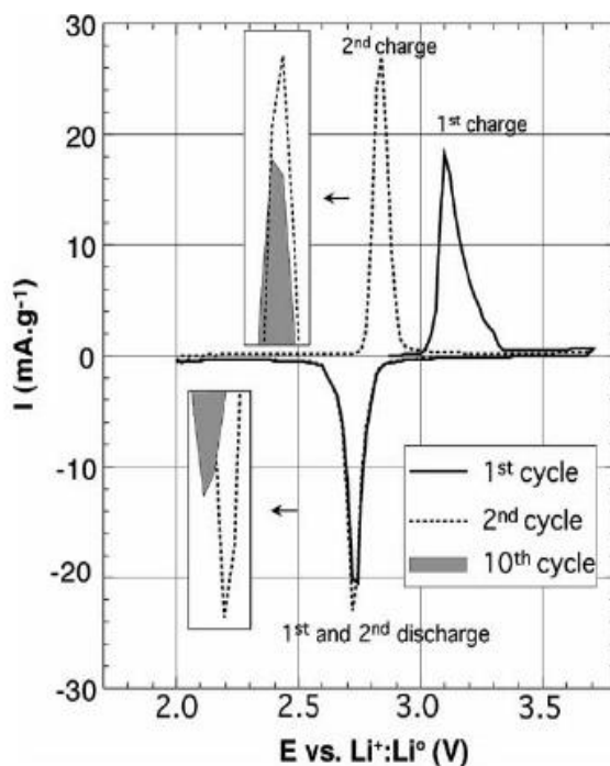
Figure 1-19. Cyclic voltammetry curve of first cycles of Li_2FeSiO_4/C at 20mV.h^{-1} [94].
