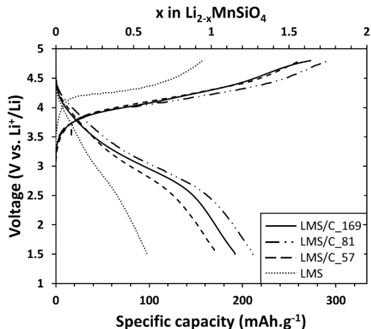
Figure 3-21. First galvanostatic cycles of LMS, LMS/C 57 , LMS/C 81 and LMS/C 169 electrodes at C/20 and room temperature between 1.5V and 4.8V. Dotted line, dashed line, dotted-dashed mixed line and straight line correspond to LMS, LMS/C 57 , LMS/C 81 and LMS/C 169 materials respectively.
