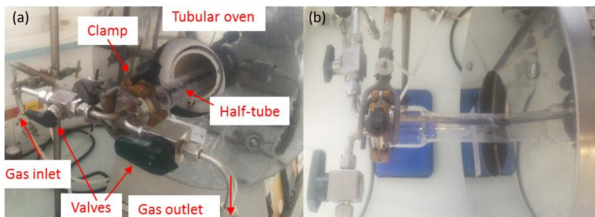
Figure 3-7. (a) Side and (b) top views of an in-house manufactured half-tube system that isolates the sample from air during and after pyrolysis.
