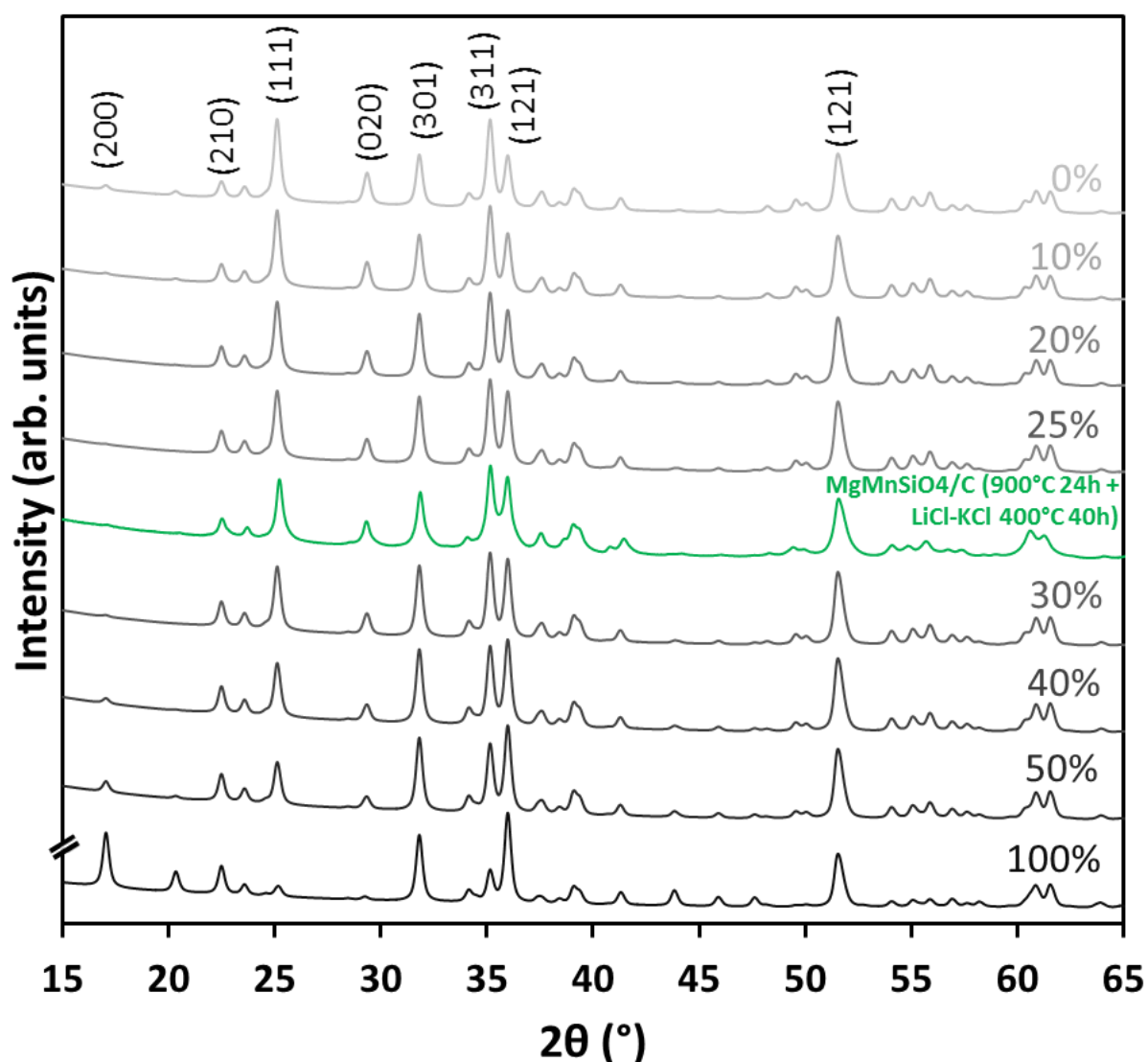
Figure 4-17. Simulated diffraction patterns of olivine MgMnSiO 4 with different antisite mixing from 100% (100% Mn 2+ on M1 site) to 0% (100% Mg 2+ on M1 site) using Fullprof software. The lattice parameters ( a=10.460(7)\text{\AA} , b=6.123(2)\text{\AA} and c=4.803(3)\text{\AA} ) are based on the experimental diffraction patterns of MgMnSiO 4 /C pyrolyzed at 900°C for 24h and treated in LiCl-KCl molten salt flux at 400°C for 40h, that is also shown in green. The major reflections impacted by the antisite mixing are labelled by their Miller index on the top of the figure.
