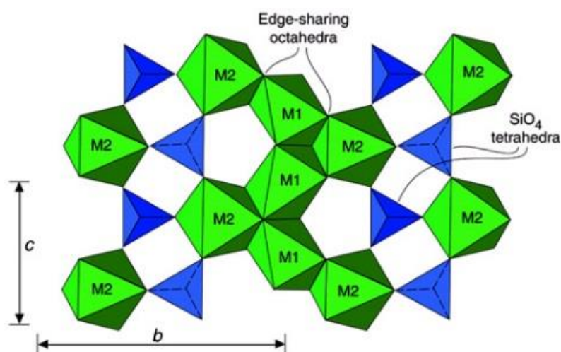
Figure 1-33. Cross-section view of (bc) plane of olivine silicate, from [217]. M1 and M2 octahedral sites (green) correspond to A and B in olivine \text{ABSiO}_4 , while blue tetrahedra represent \text{SiO}_4 units.
