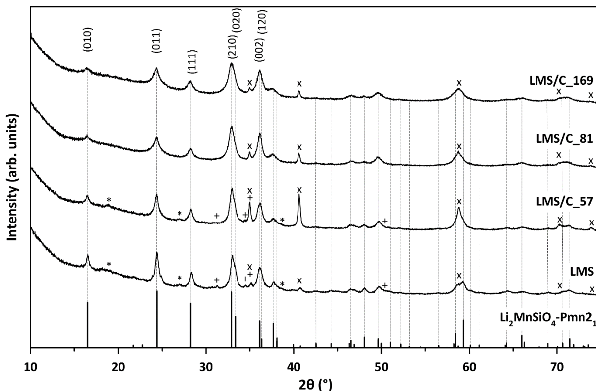
Figure 3-16. Powder X-Ray Diffraction patterns of Li 2 MnSiO 4 /C composites and Li 2 MnSiO 4 pyrolyzed at 650°C for 0.5h in argon. The main peaks of each impurity are displayed and denoted as the following: Li 2 SiO 3 (*), Mn 2 SiO 4 (+) and MnO (x). The Miller indexes of the main reflections of Pmn2 1 Li 2 MnSiO 4 are exhibited on the top.
