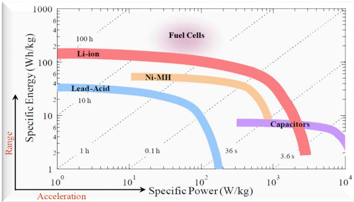
Figure 0-2. Ragone plot of electrochemical devices according to their specific energy ( \text{Wh}\cdot\text{kg}^{-1} ) and specific power ( \text{W}\cdot\text{kg}^{-1} ), adapted from [9].
