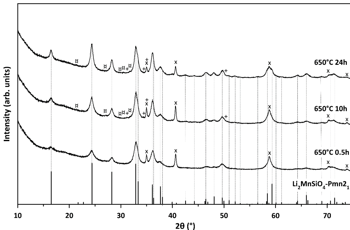
Figure 3-14. Powder X-Ray Diffraction patterns of Li 2 MnSiO 4 /C described in the Pmn2 1 space group and pyrolyzed at 650°C in argon for 0.5h, 10h and 24h. The main peaks of each impurity are displayed and denoted as the following: Li 2 CO 3 (⊠), Li 2 SiO 3 (*), Mn 2 SiO 4 (+) and MnO (x). The reflections of Pmn2 1 -Li 2 MnSiO 4 are indicated by dotted vertical lines.
