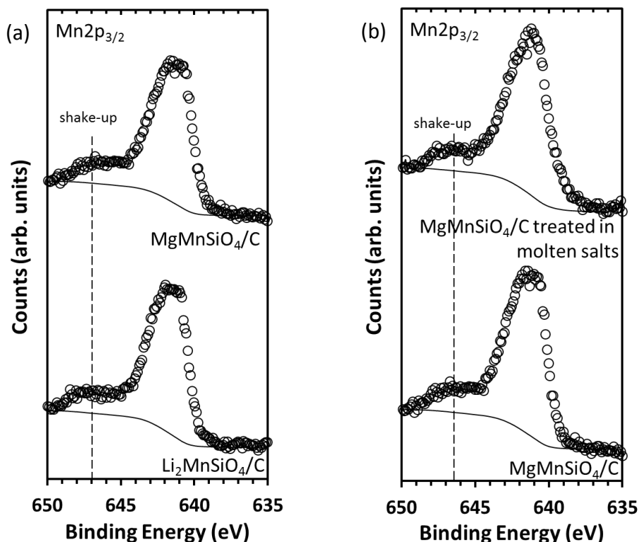
Figure 4-20. XPS Mn2p 3/2 core spectra of (a) Li 2 MnSiO 4 /C and pristine MgMnSiO 4 /C and (b) pristine MgMnSiO 4 /C and MgMnSiO 4 /C treated in molten salts. Calibration with Si2p orbital at 101.7eV.
