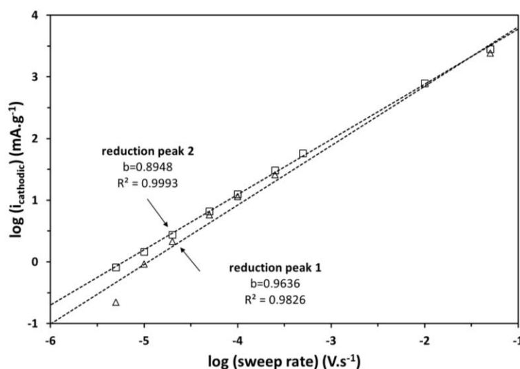
Figure 4-36. Evolution of reduction peaks current as a function of sweep rate for oxidized MgMnSiO 4 /C. The reduction peaks here correspond to those of Figure 4-35. The slope, b , of Equation 4-4 is indicated as well as the correlation coefficient, R^2 .
