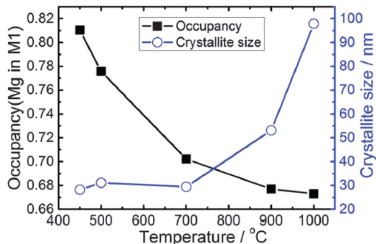
Figure 1-34. Mg occupancy on M1 site and crystallite size of \text{MgMnSiO}_4 as function of temperature of synthesis, from [223].
