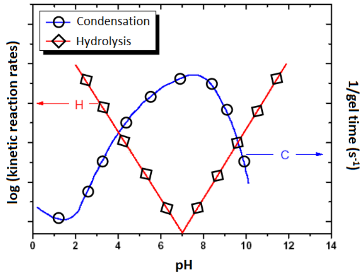
Figure 2-3. Evolution of hydrolysis and condensation kinetics as function of pH, adapted from [244].
