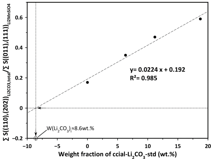
Figure 3-41. Ratio of (110) and (202) Li 2 CO 3 peaks area to (011) and (111) Li 2 MnSiO 4 peaks area as a function of ccial-Li 2 CO 3 -std weight fraction. The equation of the correlated linear function, y=a*x+b , and the correlation coefficient, R^2 , are indicated.
