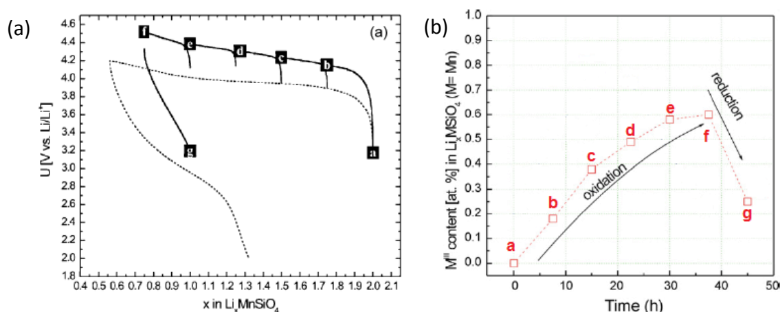
Figure 1-30. First galvanostatic cycle of \text{Li}_2\text{MnSiO}_4 XAS half-cell at different stages of charge and discharge (a: pristine, b: extraction of 0.25\text{Li}^+ , c: extraction of 0.5\text{Li}^+ , d: extraction of 0.75\text{Li}^+ , e: extraction of 1\text{Li}^+ , f: extraction of 1.25\text{Li}^+ , g: insertion of 0.25\text{Li}^+ ) (a); Proportion of \text{Mn}^{3+} in \text{Li}_2\text{MnSiO}_4 electrode, determined from XANES spectra related to state of charges indicated on the galvanostatic curve (b); adapted from [115].
