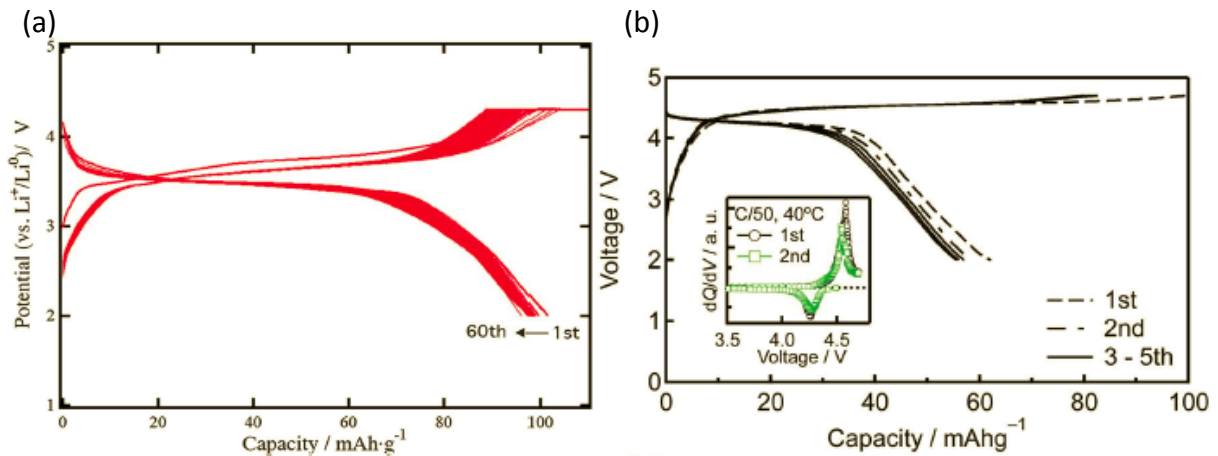
Figure 1-7. (a) Galvanostatic charge–discharge curves for \text{Li}_2\text{FeP}_2\text{O}_7 positive electrode at C/20 [57], Galvanostatic voltage–composition curve of \text{Li}_2\text{MnP}_2\text{O}_7 at a rate of C/50 obtained at 40^\circ\text{C} , the corresponding dQ/dV plot is shown in inset [59].
