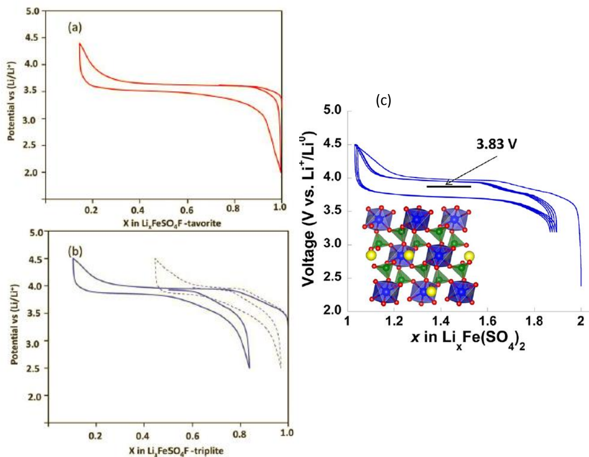
Figure 1-11. Galvanostatic charge-discharge of (a) tavorite \text{LiFeSO}_4\text{F} , (b) triplite \text{LiFeSO}_4\text{F} at C/10 [85] and (c) \text{Li}_2\text{Fe}(\text{SO}_4)_2 [82].
