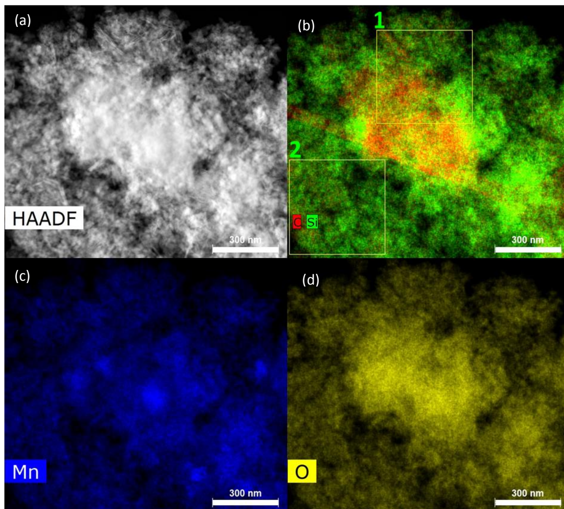
Figure 3-45. STEM image of LMS/C 81 exposed 4.5 days to air (a) and related EDX mapping of C and Si (b), Mn (c) and O (d). Two regions (1 and 2) are probed and are indicated by squares in (b). C, Si, Mn, O are respectively colored in red, green, blue and yellow.
