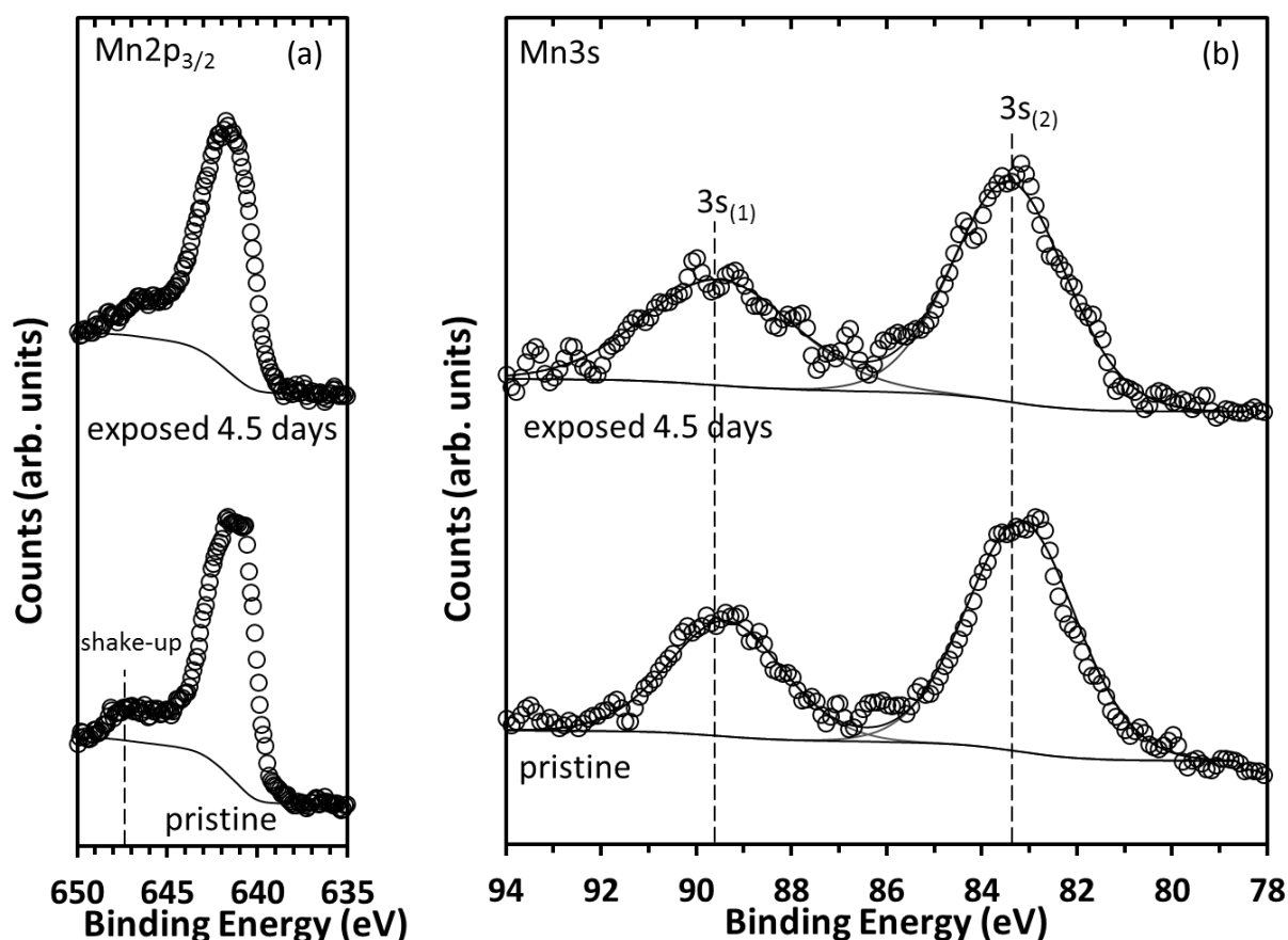
Figure 3-44. XPS Mn2p 3/2 (a) and Mn3s (b) spectra of pristine and exposed 4.5 days to air LMS/C_81 materials. Split peaks of Mn3s at high and low binding energies are respectively denoted 3s (1) and 3s (2) . Spectra were calibrated with the “SiO 4 ” O1s component at 530.5eV.
