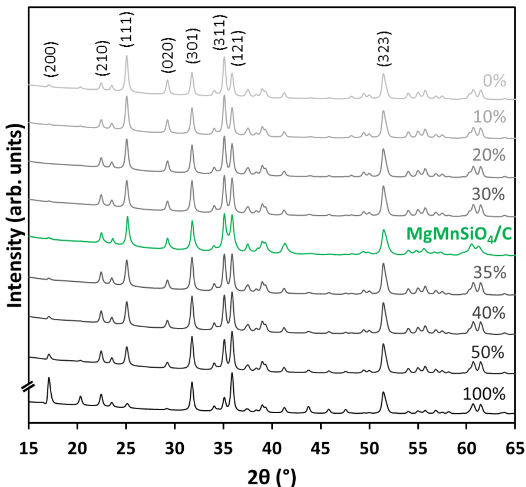
Figure 4-13. Simulated diffraction patterns of the olivine \text{MgMnSiO}_4/\text{C} material with different antsite mixing from 100% (100% \text{Mn}^{2+} on M1 site) to 0% (100% \text{Mg}^{2+} on M1 site) using Fullprof software. Lattice parameters ( a=10.457(6)\text{\AA} , b=6.129(8)\text{\AA} and c=4.810(6)\text{\AA} ) are based on the experimental diffraction patterns of \text{MgMnSiO}_4/\text{C} pyrolyzed at 900^\circ\text{C} for 24h that is also shown in green. The major reflections impacted by the antsite mixing are labelled by their Miller index on the top of the figure.
