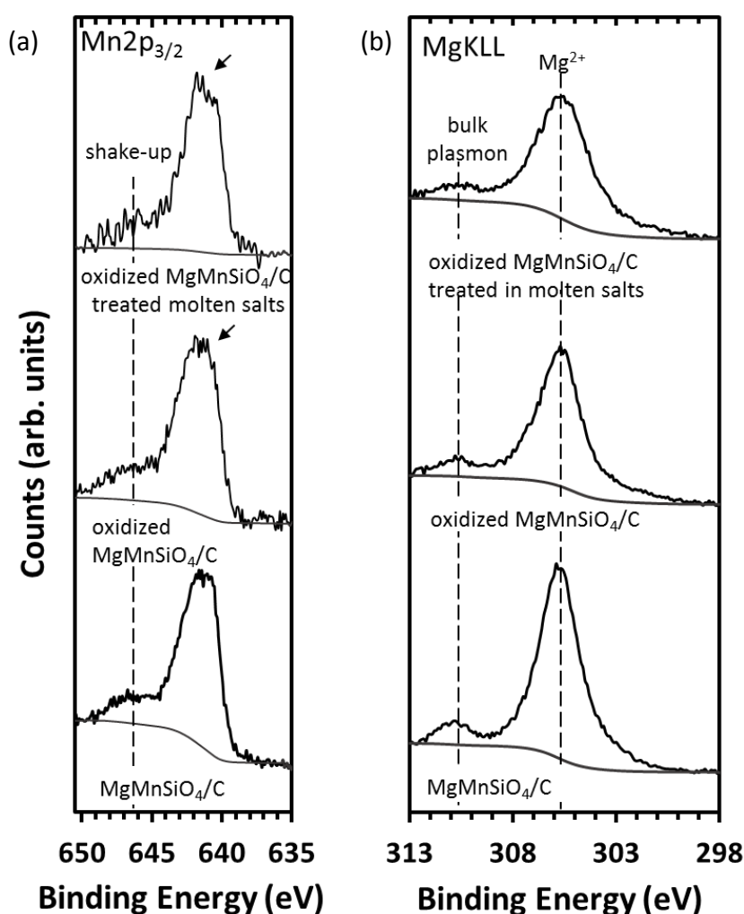
Figure 4-28. (a) XPS Mn2p 3/2 core spectra and (b) Mg KLL Auger spectra of MgMnSiO 4 /C, oxidized MgMnSiO 4 /C and chemical oxidized MgMnSiO 4 /C treated in molten salts. The arrows indicate a shoulder in the Mn2p 3/2 main peak representing final states. All spectra were calibrated with SiO 4 component of Si2p orbital at 101.7eV.
