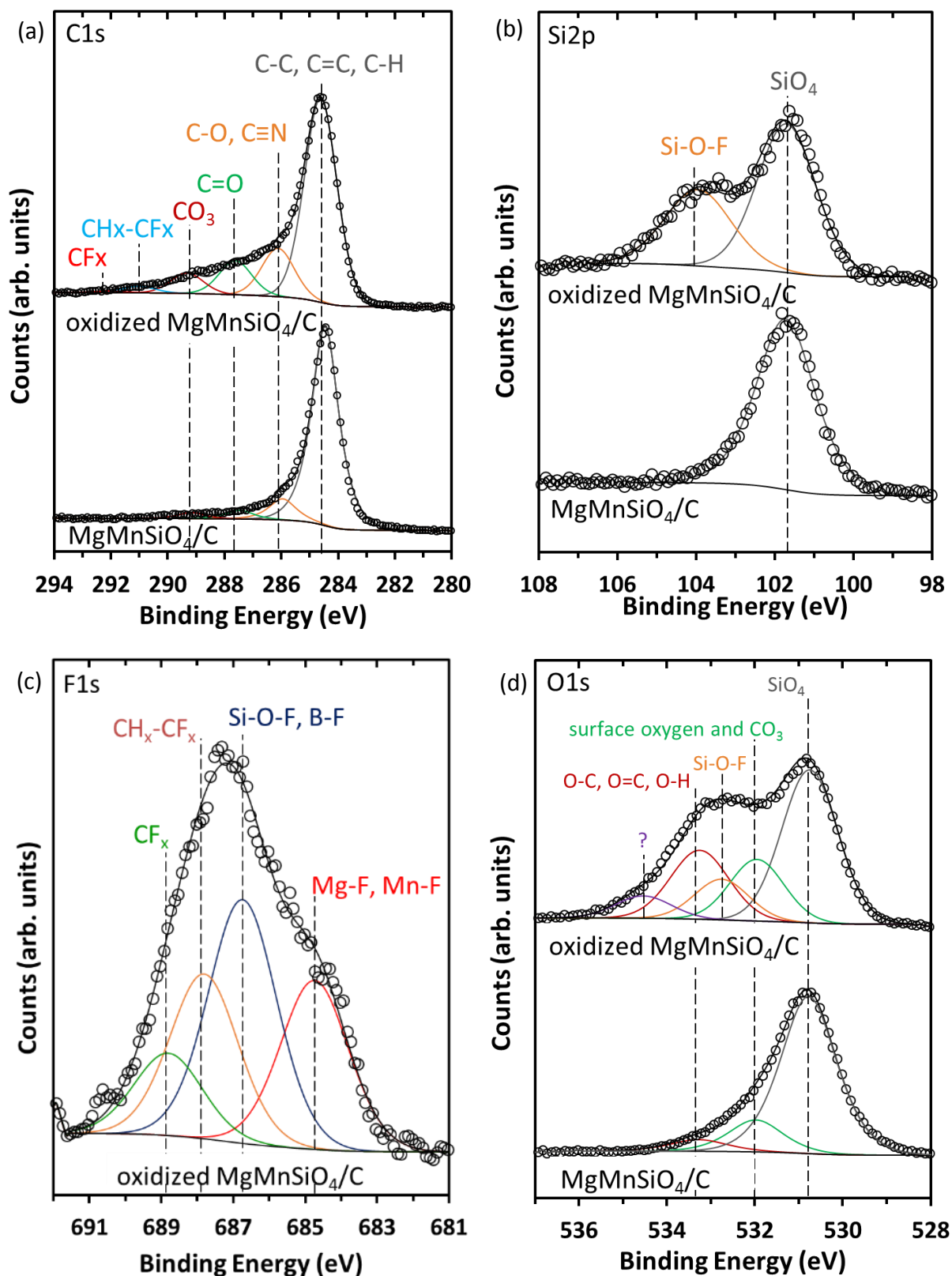
Figure 4-29. XPS core \text{C1s} (a), \text{Si2p} (b), \text{F1s} (c) and \text{O1s} (d) normalized spectra of \text{MgMnSiO}_4/\text{C} and oxidized \text{MgMnSiO}_4/\text{C} . Calibration with \text{Si2p} component of \text{SiO}_4 at 101.7 eV.
