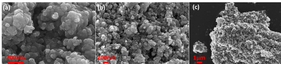
Figure 4-18. Scanning Electron Microscopy images of MgMnSiO 4 /C 900 at different magnifications: (a) x300 000; (b) x100 000; (c) x20 000.
