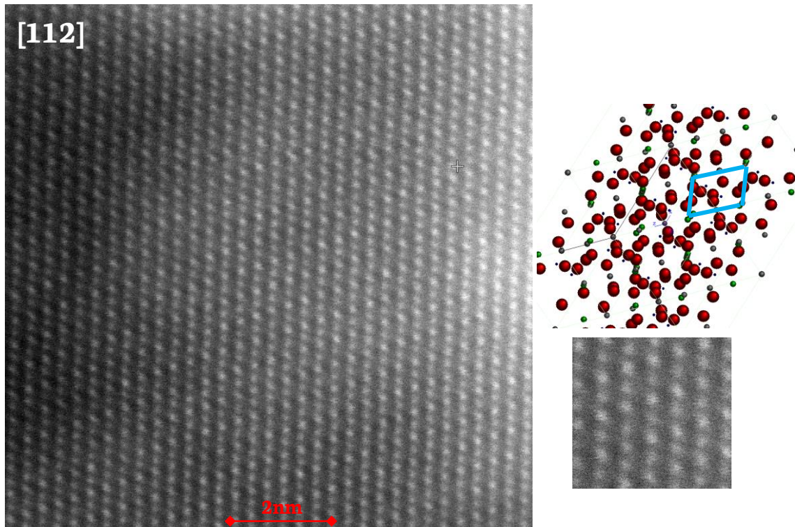
Figure 4-11. High-resolution STEM (HRSTEM) image of \text{MgMnSiO}_4/\text{C} particle observed along the [112] orthorhombic zone axis of the olivine structure. The atomic positions of olivine structure are shown as a model along the [112] with \text{O}^{2-} in red, \text{Mn}^{2+} in green and \text{Mg}^{2+} in grey.
