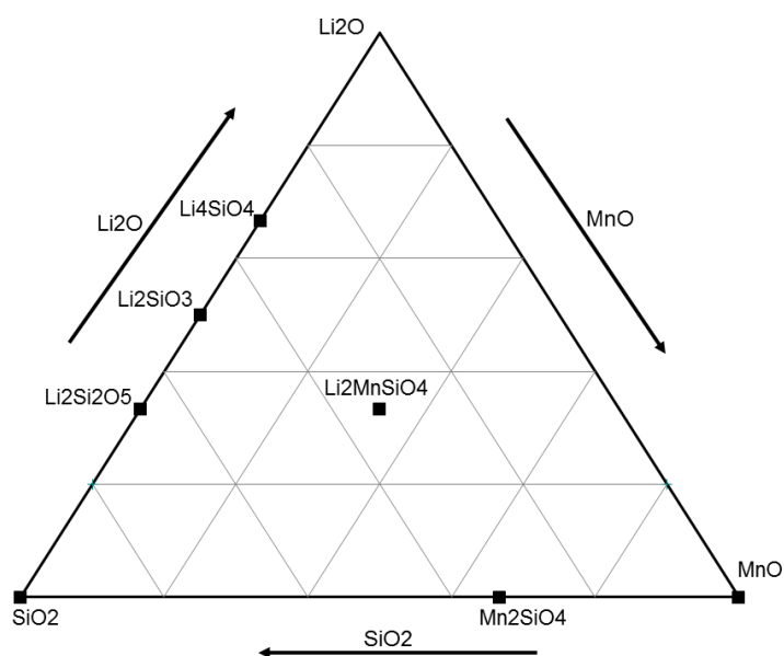
Figure 3-8. Li 2 O-MnO-SiO 2 ternary diagram. Specific compositions marked by a square are relative to common by-products obtained during Li 2 MnSiO 4 synthesis.
