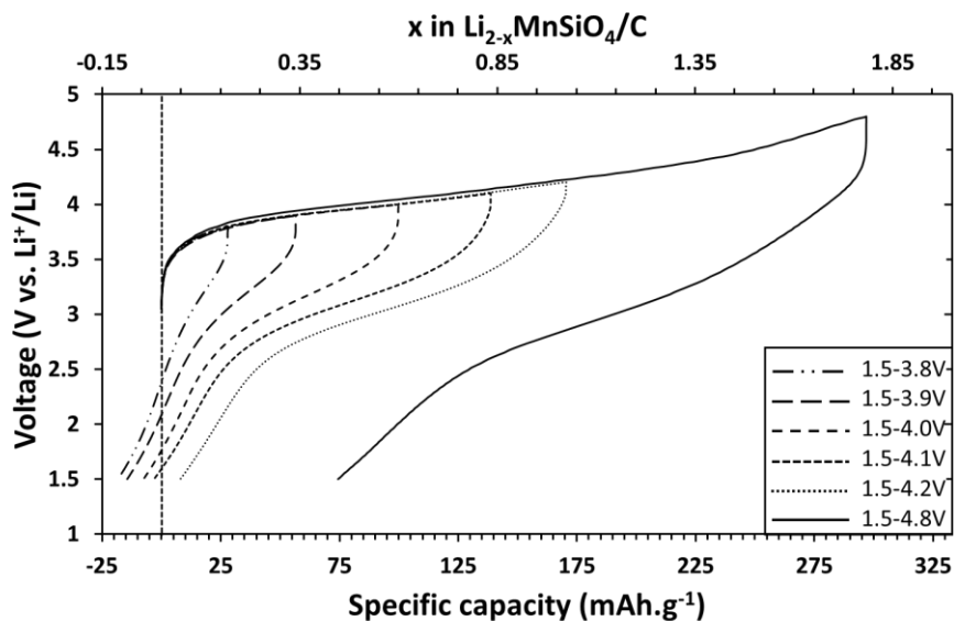
Figure 3-27. First galvanostatic cycle of LMS/C 81 at different upper cut-off voltages (3.8V, 3.9V, 4.0V, 4.1V, 4.2V and 4.8V) at C/20 and room temperature.
