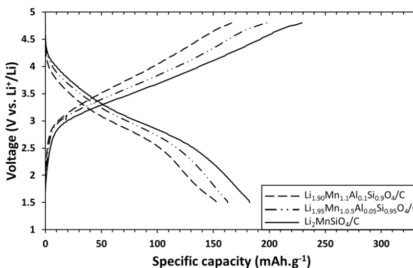
Figure 3-38. Second galvanostatic cycle of \text{Li}_{2-x}\text{Mn}_{1+x}\text{Al}_x\text{Si}_{1-x}\text{O}_4/\text{C} ( x=0, 0.05 and 0.1 ) electrodes at C/20 and room temperature between 1.5V and 4.8V. 1C=333 \text{ mA}\cdot\text{g}^{-1} ; 320 \text{ mA}\cdot\text{g}^{-1} and 308 \text{ mA}\cdot\text{g}^{-1} respectively for x=0; 0.05 and 0.10 . \text{Li}_{2-x}\text{Mn}_{1+x}\text{Al}_x\text{Si}_{1-x}\text{O}_4/\text{C} , with x=0 , correspond to the reference material LMS/C_81.
