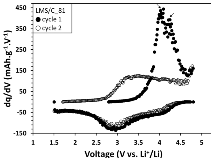
Figure 3-23. dq/dV plots of first and second galvanostatic cycles of LMS/C_81 electrodes at C/20 and room temperature between 1.5V and 4.8V. Filled and empty circles correspond to first and second cycles respectively. Black arrows indicate the oxidation peaks upon first oxidation/charge.
