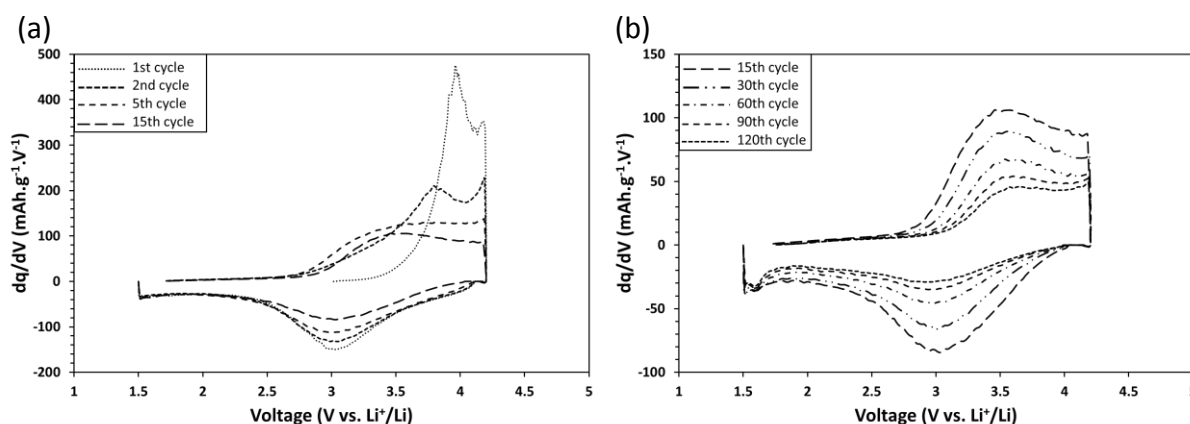
Figure 3-29. dq/dV plots of (a) 1 st , 2 nd , 5 th and 15 th and (b) 15 th , 30 th , 60 th , 90 th and 120 th galvanostatic cycles of LMS/C 81 between 1.5V and 4.2V at C/20 and room temperature.
