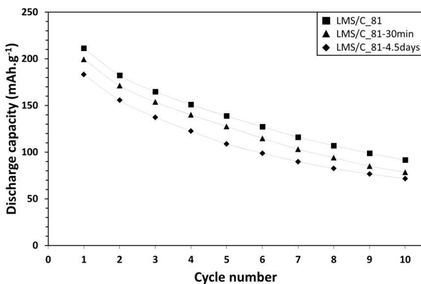
Figure 3-48. Cycling performance of pristine LMS/C 81 (square), LMS/C 81 exposed 30minutes to air, LMS/C 81 -30min (triangle) and LMS/C 81 exposed 4.5 days to air, LMS/C 81 -4.5days (diamond), at C/20 and room temperature between 1.5V and 4.8V.
