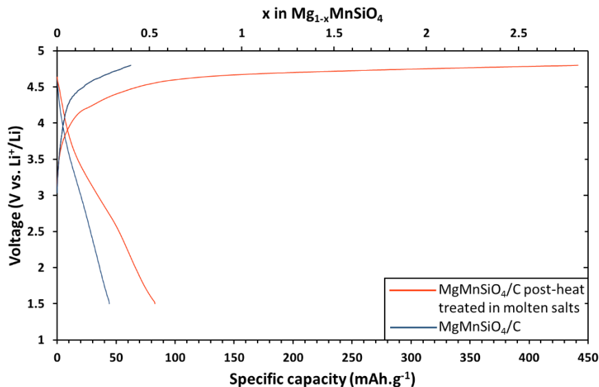
Figure 4-21. First galvanostatic charge and discharge of \text{MgMnSiO}_4/\text{C} pyrolyzed at 900^\circ\text{C} for 24h (blue line) and \text{MgMnSiO}_4/\text{C} treated in LiCl-KCl molten salts flux (orange line) electrodes between 1.5\text{V} and 4.8\text{V} at C/20 ( 1C=313\text{mAh.g}^{-1} ) and room temperature. The electrolyte and counter-electrode used are respectively based on a \text{LiPF}_6 salt and a lithium counter-electrode.
