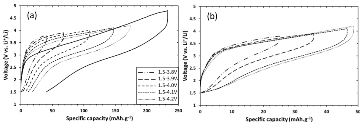
Figure 3-31. (a) 2 nd and (b) 120 th galvanostatic cycle of LMS/C_81 respectively for the 3.8V, 3.9V, 4.0V, 4.1V and 4.2V upper cut-off voltages, at C/20 and room temperature.
