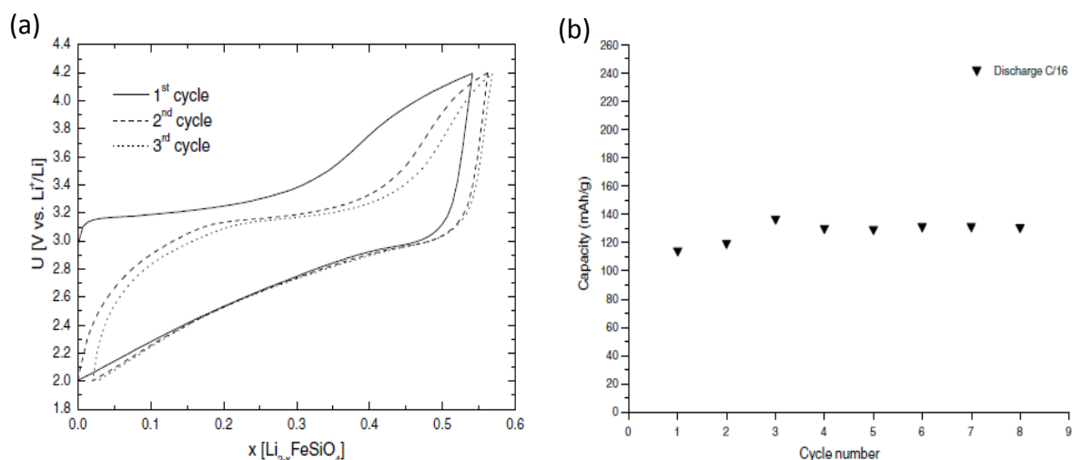
Figure 1-20. (a) First galvanostatic cycles of \text{Li}_2\text{FeSiO}_4/\text{C} at \text{C}/30 [95] and (b) cycling performance of \text{Li}_2\text{FeSiO}_4/\text{C} at \text{C}/16 and 60^\circ\text{C} [94].
