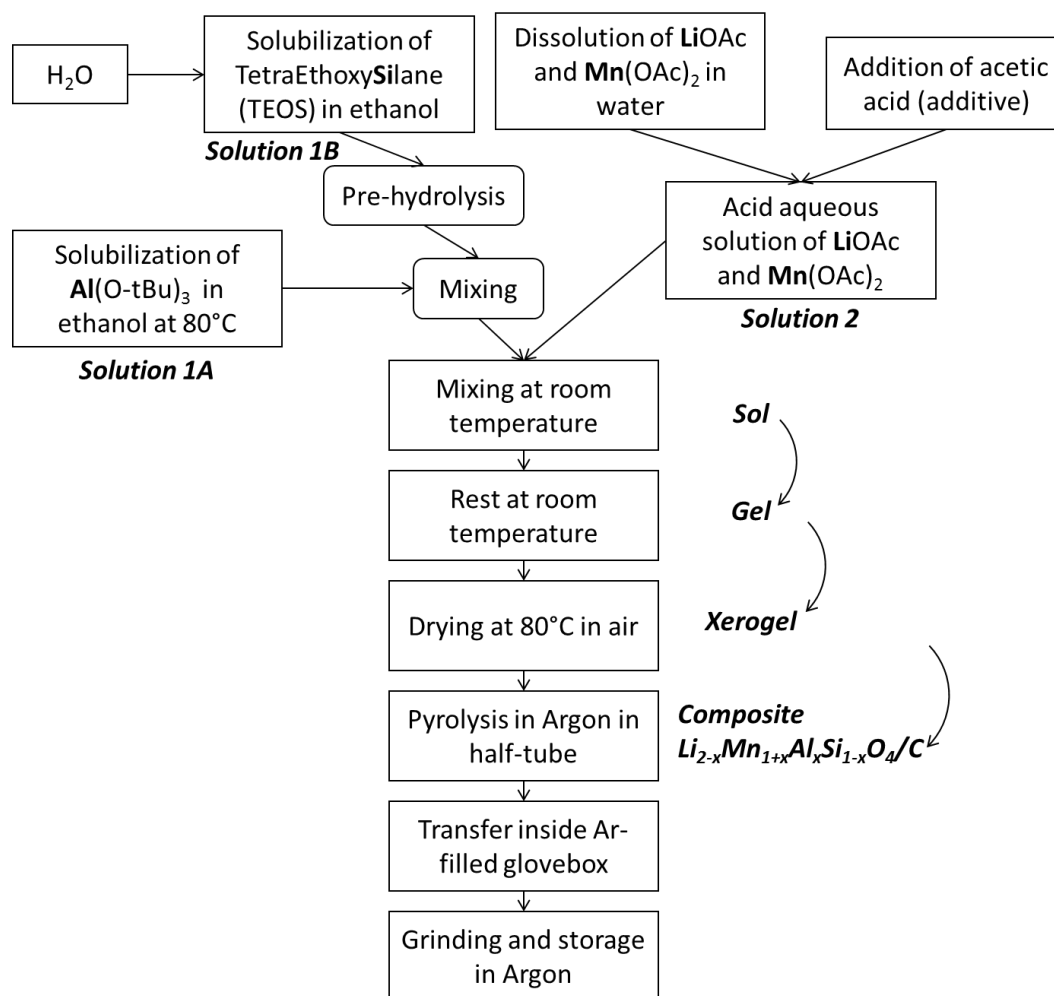
Figure 3-33. Protocol of the sol-gel synthesis of \text{Li}_{2-x}\text{Mn}_{1+x}\text{Al}_x\text{Si}_{1-x}\text{O}_4/\text{C} in inert atmosphere.
