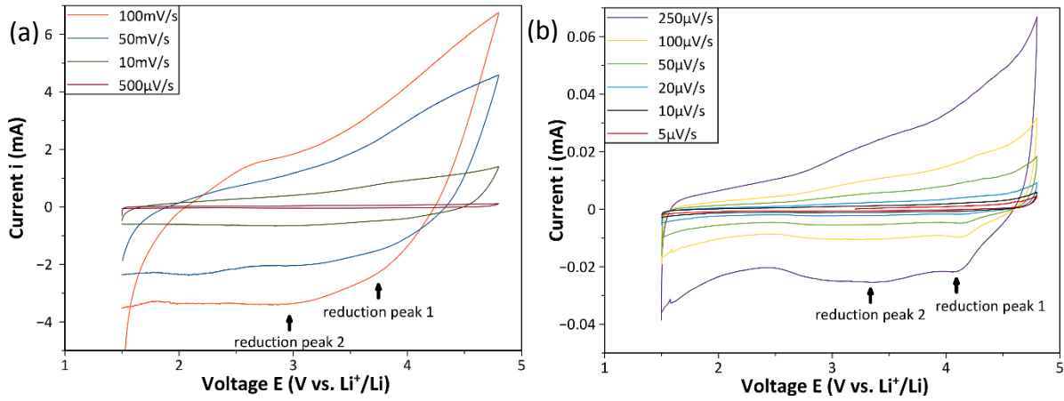
Figure 4-35. Cyclic voltammetry scans of oxidized \text{MgMnSiO}_4/\text{C} at (a) 500\mu\text{V}\cdot\text{s}^{-1} - 100\text{mV}\cdot\text{s}^{-1} sweep rates and (b) 5\mu\text{V}\cdot\text{s}^{-1} - 250\mu\text{V}\cdot\text{s}^{-1} sweep rates between 1.5V and 4.8V at room temperature. Oxidation and reduction peaks are indicated by a number in order of appearance.
