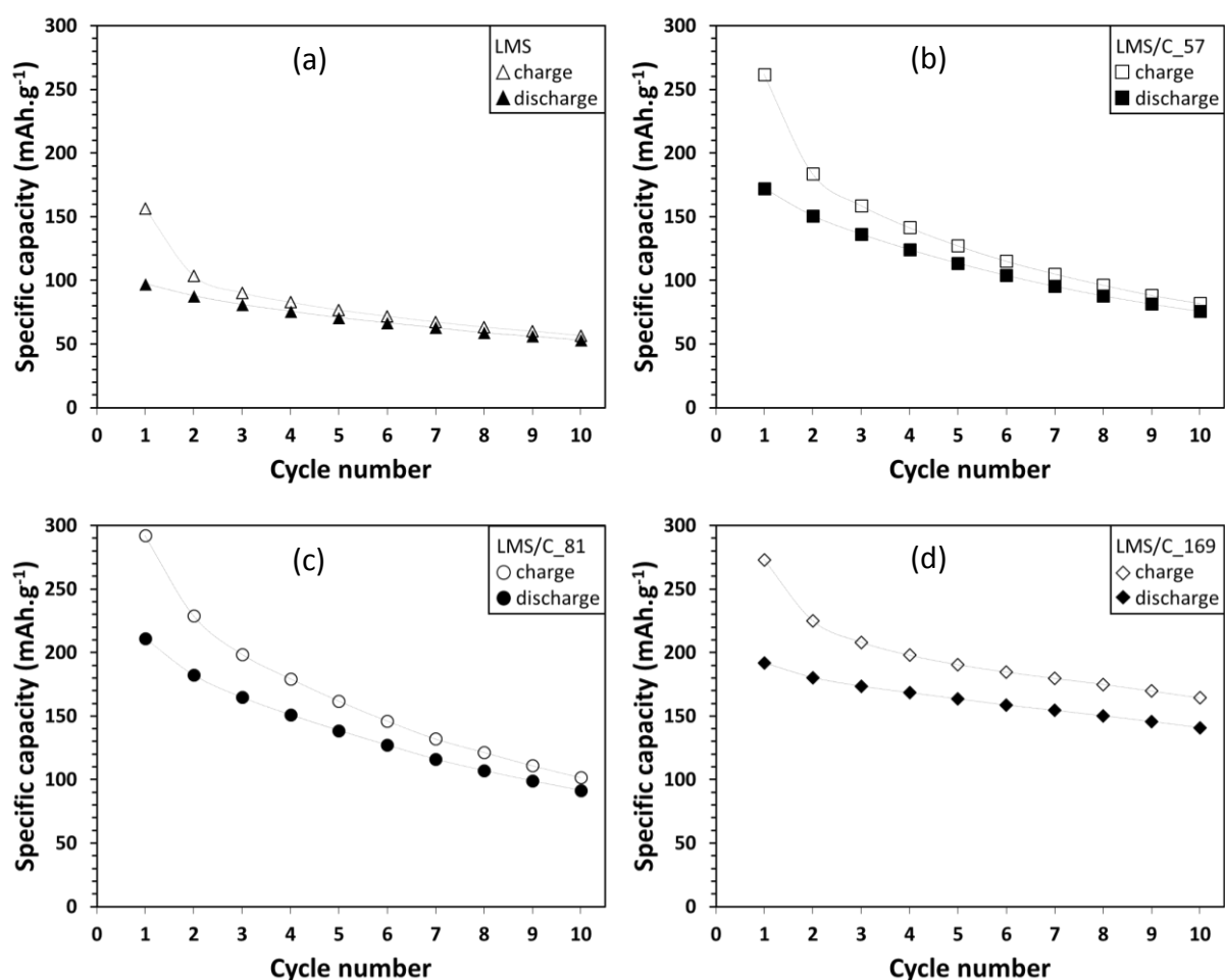
Figure 3-24. Cycling performance of LMS (a), LMS/C 57 (b), LMS/C 81 (c) and LMS/C 169 (d) electrodes at C/20 and room temperature between 1.5V and 4.8V. The empty and filled symbols respectively correspond to charge and discharge specific capacities.
