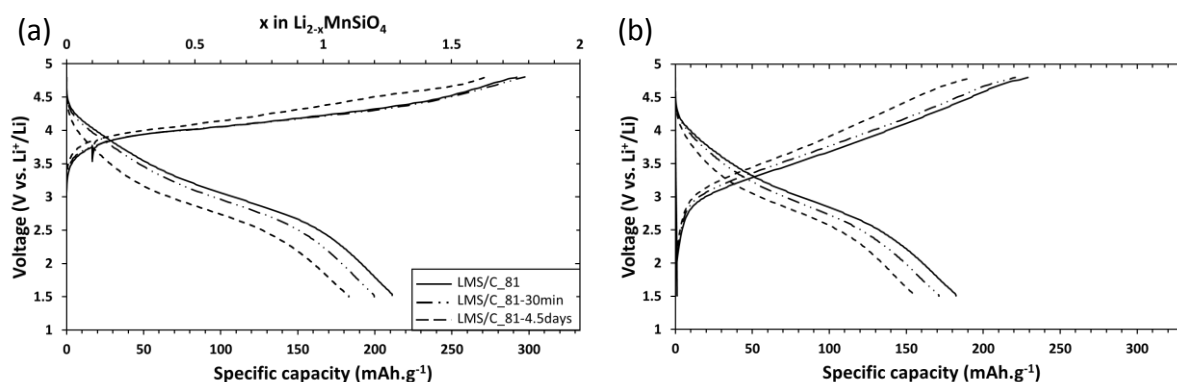
Figure 3-47. First (a) and second (b) galvanostatic cycle of pristine LMS/C_81 (straight line), LMS/C_81 exposed 30minutes to air, LMS/C_81-30min (dotted-dashed line) and LMS/C_81 exposed 4.5 days to air, LMS/C_81-4.5 days (dashed line), at C/20 and room temperature between 1.5V and 4.8V.
