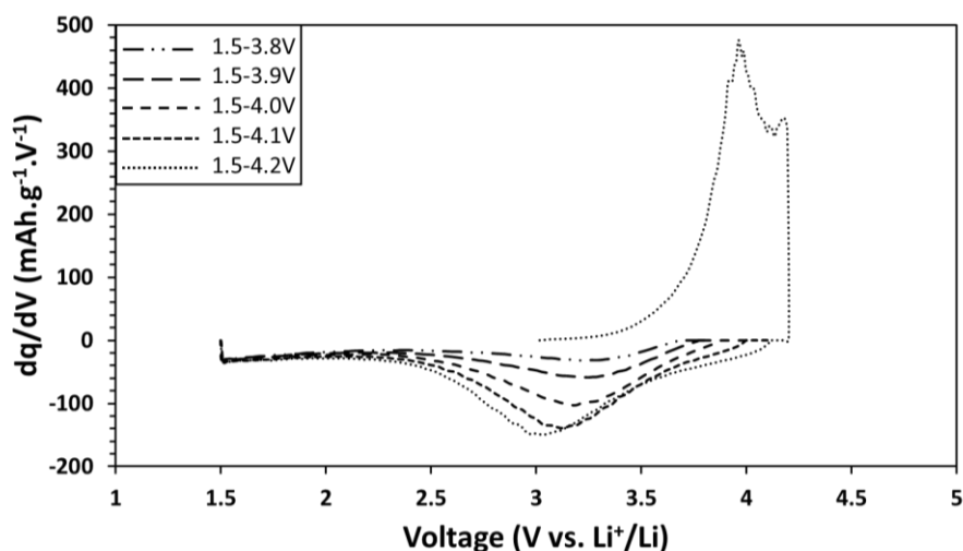
Figure 3-28. dq/dV plot of the first galvanostatic cycle of LMS/C 81 , exhibiting the charge voltage profile of the 4.2V upper cut-off voltage and the discharge voltage of the 3.8V, 3.9V, 4.0V, 4.1V and 4.2V upper cut-off voltages at C/20 and room temperature.
