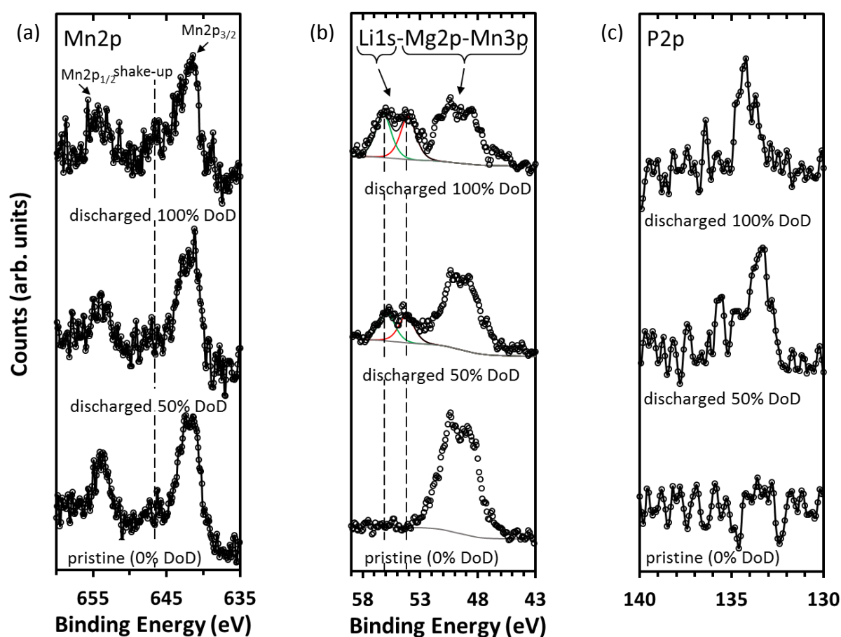
Figure 4-44. (a) Mn2p, (b) Li1s and (c) P2p XPS core spectra of oxidized \text{MgMnSiO}_4/\text{C} treated in molten salts electrodes first discharged at C/10 at 0%, 50% and 100% DoD. Calibration with C1s at 284.8eV.
