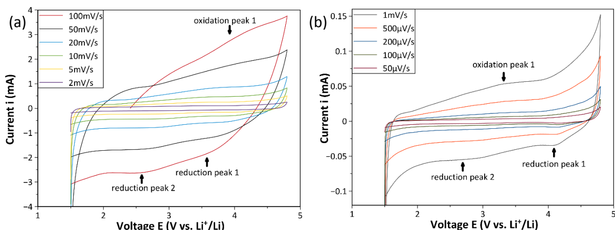
Figure 4-37. Cyclic voltammograms of oxidized MgMnSiO 4 /C treated in molten salts at (a) 2 mV.s -1 -100 mV.s -1 sweep rates and 50 μV.s -1 -1 mV.s -1 sweep rates between 1.5 V and 4.8 V at room temperature. Oxidation and reduction peaks are indicated by a number in order of appearance.
