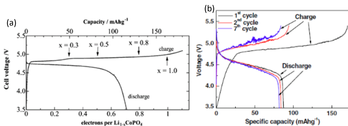
Figure 1-5. Galvanostatic charge-discharge cycles of (a) \text{LiCoPO}_4 at 0.1\text{mA.cm}^{-2} and (b) \text{LiNiPO}_4/\text{C} at \text{C}/10 , respectively adapted from [48] and [49].
