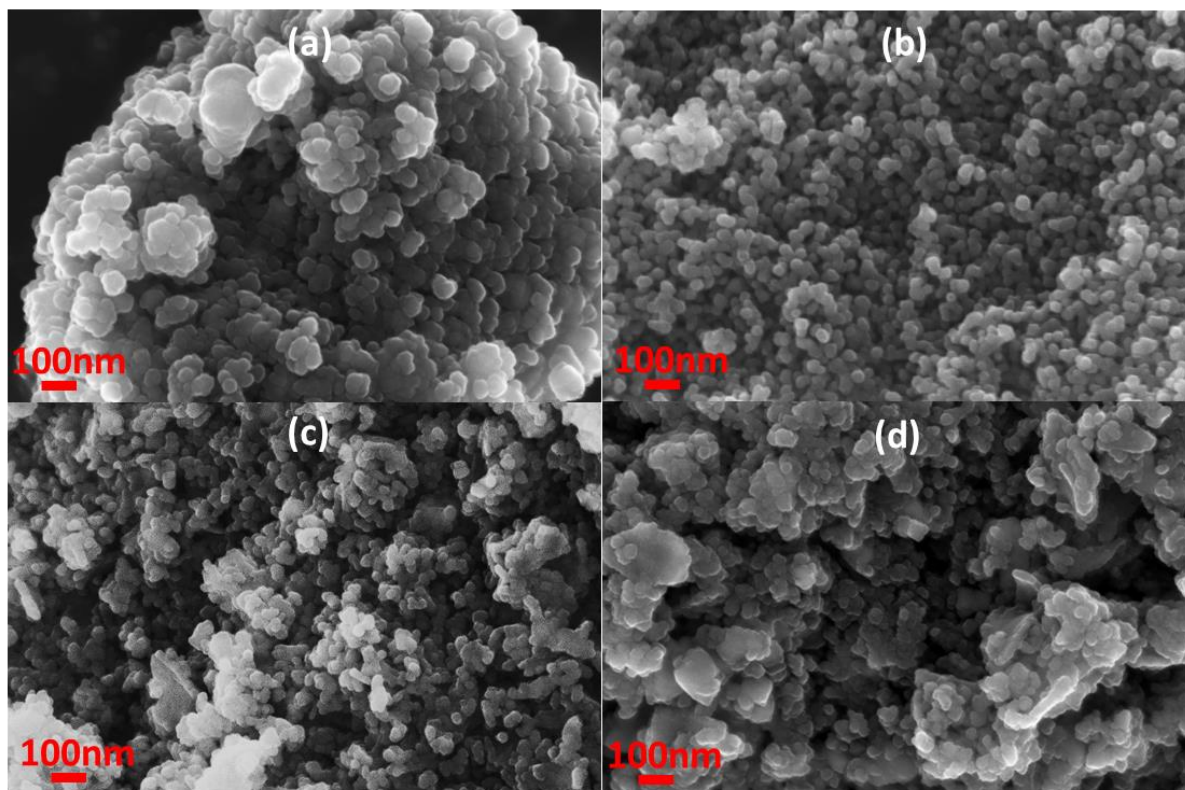
Figure 3-17. Scanning Electron Microscopy images of LMS (a), LMS/C 57 (b), LMS/C 81 (c) and LMS/C 169 (d).
