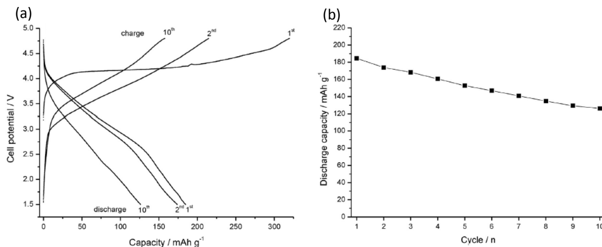
Figure 1-27. Galvanostatic cycles of a \text{Li}_2\text{MnSiO}_4/\text{C} material between 1.5V and 4.8V at C/50 and room temperature (a), and associated discharge capacity as a function of cycle number (b), adapted from [161].
