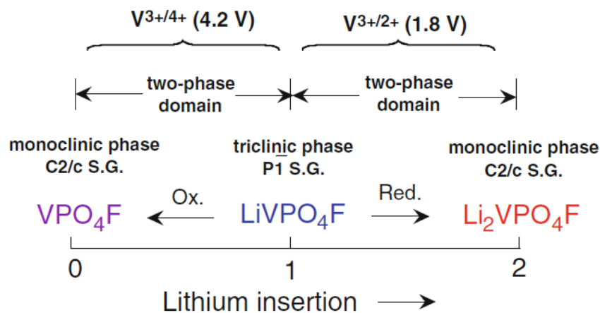
Figure 1-8. Schematic diagram of voltage–structure of \text{Li}_x\text{VPO}_4\text{F} ( 0 \leq x \leq 2 ) material [62].
