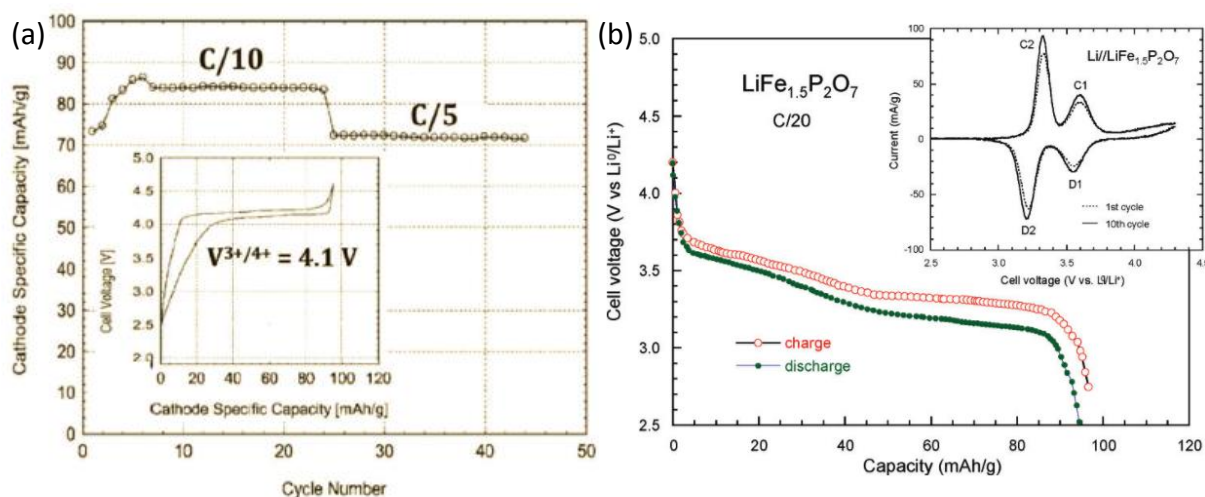
Figure 1-6. Reversible electrochemical capacity close to 90\text{mAh}\cdot\text{g}^{-1} depicted for carbothermally produced \text{LiVP}_2\text{O}_7 positive electrode material using \text{V}^{3+}/\text{V}^{4+} redox reaction at high voltage of 4.1V [55], (b) first charge-discharge profile for \text{LiFe}_{1.5}\text{P}_2\text{O}_7 at C/20, the inset shows the cyclic voltammogram recorded at a 0.1\text{mV}\cdot\text{s}^{-1} sweep rate for the 1 st and 10 th charge-discharge cycle [56].
