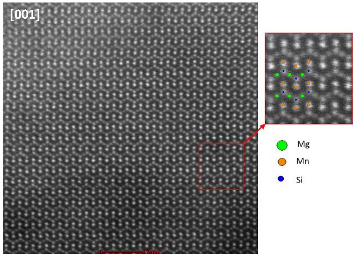
Figure 4-12. High-resolution STEM image of \text{MgMnSiO}_4/\text{C} particle observed along the [001] orthorhombic zone axis. The general Mg, Mn and Si atomic positions are shown in inset, respectively in green, orange and blue.
