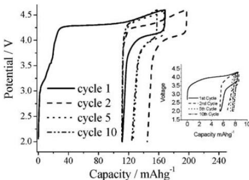
Figure 1-18. Variation of voltage with state of charge (Li content) on cycling the β I -Li 2 CoSiO 4 polymorph carbon coated by the xerogel process at a rate of 10mA.g -1 , from [100]. Inset shows performance of uncoated material.
