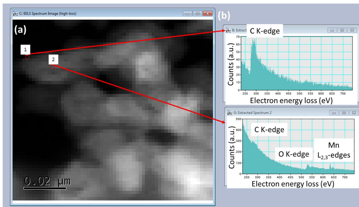
Figure 3-19. Scanning Transmission Electron Microscopy image in High-Angle Annular Dark-Field mode (a) and Electron Energy Loss Spectroscopy spectra in the 200-800eV range (b) of LMS/C_81.
