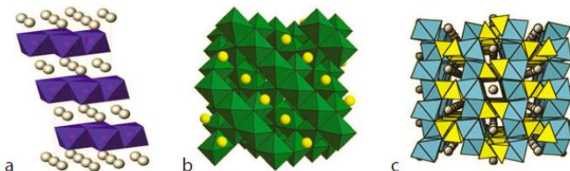
Figure 1-2. Structures of common positive electrode materials: (a) The layered structure of \text{LiCoO}_2 , with the octahedrally coordinated Li ions are represented as spheres and \text{CoO}_6 as octahedra; (b) the cubic structure of \text{LiMn}_2\text{O}_4 spinel, with tetrahedrally coordinated \text{Li}^+ ions represented as spheres, and \text{MnO}_6 as octahedra; and (c) the olivine structure of \text{LiFePO}_4 , looking down the b -axis. Octahedrally coordinated Li ions are represented as spheres, and \text{FeO}_6 and \text{PO}_4 as octahedra and tetrahedra, respectively; adapted from [18].
