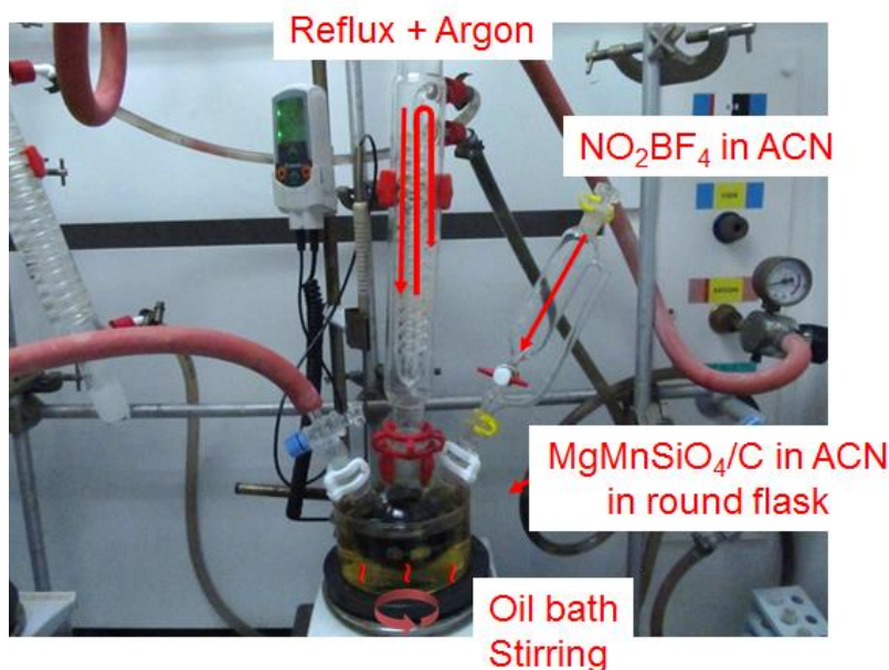
Figure 4-6. Picture of the chemical oxidation set-up including: a round flask containing a dispersion of MgMnSiO 4 /C in acetonitrile heated by an oil bath at 60°C and stirred continuously; a water-cooled condenser which condenses ACN vapors and an isobar dropping funnel containing a solution of NO 2 BF 4 in ACN.
