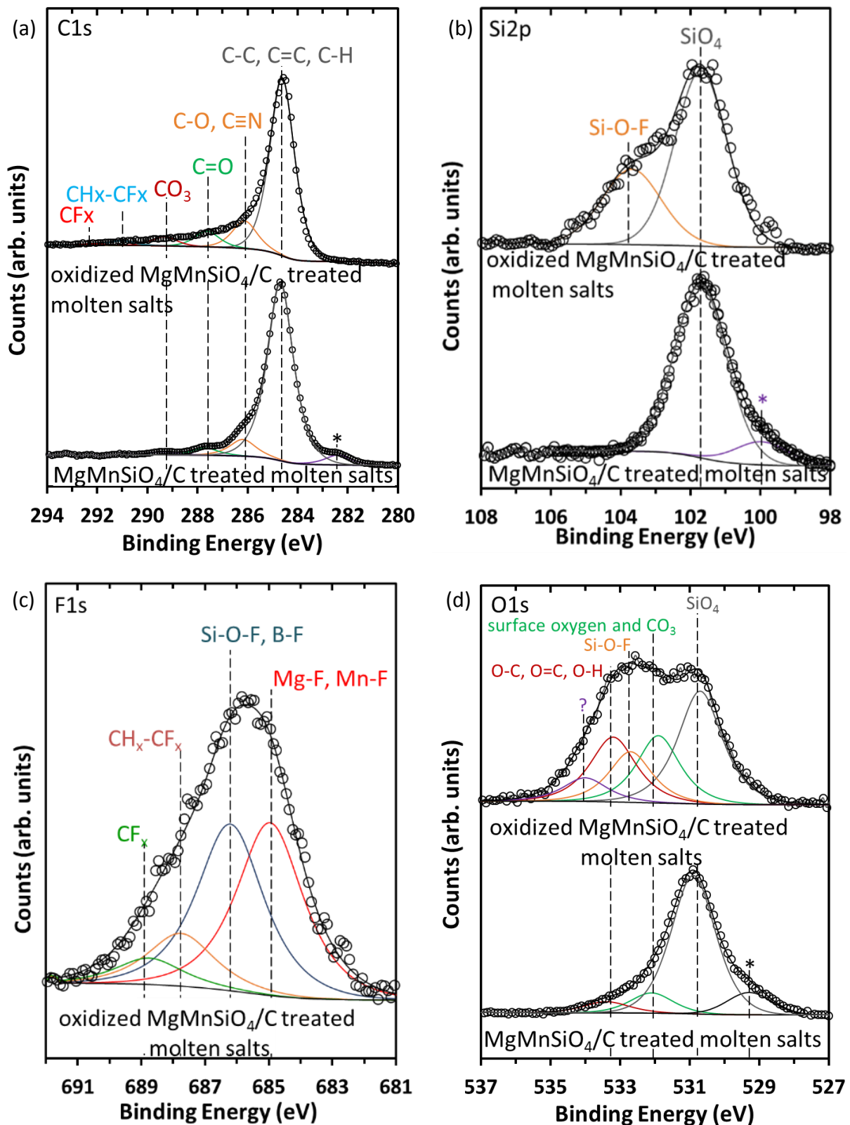
Figure 4-30. XPS C1s (a), Si2p (b), F1s (c) and O1s (d) normalized spectra of MgMnSiO 4 /C treated in molten salts and oxidized MgMnSiO 4 /C treated in molten salts. Calibration with Si2p component of SiO 4 at 101.7eV. The charge effect is represented by a component which is marked by a star "*" on C1s, Si2p and O1s spectra of MgMnSiO 4 /C treated molten salts.
