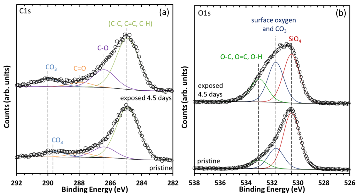
Figure 3-43. XPS C1s (a) and O1s (s) spectra of pristine LMS/C_81 and exposed 4.5 days to air LMS/C_81 materials. Spectra were calibrated with the "SiO 4 " O1s component at 530.5eV.
