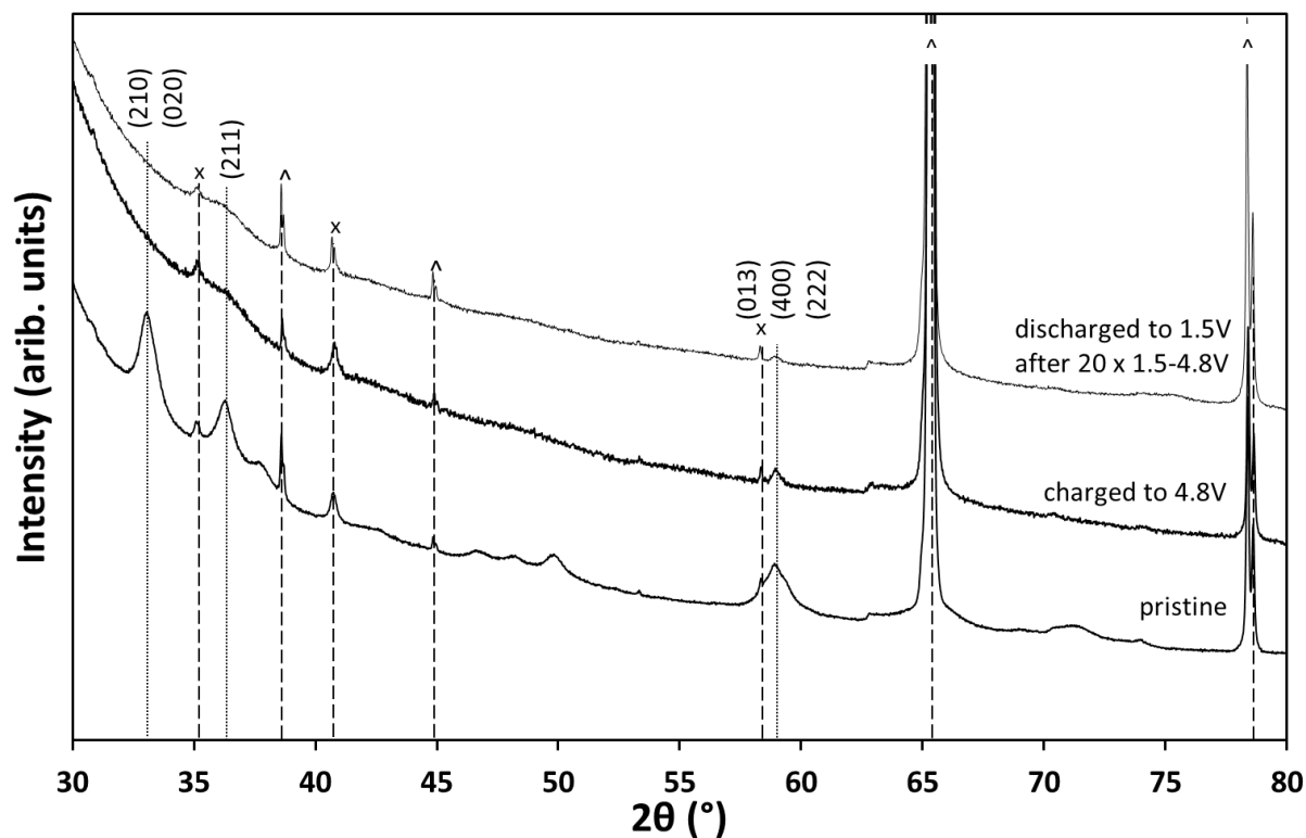
Figure 3-25. Ex-situ XRD patterns of pristine, charged to 4.8V and cycled 20 times between 1.5V and 4.8V and discharged to 1.5V LMS/C_81 electrodes. The following symbols correspond to MnO (X) and Al current collector (^). The most intense reflections of Li 2 MnSiO 4 are represented by their Miller indexes.
