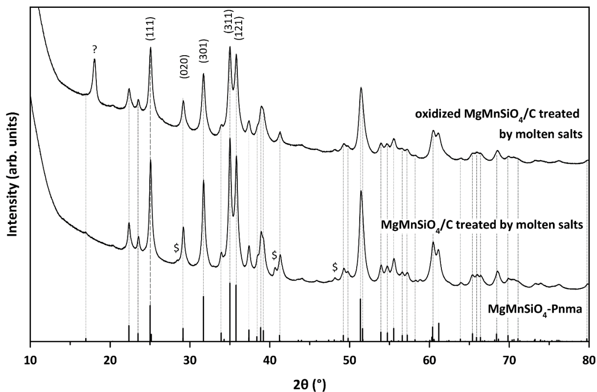
Figure 4-26. Powder X-Ray Diffraction patterns of pristine \text{MgMnSiO}_4/\text{C} treated in molten salts and oxidized \text{MgMnSiO}_4/\text{C} treated in molten salts. The KCl impurity peaks are labelled by a ($) symbol. The additional peak appearing after the chemical oxidation is labelled with a (?) symbol.
