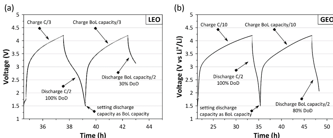
Figure 4-47. Examples of beginning of life capacity determination (1 st galvanostatic cycle) and relevant C/rate and DoD conditions (2 nd galvanostatic cycle for (a) LEO cycling and (b) GEO cycling) based on \text{Li}_2\text{MnSiO}_4/\text{C} cells at 20°C.
