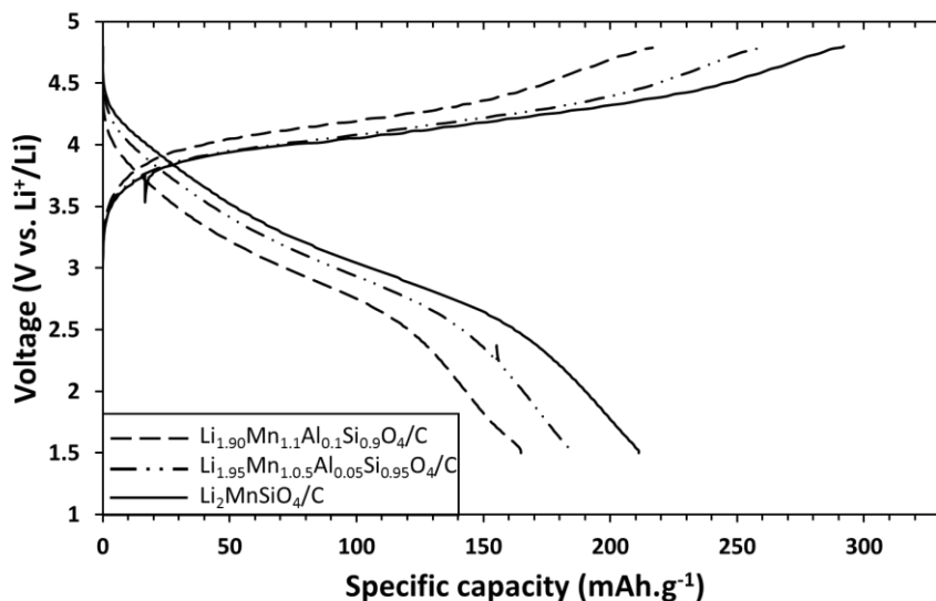
Figure 3-37. First galvanostatic cycle of \text{Li}_{2-x}\text{Mn}_{1+x}\text{Al}_x\text{Si}_{1-x}\text{O}_4/\text{C} ( x=0, 0.05 and 0.1 ) electrodes at C/20 and room temperature between 1.5V and 4.8V. 1C=333 \text{ mA}\cdot\text{g}^{-1} ; 320 \text{ mA}\cdot\text{g}^{-1} and 308 \text{ mA}\cdot\text{g}^{-1} respectively for x=0; 0.05 and 0.10 . \text{Li}_{2-x}\text{Mn}_{1+x}\text{Al}_x\text{Si}_{1-x}\text{O}_4/\text{C} , with x=0 , correspond to the reference material LMS/C_81.
