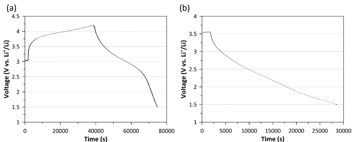
Figure 4-45. (a) First galvanostatic cycle of \text{Li}_2\text{MnSiO}_4/\text{C} positive electrode charged to 4.2V and discharged to 1.5V at C/20 ( 1C=333\text{mA}\cdot\text{g}^{-1} ) and (b) residual discharge of \text{Mg}_{1-x}\text{MnSiO}_4/\text{C} positive electrode to 1.5V at C/10 ( 1C=174\text{mA}\cdot\text{g}^{-1} ), tested at CEA. Discharge capacities are used to define the nominal capacity of the battery at the beginning of testing.
