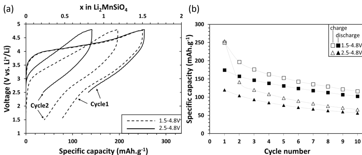
Figure 3-26. First and second galvanostatic cycles (a) and cycling performance (b) of LMS/C 81 electrodes charged up to 4.8V and discharged to 1.5V or 2.5V at C/20 and room temperature.
