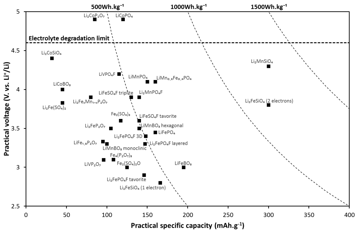
Figure 1-12. Practical voltage (V vs. \text{Li}^+/\text{Li} ) of polyanionic materials as a function of practical specific capacity ( \text{mAh.g}^{-1} ) inspired from [88], the isovalue lines represent the energy density of the positive electrode ( \text{Wh.kg}^{-1} ).
