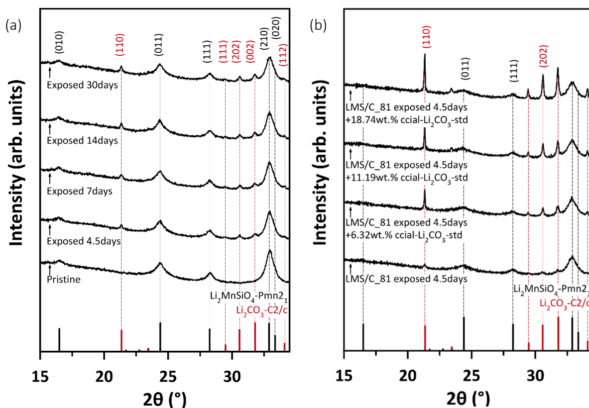
Figure 3-40. X-ray diffraction patterns of (a) pristine and exposed 4.5, 7, 14 and 30 days to air LMS/C_81, (b) LMS/C_81 exposed 4.5 days to air mixed with different weight fractions of commercial Li 2 CO 3 standard, ccial-Li 2 CO 3 -std. All the reflections and Miller indexes of Pmn2 1 -Li 2 MnSiO 4 and C2/c-Li 2 CO 3 are indicated in (a), while only those used for quantitative analysis are displayed in (b).
