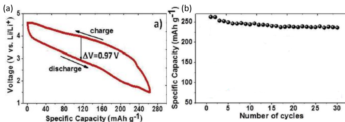
Figure 1-28. Second galvanostatic cycle of a \text{Li}_2\text{MnSiO}_4/\text{C} electrode between 1.5V and 4.8V at C/10 (a) and the associated reversible discharge capacity behavior as function of cycle number (b), adapted from [149].
