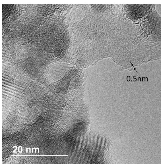
Figure 3-18. Scanning Transmission Electron Microscopy images of LMS/C 81 . Carbon-coating is evidenced by the black arrows and its thickness is indicated.
