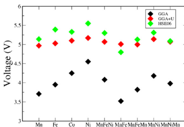
Figure 1-35. Voltage prediction of LiMSiO 4 (M=Mn, Fe, Co, Ni) (V vs. Li + /Li) according to several computation methods [225].
