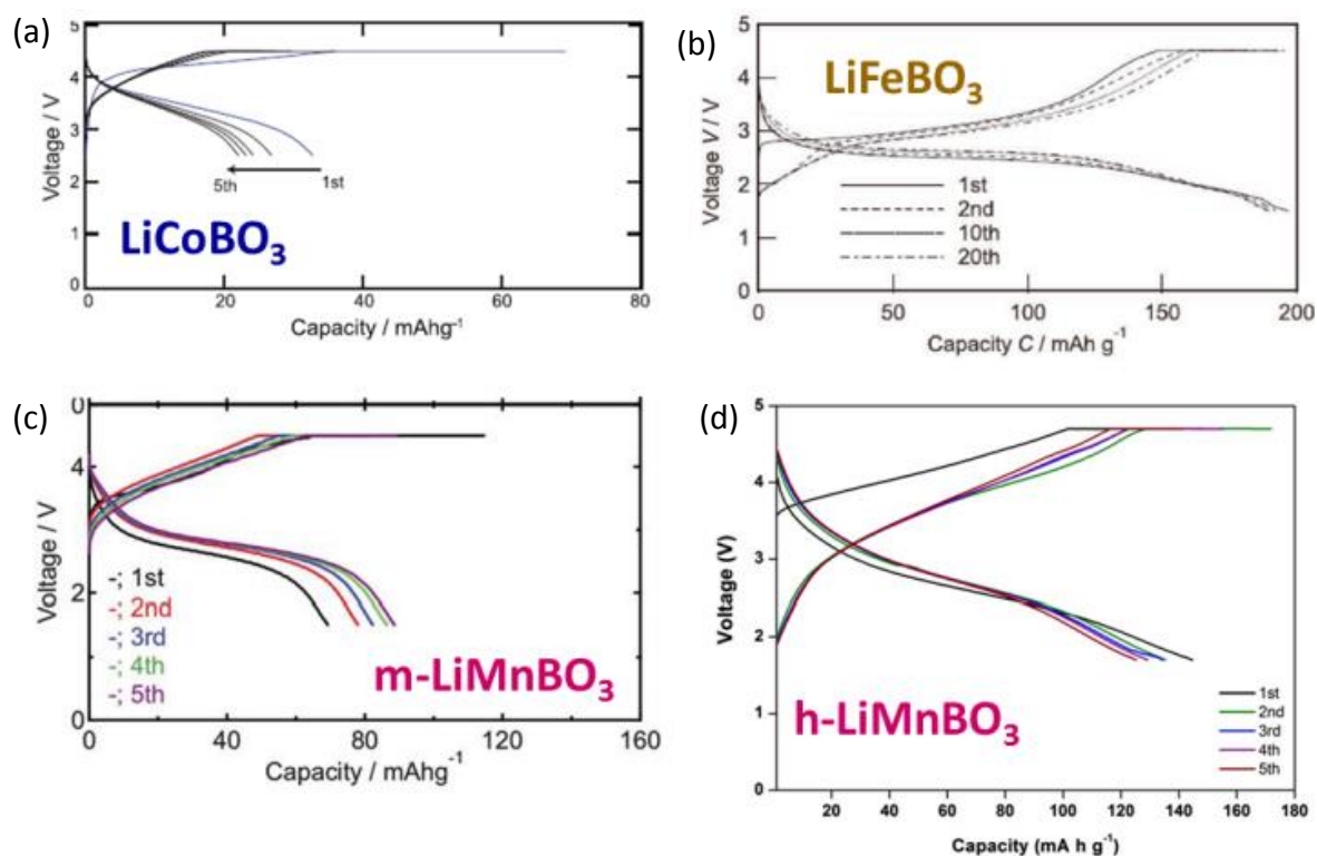
Figure 1-10. Galvanostatic charge-discharge curve of (a) \text{LiCoBO}_3 [75], (b) \text{LiFeBO}_3 [71], (c) monoclinic \text{LiMnBO}_3 [73], (d) hexagonal \text{LiMnBO}_3 [76] cycled at C/20 , adapted from [77].
