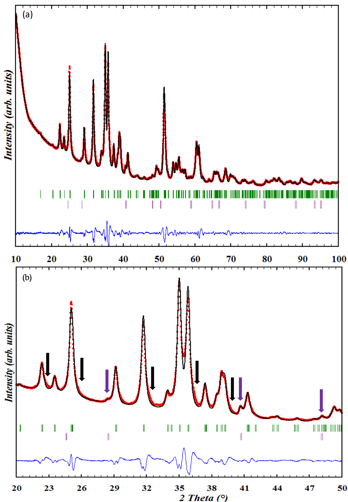
Figure 4-16. (a) Full-pattern matching of \text{MgMnSiO}_4/\text{C} pyrolyzed at 900^\circ\text{C} 24h and treated in \text{LiCl-KCl} molten salts flux at 400^\circ\text{C} for 40h, (b) in the 20-50^\circ 2\theta region. An olivine lattice is used in the \text{Pnma} space group as structural model combined with a cubic \text{KCl} phase, \text{Fm-3m} , as impurity (purple arrows). Red markers: experimental data; black curve: refinement; green tics: Bragg reflections of olivine \text{Pnma} cell; purple tics: Bragg reflections of cubic \text{Fm-3m} cell; blue curve: least squares difference between experimental and refined data; the black arrows represent the tails at bottom of peaks of the \text{MgMnSiO}_4 phase.
