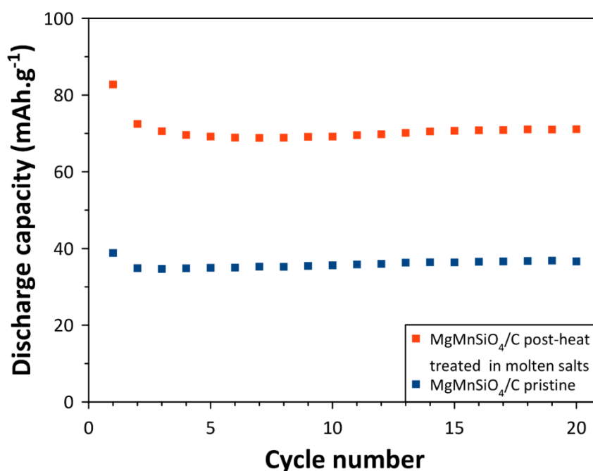
Figure 4-24. Cycling performance of pristine MgMnSiO 4 /C (blue □) and MgMnSiO 4 /C treated in molten salts (orange □) at C/20 ( 1C=313\text{mAh.g}^{-1} ) and room temperature between 1.5-4.8V. The electrolyte and counter-electrode used are respectively based on a LiPF 6 salt and a lithium counter-electrode.
