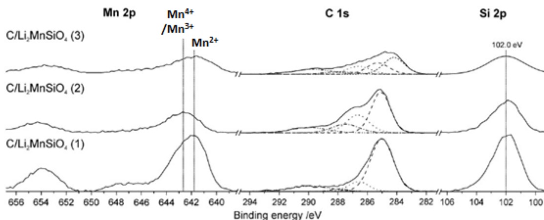
Figure 1-29. Mn2p, C1s and Si2p XPS core spectra of ex-situ \text{Li}_2\text{MnSiO}_4/\text{C} electrodes: pristine (1), after first charge to 4.8V (2), after first discharge to 1.5V (3); from [176].
