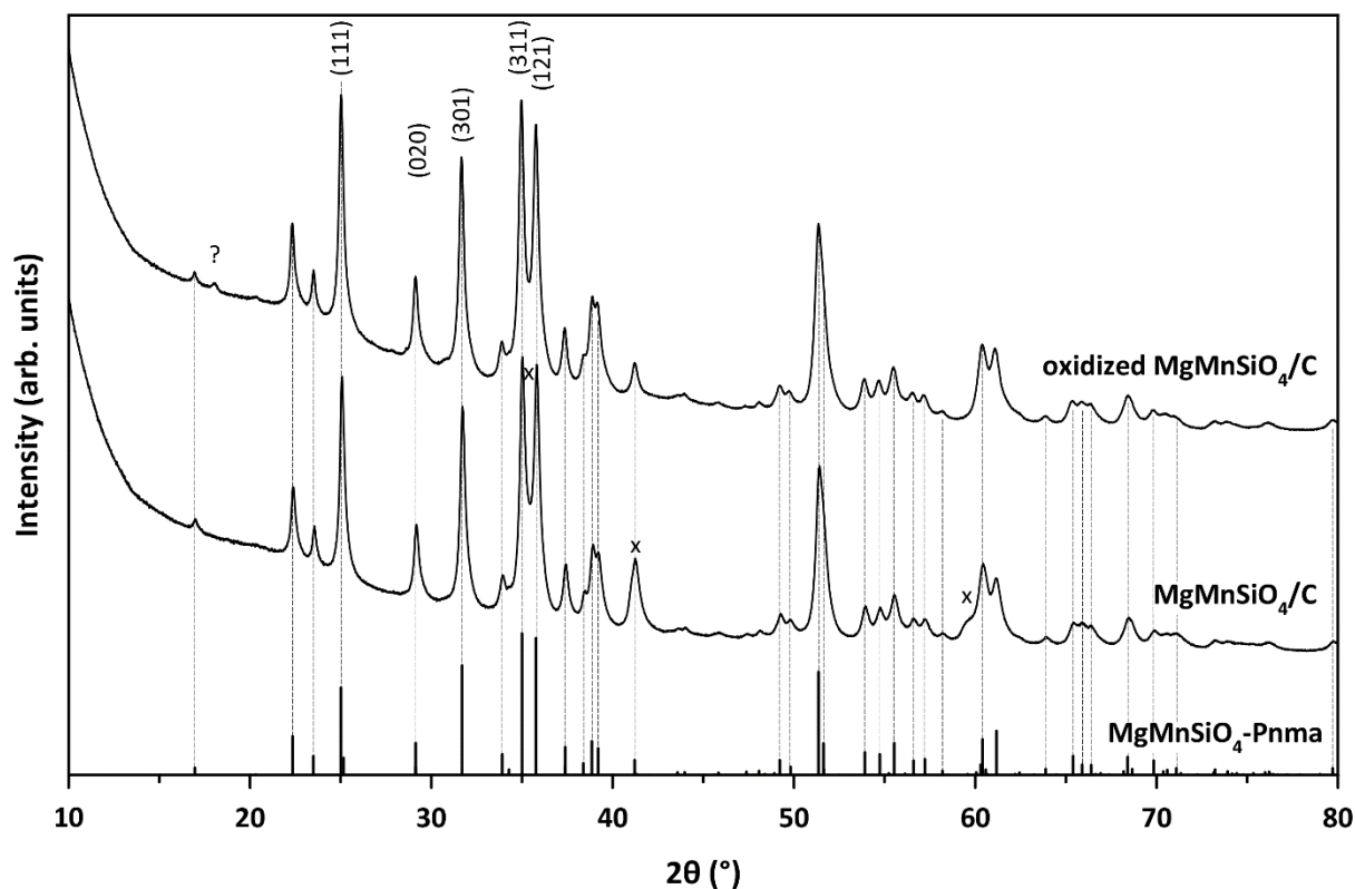
Figure 4-25. Powder X-Ray Diffraction patterns of pristine \text{MgMnSiO}_4/\text{C} and oxidized \text{MgMnSiO}_4/\text{C} . The additional peak appearing after the chemical oxidation is labelled with a (?) symbol.
