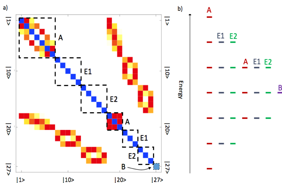
Figure 4.2. a) Pictorial representation of the symmetry-adapted eigenstates and the relaxation matrix of the 27 states of the D 3 subsystem of a 13 CD 3 group after dissolution, appropriate for the extreme narrowing regime ( \omega_L \tau_c \ll 1 ). Positive relaxation matrix elements are represented by yellow and red boxes, and negative elements by blue boxes. Each of the 27 symmetry-adapted states belongs to one of the four symmetry manifolds A, E1, E2 and B. There are no matrix elements that connect different irreducible representations. Therefore, if one considers only quadrupolar relaxation, the populations cannot flow freely between states belonging to different irreducible representations. b) Energy level diagram associated with the D 3 spin system.
