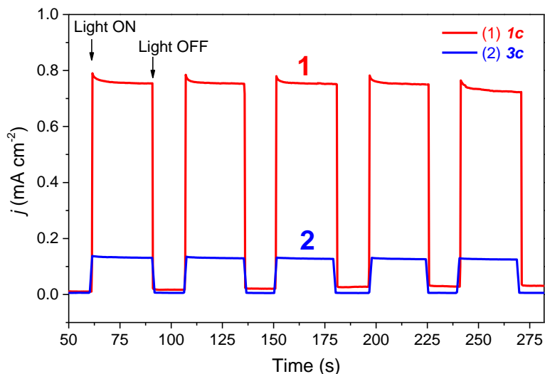
Figure 63 Chronoamperometric curves obtained on 1c ZnO/TiO 2 (curve 1, red), and 3c ZnO/TiO 2 (curve 2, blue) composites in dark and under illumination, at constant potential of 0.8 V vs. Ag/AgCl in aqueous solution of 5 mM Na 2 SO 4 .
