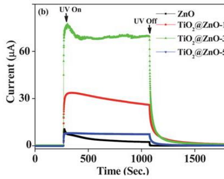
Figure 35 Transient current under dark and illuminated periods for corresponding ZnO and ZnO/TiO 2 composites [275].
