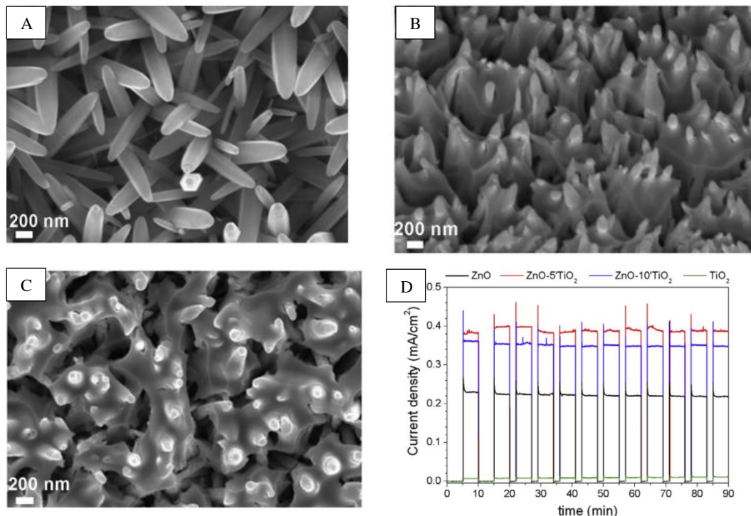
Figure 34 SEM images of bare ZnO (A), and core/shell ZnO/TiO 2 composites with TiO 2 layer prepared after 5 min (B), and 10 min (C) of impregnation. Photocurrent transients of the respective photoanodes under solar light (450 W Xe lamp) irradiation at 0.2 V vs. Ag/AgCl (D) [274].
