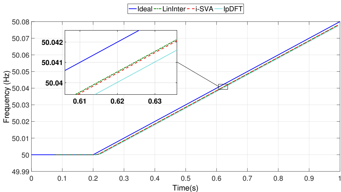
FIGURE III.26 – Frequency computation response of very slow ramp of frequency
