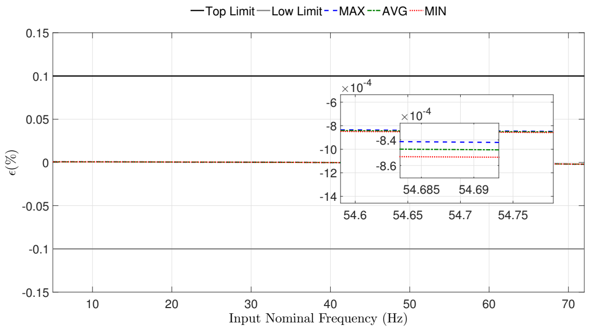
FIGURE II.25 – Ratio error for various frequencies
