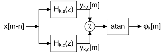
FIGURE I.3 – Microprocessor-based relay phase estimation algorithm
