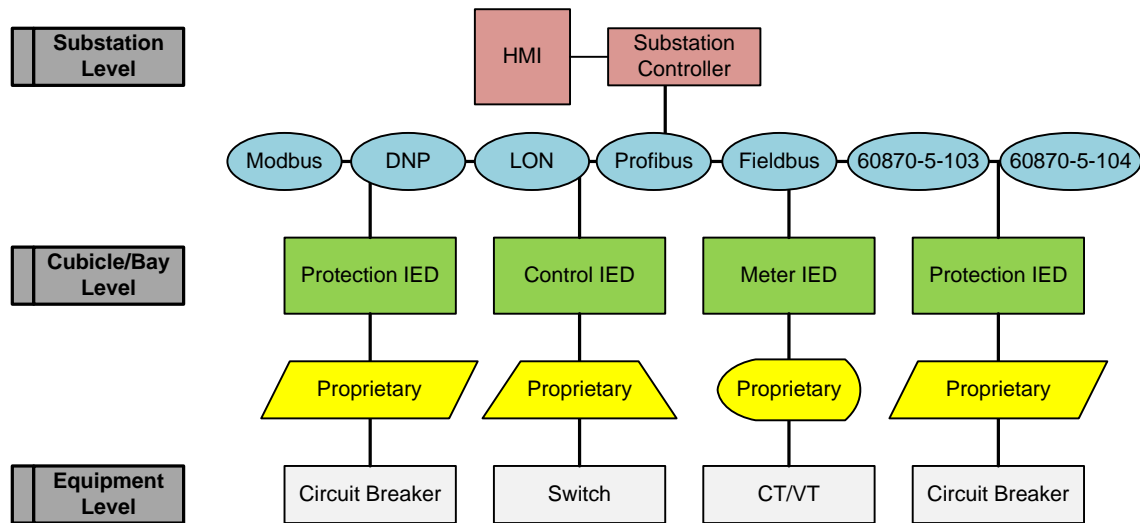
FIGURE II.1 – Traditional SAS architecture with various communication protocols
