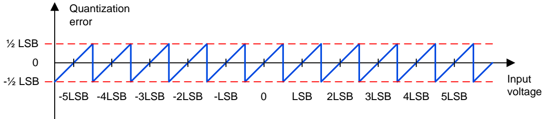
FIGURE I.13 – Evolution of the quantization error
