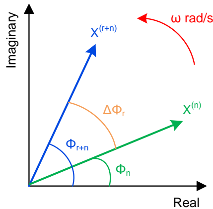
FIGURE I.25 – Rotation of phasors for frequency estimation
