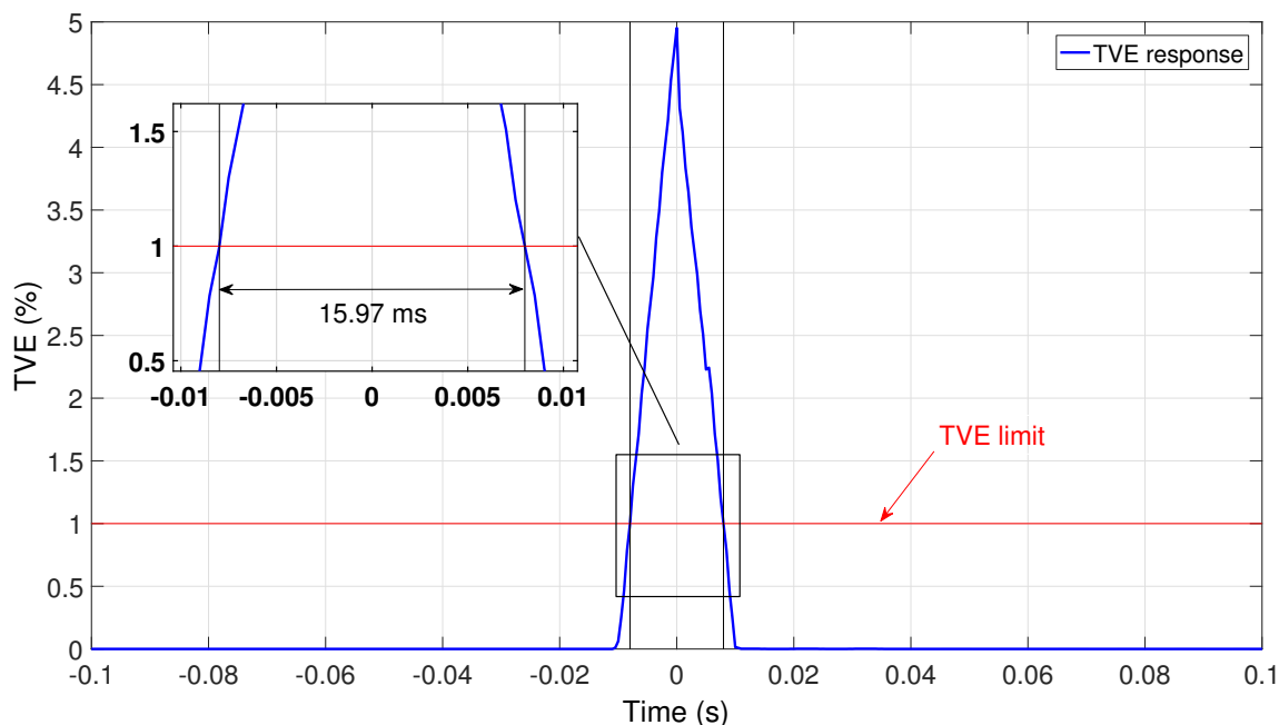
FIGURE IV.15 – Magnitude step change test result - Determination of the synchrophasor algorithm response time
