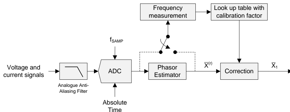
FIGURE I.23 – Simplified frequency error compensation implementation
