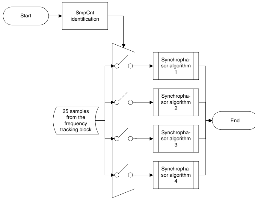
FIGURE IV.7 – Parallelization of synchrophasor estimations
