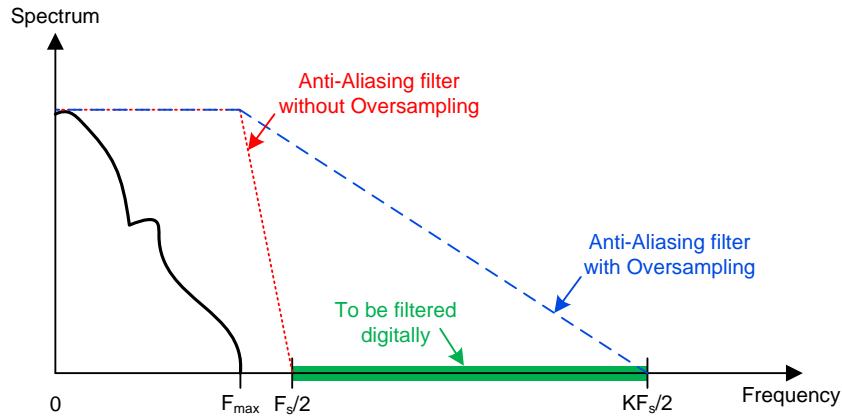
FIGURE I.15 – Anti-aliasing filter characteristics with and without oversampling
