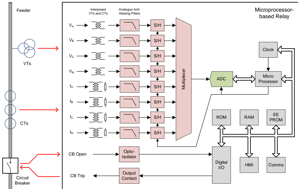
FIGURE I.4 – Microprocessor-based relay involved in the protection system
