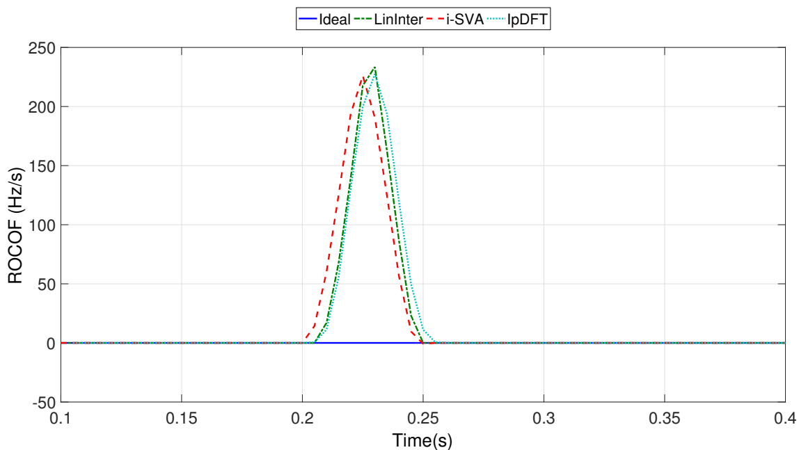
FIGURE III.35 – ROCOF computation response of very slow ramp of frequency
