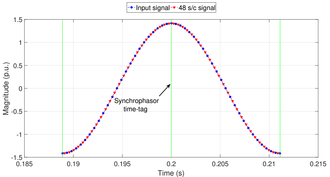
FIGURE IV.5 – Example application of the synchronous linear trigonometric interpolation method
