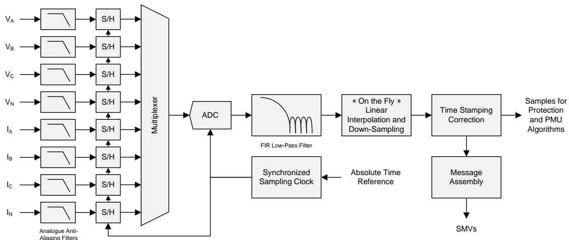
FIGURE II.17 – Simplified signal processing principle for SAMU
