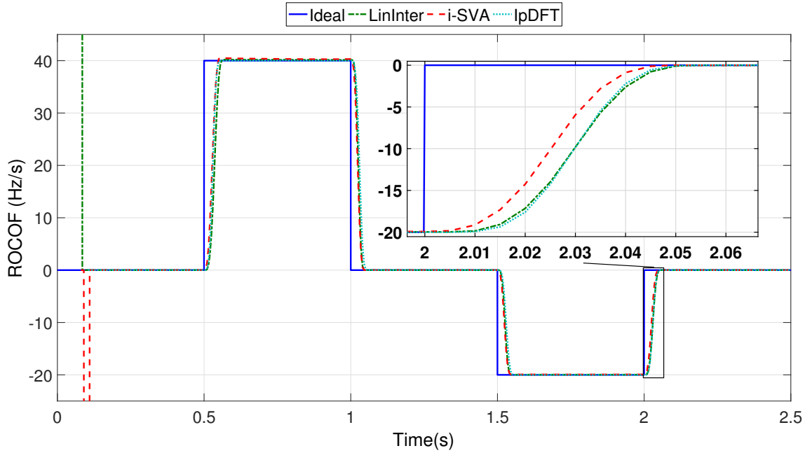
FIGURE III.31 – ROCOF computation response of fast ramps of frequency
