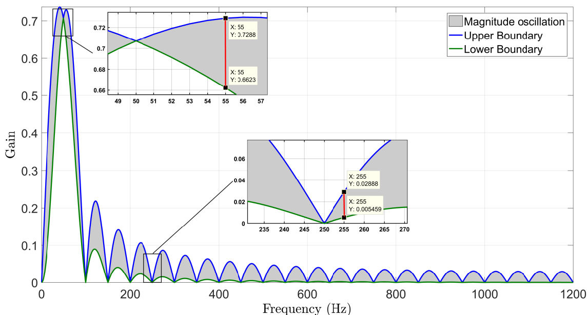
FIGURE I.20 – Example on the effects of off-nominal signal frequency on phasor estimates
