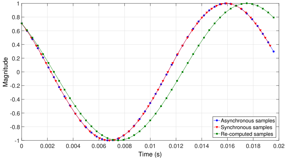
FIGURE III.3 – Basic idea of the resampling algorithm
