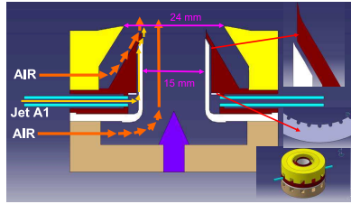
Figure 2.29: Geometrical details of the prefilmer atomizer [103].
