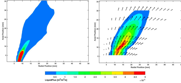
Figure 2.42: Comparison of liquid volume flux for the 16\ \mu\text{m} class obtained with ATF against experimental data (adapted from [103])[90].
