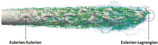
Figure 3.3: Schematical representation of the ELSA coupling proposed in [120]. Adapted from [132].
