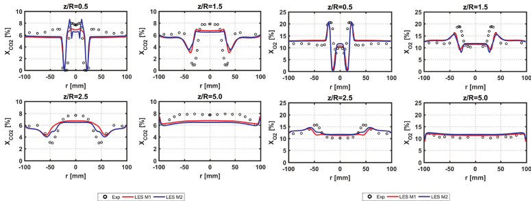
Figure 2.25: Dry (percent) mole fractions of CO_2 (left) and O_2 (right) profiles at several axial positions [90].
