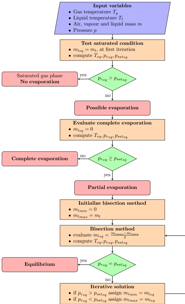
Figure 5.4: Method implemented for computation of equilibrium composition and temperature [185, 187].
