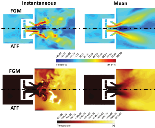
Figure 2.34: Instantaneous (for \tau_{ft}=2 ) and mean axial velocity and temperature distributions obtained with FGM and ATF [90].
