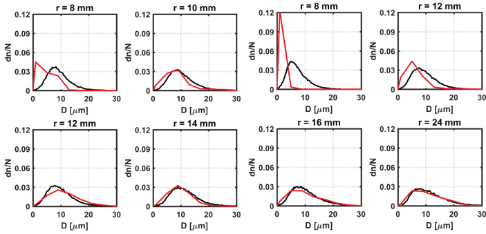
Figure 2.45: PDF spray distributions at z=7 mm (left) and z=15 mm (right) at four radial positions (see Figure 2.35 for details about the four locations) [105]. Experiments in black and numerical results in red.
