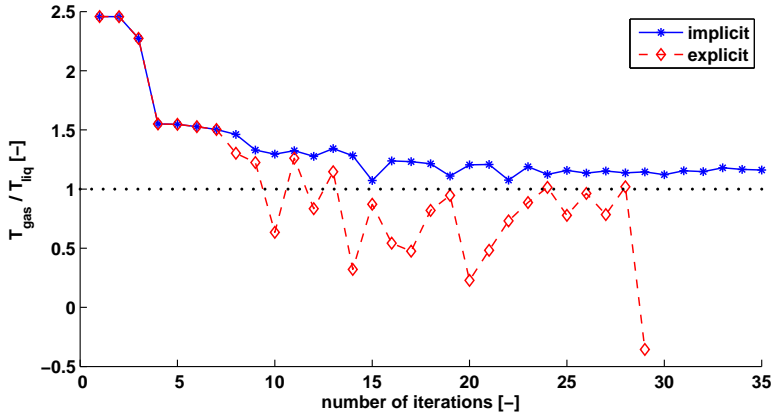
Figure 5.11: Instabilities in gas phase temperature with explicit source term in gas phase temperature [185].
