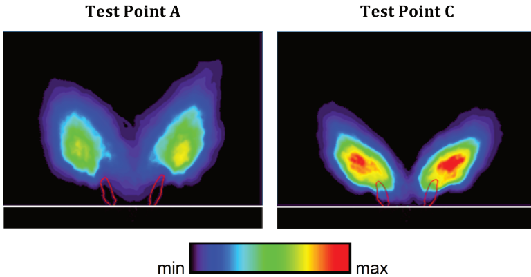
Figure 2.57: Comparison between heat release maps superimposed on fuel distribution for test points A and C [62].
