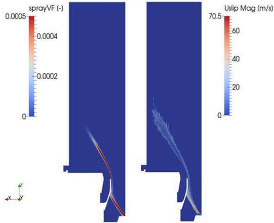
Figure 3.10: Evolution of slip velocity and liquid volume fraction on the symmetry plane [163].
