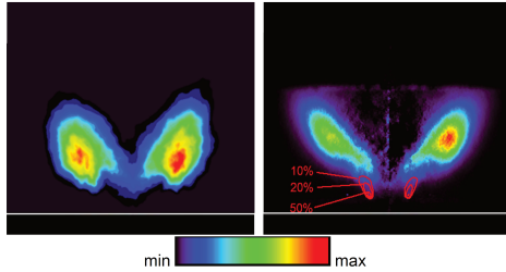
Figure 2.52: Iso-contours of heat release obtained with SAS-FGM (left) against the experimental map (right).
