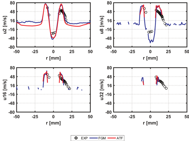
Figure 2.43: Profiles of axial velocities at axial position 7 mm for different size classes obtained with FGM and ATF[90].
