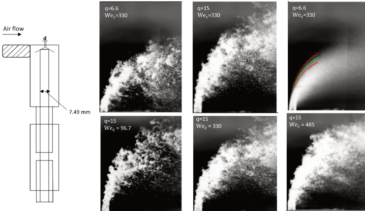
Figure 4.4: Main characteristics of the considered jet in crossflow test case (modified from [172]).
