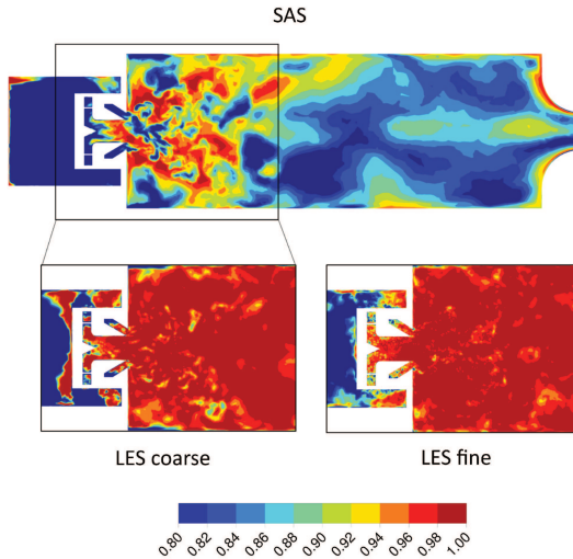
Figure 2.32: Contour of Pope's criterion with SAS and LES with different mesh sizes.
