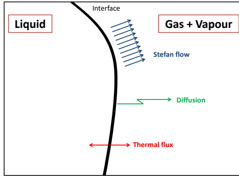
Figure 3.6: Schematic representation of the phenomena involved in liquid evaporation (adapted from [143])
