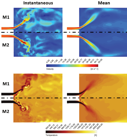
Figure 2.22: Instantaneous (for \tau_{ft}=3.5 for M1 \tau_{ft}=2.5 for M2) and mean temperature and velocity distributions for Sheen Burner for M1 and M2 [90].
