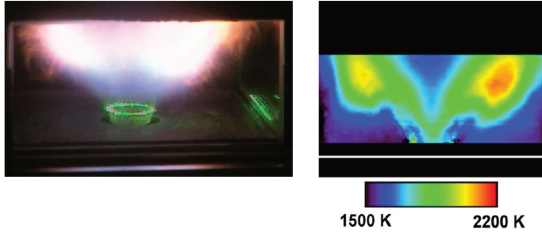
Figure 2.28: Flame visualization and temperature map from OH-PLIF for Test Point A. The white line indicates swirler exit plane [103].
