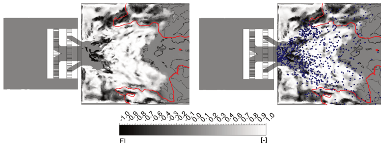
Figure 2.37: Flame Index (FI) distribution obtained with LES-FGM model on the fine mesh. See text for explanations.
