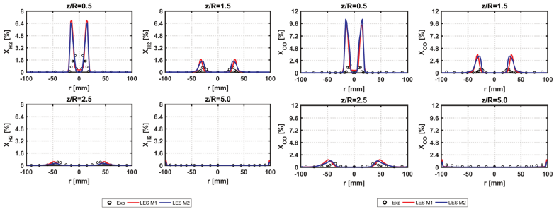
Figure 2.26: Dry (percent) mole fractions of H_2 (left) and CO (right) profiles at several axial positions [90].
