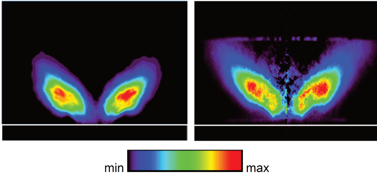
Figure 2.56: Iso-contours of heat release obtained with SAS-FGM (left) against the experimental map (right)[62].
