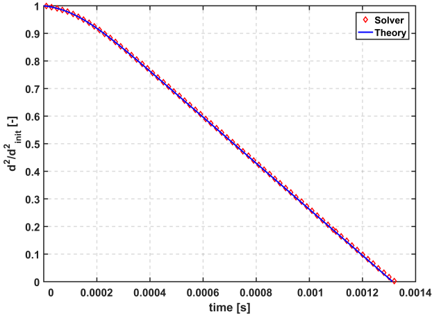
Figure 5.6: Analytical validation of the code for a single evaporating droplet [185].
