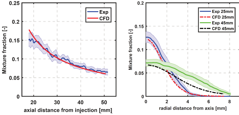
Figure 5.16: Mixture fraction distributions for Test point 2 [185, 187].
