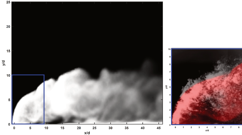
Figure 4.10: Liquid distribution obtained from ELSA calculations compared with experiments.
