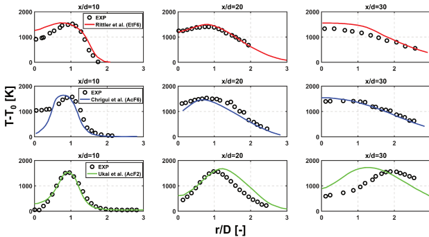
Figure 2.3: Comparison of numerical results obtained on the Sydney spray burner taken from Rittler et al. [78] for EtF6 (top), from Chrigui et al. [37] for AcF6 (middle) and from Ukai et al. [77] for AcF2 (bottom).
