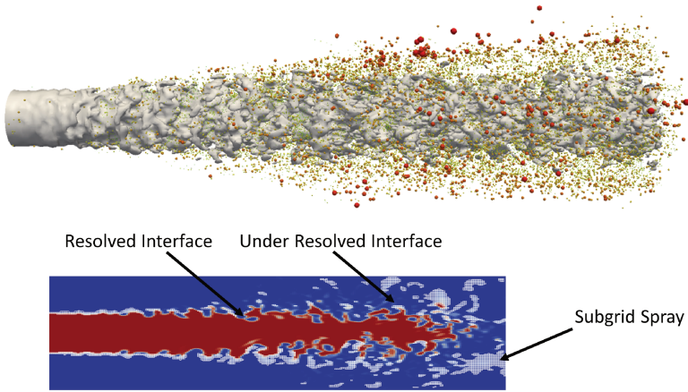
Figure 3.9: Evolution of the complete atomization process for a diesel jet from injection up to the dispersed spray. Adapted from [120].
