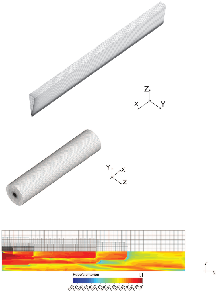
Figure 2.5: Mesh adopted in RANS (top) and LES (bottom) simulations (taken from [80]). Pope's criterion for LES is also shown on the bottom figure.
