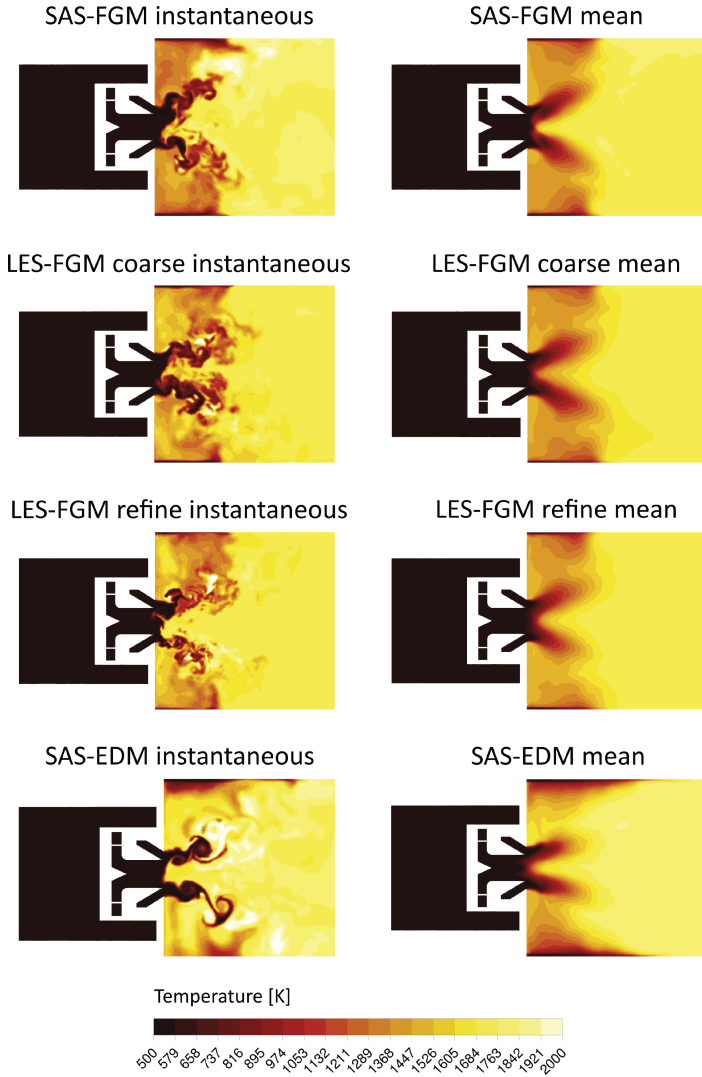
Figure 2.33: Temperature contours obtained with FGM and EDM combustion models with several resolutions of the turbulent field and mesh sizes [104].
