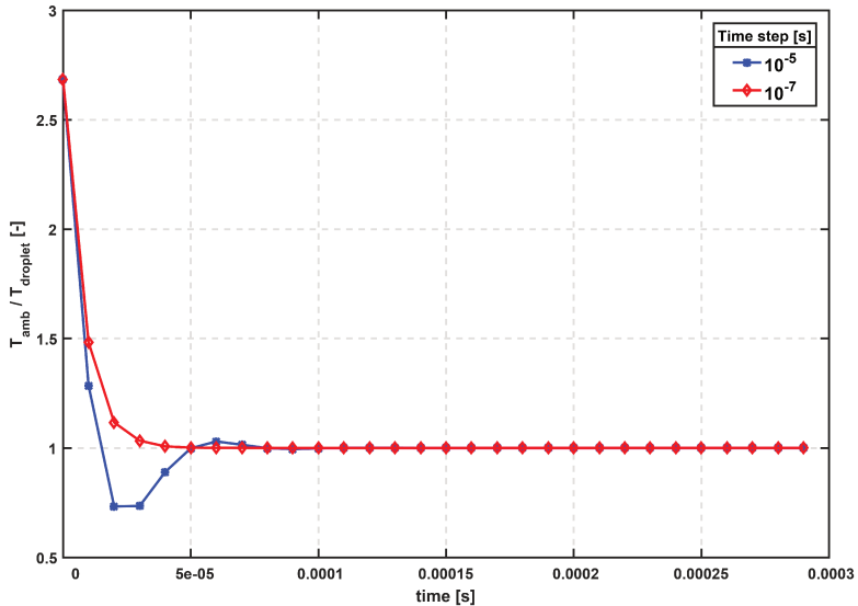
Figure 5.3: Ratio of ambient and droplet temperature with the respect to time for different time step in lagrangian simulation [185, 187].
