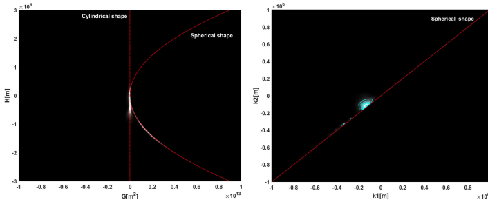
Figure 6.15: Joint PDF of the surface curvatures for \alpha_1 = 1\% : on the left the joint PDF( H, G ) and on the right the PDF( k_1, k_2 ).
