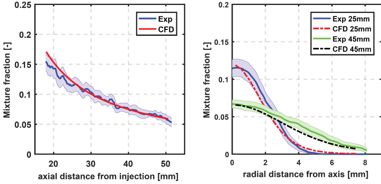
Figure 5.18: Mixture fraction distributions for Test point 3 [185].
