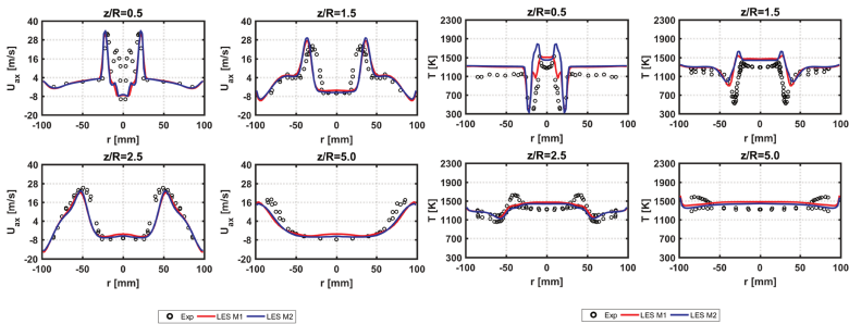
Figure 2.23: Axial velocity (left) and temperature (right) profiles at several axial positions [90].
