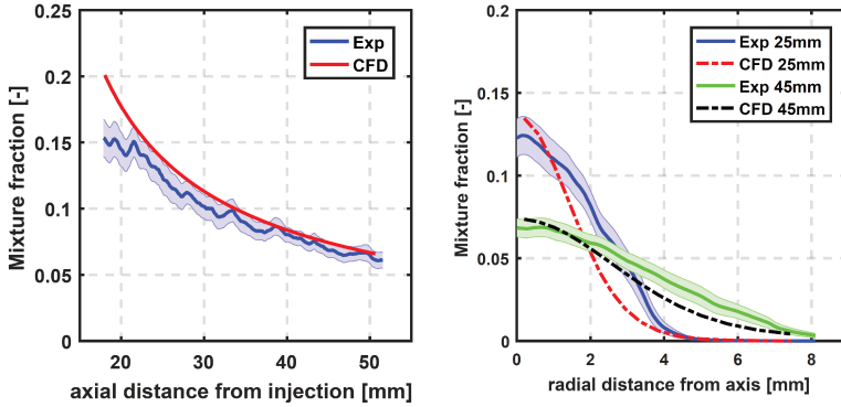
Figure 5.13: Mixture fraction distributions for Test point 1 [185, 187].
