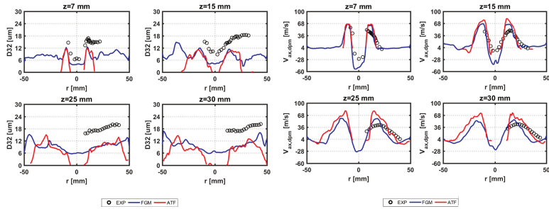
Figure 2.41: Comparison of SMD (left) and axial velocity (right) obtained with FGM and ATF against experimental data [90].
