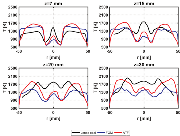
Figure 2.39: Temperature profiles obtained with FGM and ATF at several axial distances [90].
