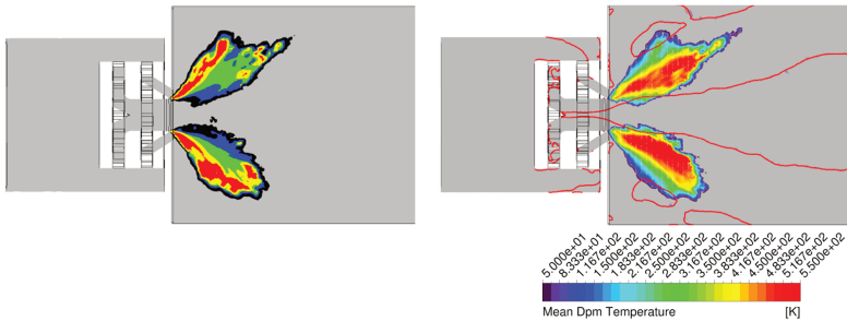
Figure 2.48: Time averaged droplet diameter (left) and axial velocity (right) contour plots. See text for explanations about iso-lines.
