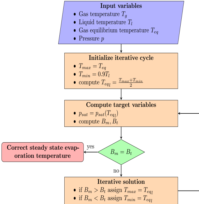
Figure 5.5: Method implemented for computation of equilibrium temperature of liquid in case of complete evaporation [185].
