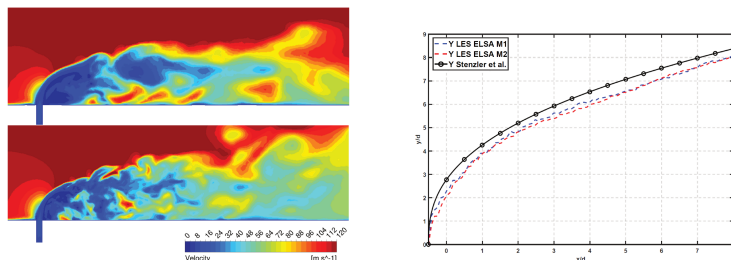
Figure 4.9: Velocity field obtained in LES framework with two different grid sizings (left) and liquid penetration using a first order closure (right).
