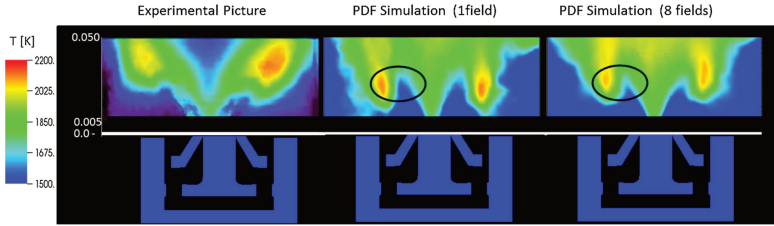
Figure 2.30: Comparison between the experimental temperature map (left) and the contour-plot obtained with one (middle) and eight (right) Eulerian fields obtained in [94]. Adapted from [94].
