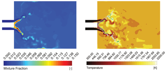
Figure 2.24: Instantaneous mixture fraction contour plot (left) and temperature distribution (right). The white line represents the iso-line at \alpha_1=1e-05 , the green line the stoichiometric Z and the blue one Z=0.012 .
