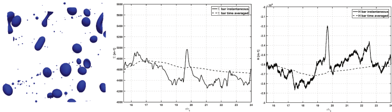
Figure 6.11: Visualization of liquid-gas interface for liquid volume fraction of 1%, together with time evolution of \bar{S} and \bar{H} .
