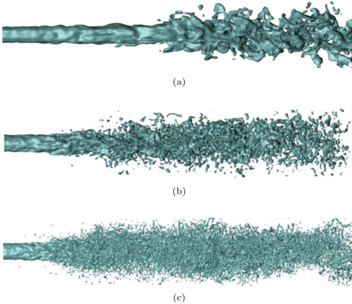
Figure 3.2: Diesel jet simulation for several mesh sizings: 32^2 \times 256 in Figure 3.2a, 64^2 \times 512 in Figure 3.2b, 128^2 \times 1024 in Figure 3.2c. Adapted from [130]
