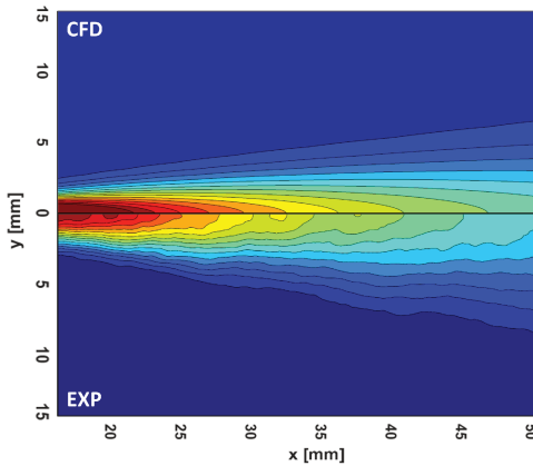
Figure 5.14: Mixture fraction contour comparison for Test point 1 [185, 187].
