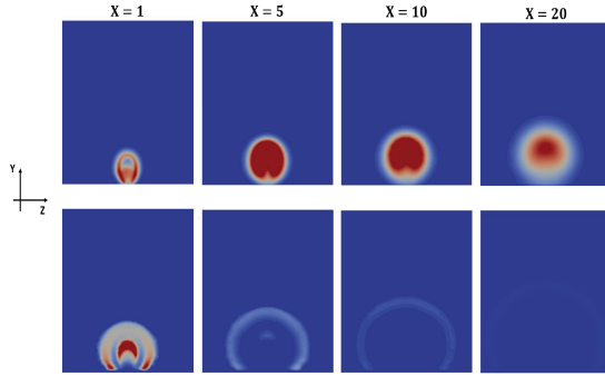
Figure 4.6: Liquid/gas interface density (top) and slip velocity (bottom) distributions at different axial distances with QME [163].
