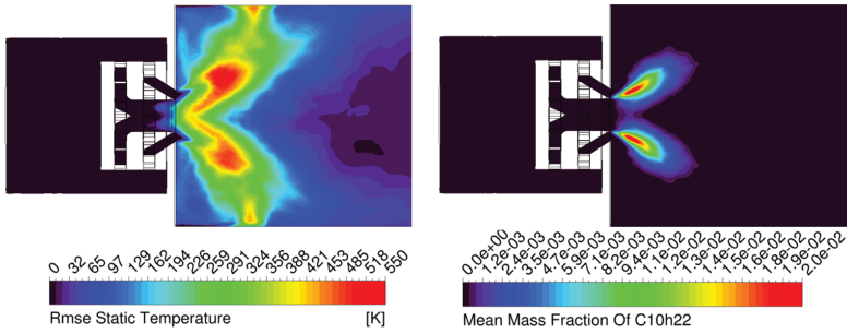
Figure 2.50: Contour plots of temperature fluctuations (left) and decane vapour mass fraction (right).
