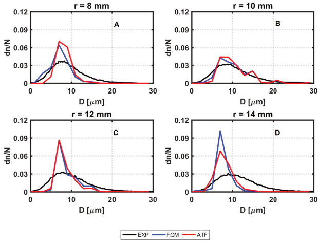
Figure 2.40: PDF spray distributions obtained with FGM and ATF at z=7 mm at four radial positions (see Figure 2.35 for details about the four locations)[90].
