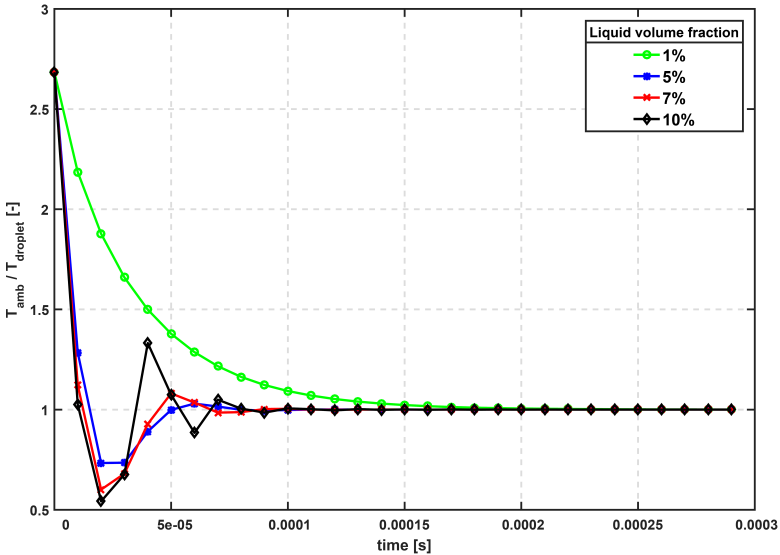
Figure 5.2: Ratio of ambient over liquid temperature with the respect to time for several liquid volume fraction values [185, 187].
