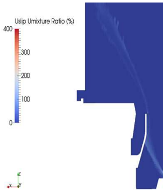
Figure 3.11: Zoom of the distribution of the ratio between the slip and the mixture velocity in the pilot region [163].
