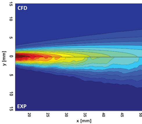
Figure 5.17: Mixture fraction contour comparison for Test point 2 [185, 187].
