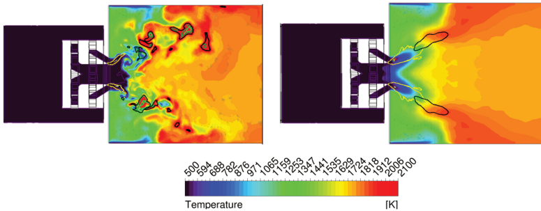
Figure 2.51: Instantaneous and mean contour plots of temperature. See text for explanations about iso-lines.
