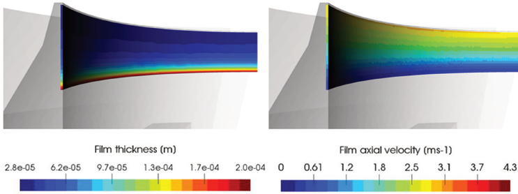
Figure 2.44: Evolution of film thickness together with its axial velocity [105].
