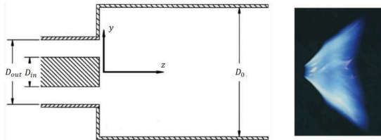
Figure 2.18: Sketch of the geometry experimentally studied and of the spray flame under investigation (adapted from [88]).
