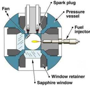
Figure 5.7: Schematic representation of ECN combustion chamber [192].
