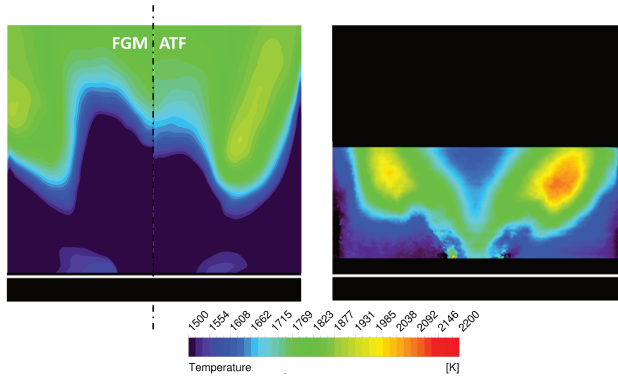
Figure 2.36: Temperature distributions obtained with FGM and ATF against the experimental map (modified from [103]). The white line indicates the burner exit plane [90].
