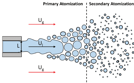
Figure 3.1: Sketch of various atomization processes in liquid jet breakup. Adapted from [120].
