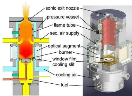
Figure 2.27: Schematic and 3D views of the Single Sector Combustor [103].
