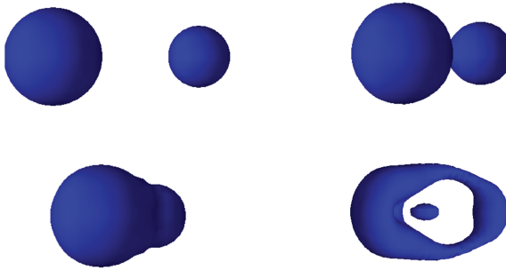
Figure 6.8: Surface evolution for droplet collision test case at t_a (top left), t_b (top right), t_c (bottom left) and t_d (bottom right).
