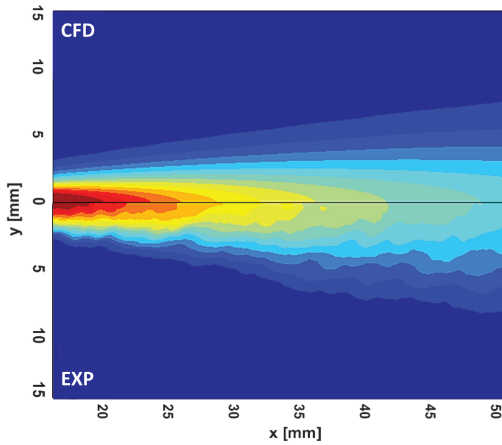
Figure 5.19: Mixture fraction contour comparison for Test point 3 [185].
