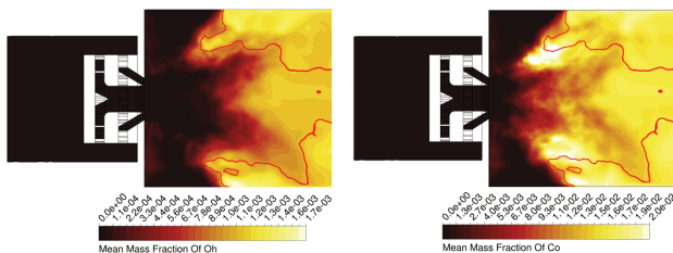
Figure 2.38: Time averaged contour plots of CO and OH mass fraction obtained with LES-FGM.
