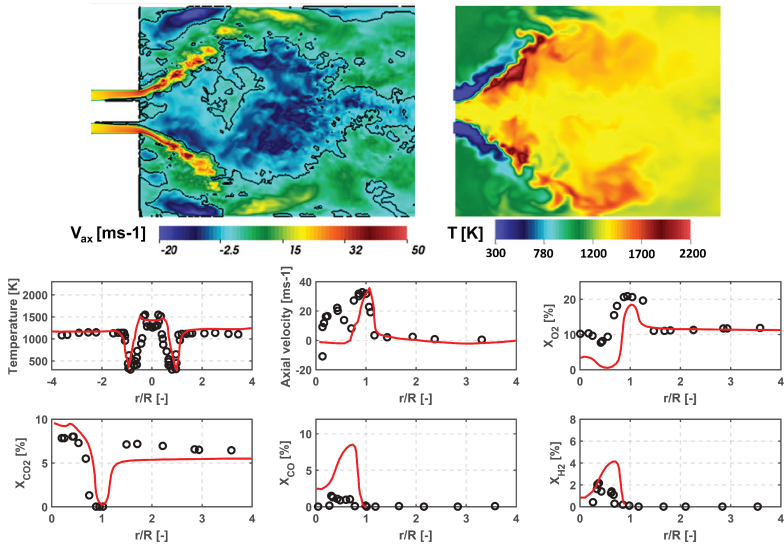
Figure 2.19: Numerical results obtained by Jones et al. [91] in terms of flow-field and temperature contour plots (top) and radial profiles at z/R = 0.5 (bottom). Modified from Jones et al. [91].
