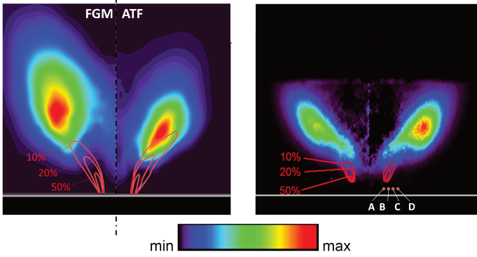
Figure 2.35: Iso-contours of heat release rates obtained with FGM and ATF against the experimental map (modified from [103]). Red iso-lines represent different levels of fuel distribution. The white line indicates the burner exit plane. The red points A, B, C, and D on the experimental map highlight the radial positions where spray PDF is evaluated (see Fig. 2.40)[90].
