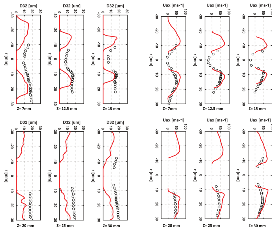
Figure 2.46: Comparison of SMD (left) and axial velocity (right) profiles obtained after the film sensitivity against experimental data [105].
