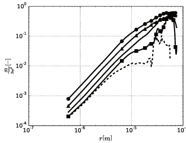
Figure B.6: Second order structure function S_2 in liquid part. The curve with \bullet represents S_2 for \varphi \in [0; 5]dx ; the curve with \blacktriangle represents S_2 for \varphi \in [5; 10]dx ; the solid curve represents S_2 for \varphi \in [10; 15]dx ; the curve with \blacksquare represents S_2 for \varphi \in [15; 20]dx ; the dashed curve represents S_2 for \varphi \in [20; 25]dx
