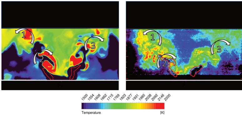
Figure 2.55: Comparison of instantaneous temperature contour obtained between SAS-FGM (left) and experiments (right) for Test Point C [62].
