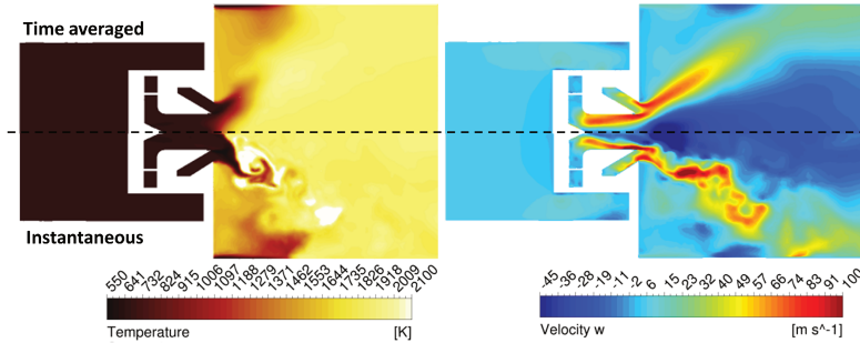
Figure 2.54: Time-averaged and instantaneous temperature and velocity contour plots obtained with SAS-FGM for Test Point C.
