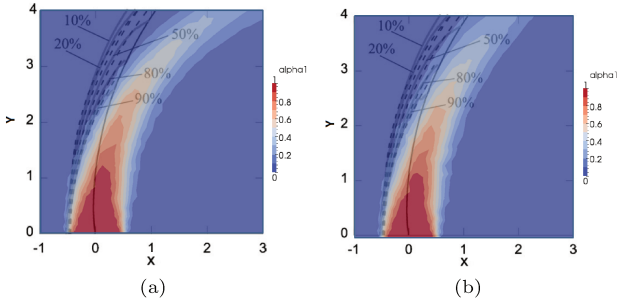
Figure 4.7: Comparison of the probability isolines in [131] for R=100 with the liquid volume fraction field obtained with first order (a) and second order (b) closure with R=1000 [163].
