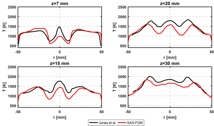
Figure 2.53: Temperature profiles obtained with SAS-FGM compared with profiles of Jones et al. [94].
