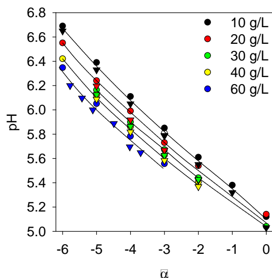
Figure 2. Dependency of the pH on the charge density of WPI aggregates with R_h = 35 nm (triangles) and R_h = 77 nm (circles) at different aggregate concentrations indicated in the figure. The lines are guides to the eye.
