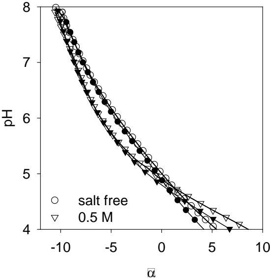
Figure 2. Comparison of the pH as a function of the net charge density between native WPI (filled symbols) and \beta -lg (open symbols) without NaCl (circles) and with 0.5 M NaCl (triangles). The protein concentration was 10 g/L.
