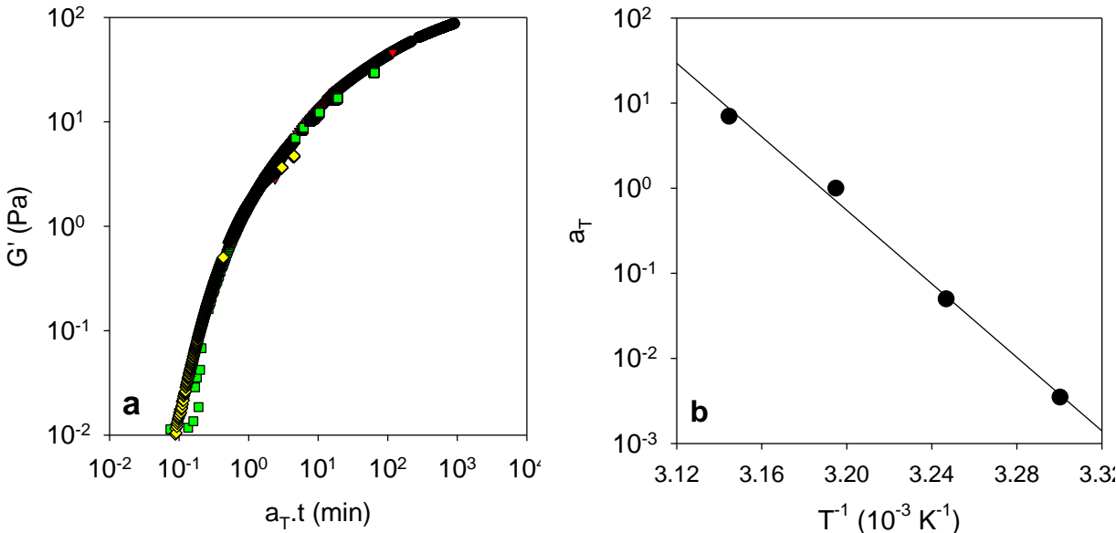
Figure 11. a) Master curve of the results shown in Fig. 9c for a mixture with C_{MC} = 60 \text{ g/L} and C_{WPI} = 10 \text{ g/L} at pH 6.0 obtained by time-temperature superposition. b). Arrhenius representation of the shift factors.
