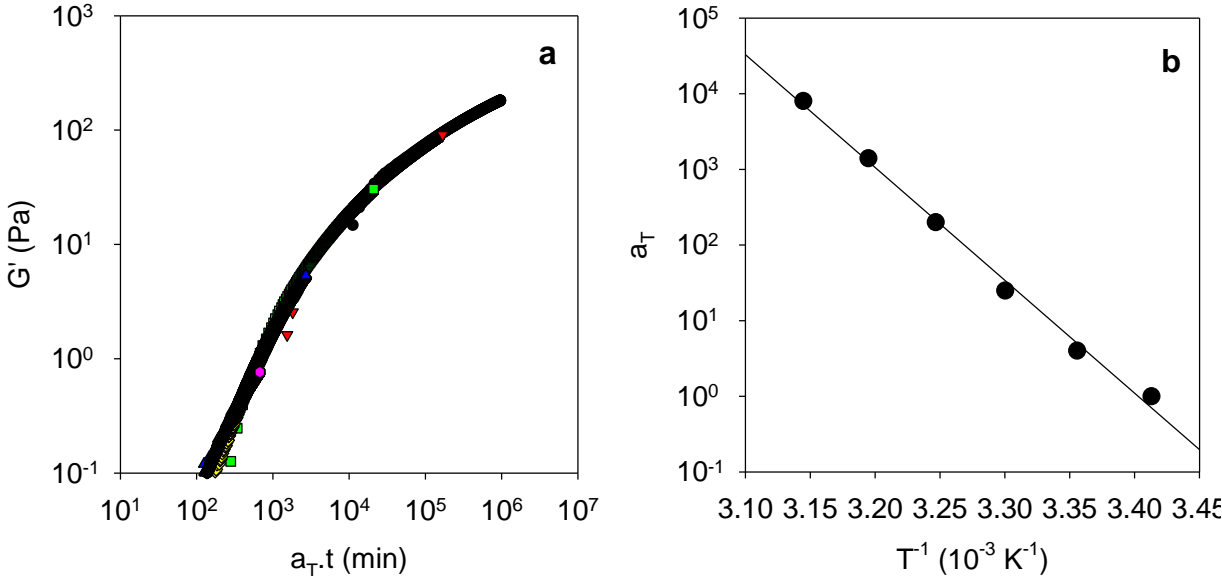
Figure 10. a). Master curve of the data shown in Fig. 9d for a mixture with C_{MC} = 60 \text{ g/L} and C_{WPI} = 15 \text{ g/L} at pH 6.0 obtained by time-temperature superposition. b). Arrhenius representation of the shift factors used to obtain the master curve shown in Fig. 10a.
