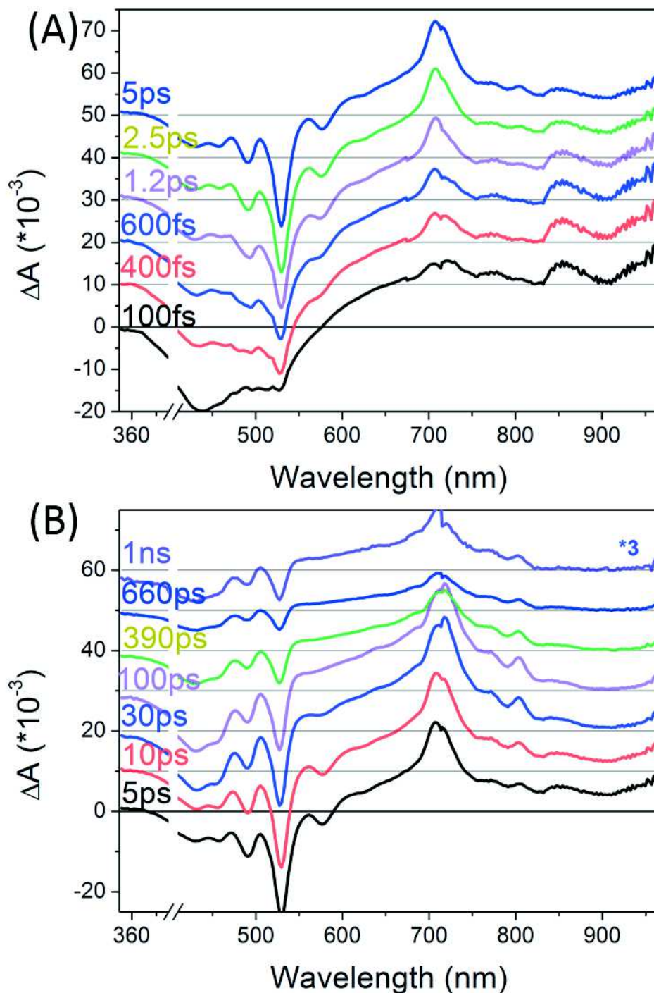
Figure IV.5 Selection of differential absorption spectra of D_1\delta A in chloroform (A) within the first 5ps, showing the formation of D excited state and energy transfer from D excited state to A excited state (B) until 1ns, illustrating the formation of CT state from A excited state and CT state recombination. The differential absorption spectrum at 1ns is magnified by 3 to show the spectral feature.
