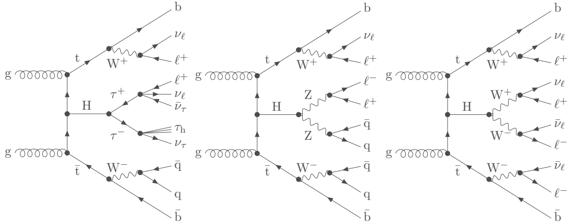
Figure 5.10: Examples of leading Feynman diagrams for t\bar{t}H production in the multilepton final state.
