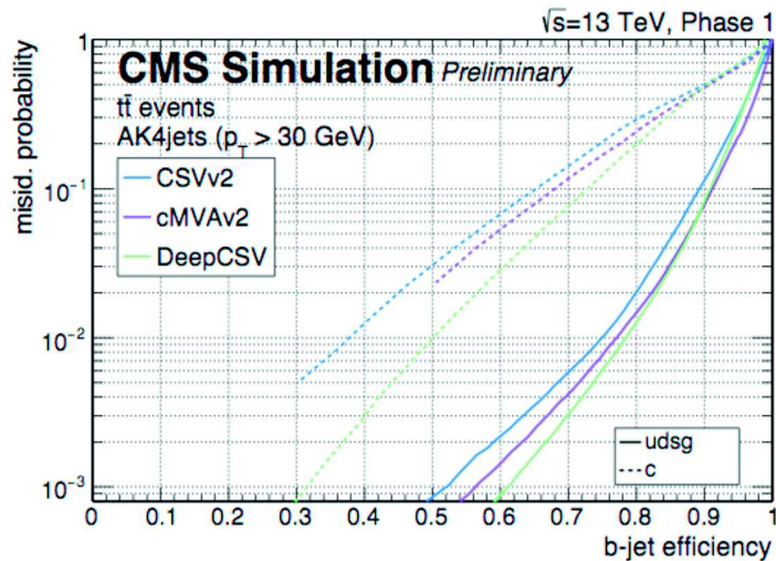
Figure 4.7: Performances of the CSV, cMVA and Deep CSV taggers.
