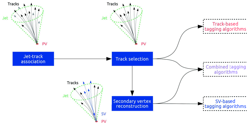
Figure 4.2: b-tagging strategy.
