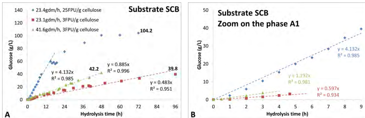
Figure 3-50. Glucose production as a function of time for different feeding rates and enzyme/substrate loadings with SCB. (A: whole experiment, B: focus on A1 step).
