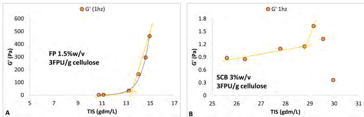
Figure 3-22. Correlation between ex-situ rheometry and biochemistry for FP and SCB at 3 FPU/g cellulose.
